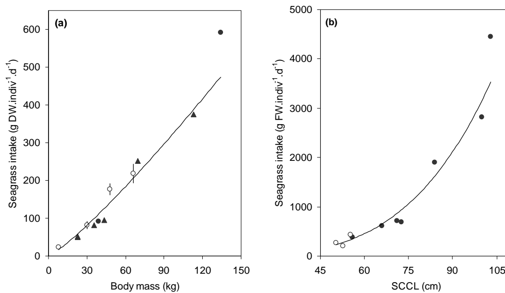
Fig. 6 Relationship between the daily food intake (DFI) and the body size in green turtles Chelonia mydas in (sub-)tropical regions. (a) Relationship between the daily food intake (DFI) and the body mass: DFI \text{ (g DW indiv}^{-1} \text{ d}^{-1}) = 0.51 \times \text{body mass}^{1.43} \text{ (kg)} . Open circles correspond to 12 green turtles (3 individuals for four body mass classes over 12 months) feeding on a monospecific Thalassia testudinum seagrass bed (Great Inagua, Bahamas; Bjorndal 1980). Error bars are ( \pm se). Filled symbols correspond to values calculated in this study for 5 immature and 3 mature green turtles feeding on the multispecific seagrass bed of N’Gouja (see Table 3 ). Full triangles represent individuals for which the body mass was not measured using an electronic spring scale ( \pm 0.1 kg, as full circles), but was deduced from the standard curved carapace length (SCCL) using the model calculated in Fig. 3 . (b) Relationship between the daily food intake (DFI) and the curved carapace length SCCL: DFI \text{ (g FW indiv}^{-1} \text{ d}^{-1}) = 3\,474.7 \times \text{SCCL}^{4.27} \text{ (m)} . Open circles correspond to 3 immature green turtles (captured one time in spring or summer) feeding on different seagrass and algal species (Moreton Bay, South-eastern Queensland, Australia; Brand et al. 1999). Filled circles correspond to values calculated in this study for 5 immature and 3 mature green turtles feeding on the multispecific seagrass bed of N’Gouja (see Table 3 ).
