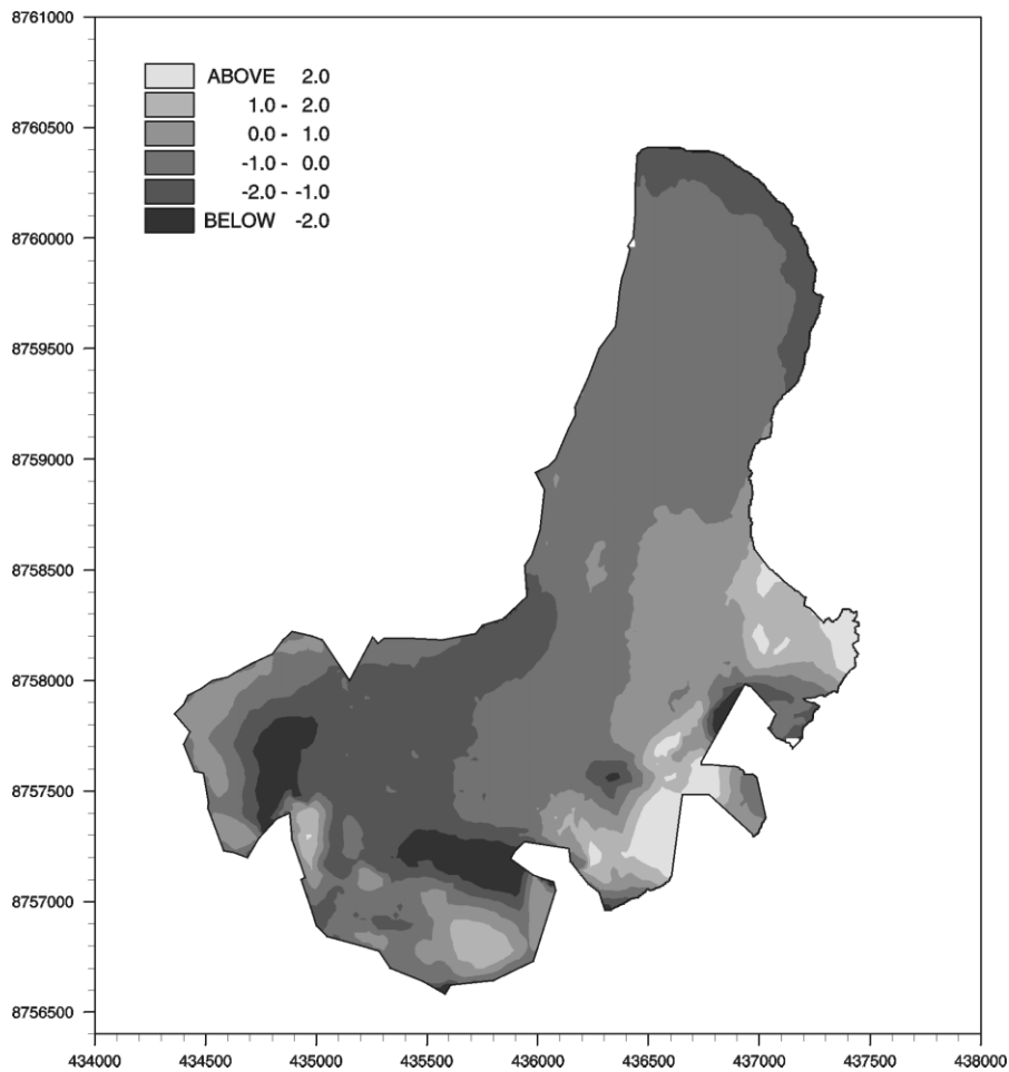
Figure 7. Surface height change (m w.e. a^{-1} ) between 1977 and 1995. Negative values indicate decreasing height (thinning); positive values indicate increasing height (thickening). Easting on x -axis; northing on y -axis; units are metres; north is to top of figure
