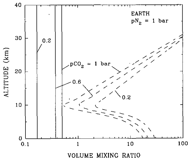
FIG. 6. Diagram illustrating the onset of \text{CO}_2 condensation in the standard outer edge model. Solid curves represent the \text{CO}_2 volume mixing ratio; dashed curves represent the saturation vapor pressure of \text{CO}_2 divided by the ambient atmospheric pressure.
