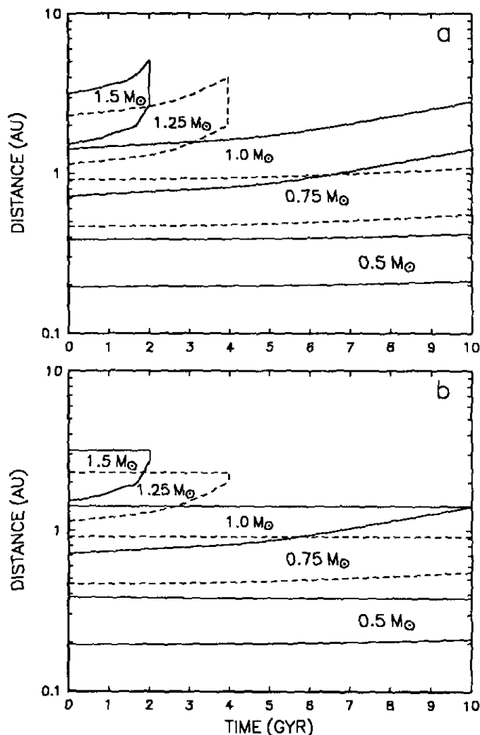
FIG. 14. Evolution of the HZ around different stars for two different assumptions about the possibility of planetary cold starts: (a) cold starts permitted, (b) no cold starts allowed. The intermediate (runaway and maximum greenhouse) estimates for the width of the HZ were used and the evolution was truncated at the end of the main sequence phase.
