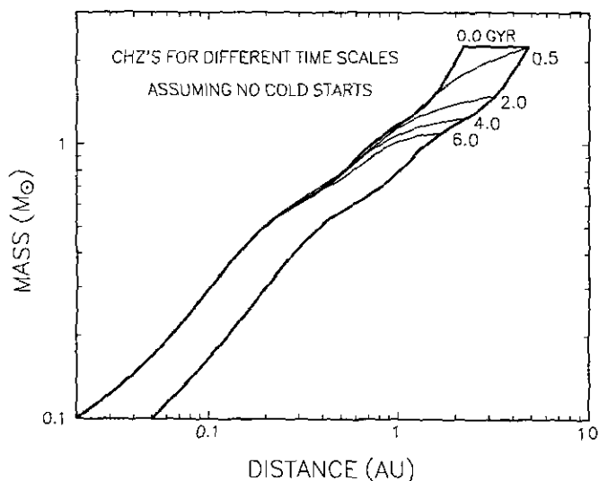
FIG. 15. CHZ widths as a function of stellar mass for different planetary habitability times, \tau_H , again using the intermediate HZ limits. The calculations shown here assume that planetary cold starts are not possible; thus, the inner edge of the CHZ moves outward as \tau_H increases, but the outer edge remains fixed. The \tau_H = 0 outer envelope corresponds to the HZ of a ZAMS star.
