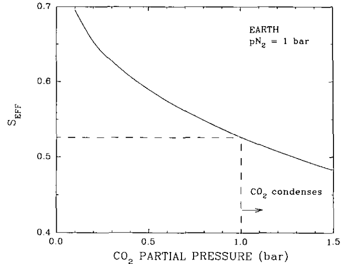
FIG. 7. The variation of effective solar flux with p\text{CO}_2 for the sequence of calculations shown in Fig. 6. The dashed lines show where \text{CO}_2 first condenses.
