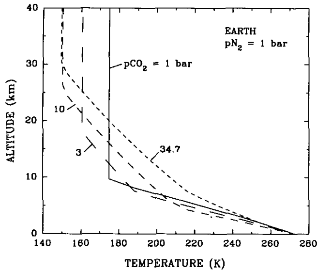
FIG. 5. Vertical temperature profiles for selected \text{CO}_2 partial pressures in the standard outer edge model.
