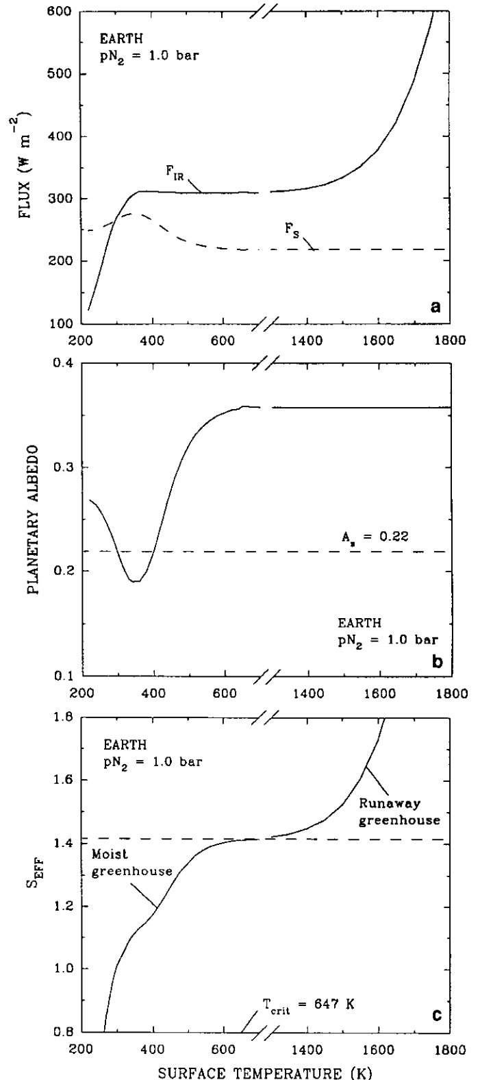
FIG. 1. Dependence of various quantities on surface temperature for the standard inner edge model: (a) outgoing infrared flux ( F_{\text{IR}} ) and net incident solar flux ( F_S ), (b) planetary albedo, and (c) effective solar flux. Note the scale break between 700 and 1300 K. The dashed curve in (b) shows the assumed surface albedo.
