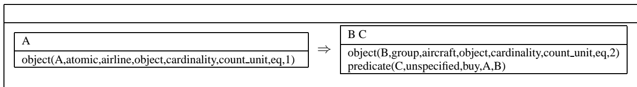
Figure 1: DRS corresponding to the ACE sentence “Every airline buys 2 aircraft.”
