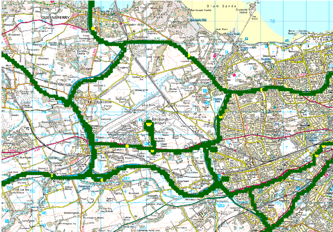
Figure 24: Edinburgh west and airport coverage, 4-QAM rate 1/3.
