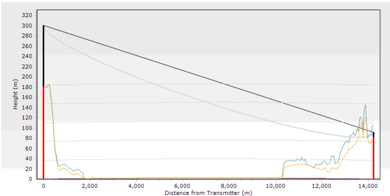
Figure 22: Path profile for light blue ring.
