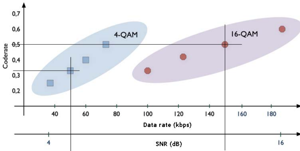
Figure 17: Comparison of data rate and required SNR in a Gaussian channel for different constellations and coderates.
