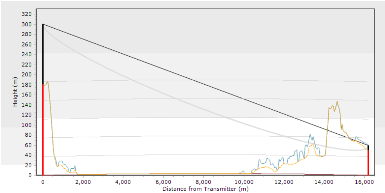
Figure 21: Path profile for dark blue ring.
