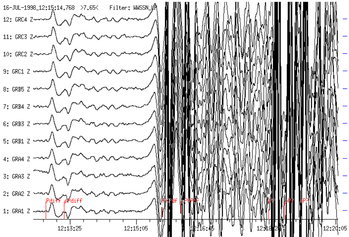
Figure 7b The same record as in Figure 7a, however, after long-period filtering (WWSSN-LP simulation). Note the pronounced onsets Pdfff and pPdfff. Also remarkable is the long-period and slowly emerging onset 24 sec before PKP.
