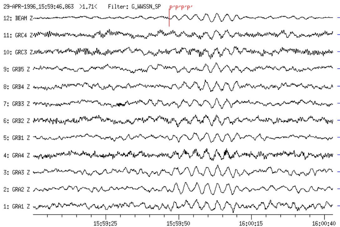
Figure 6d Short-period filtered (WWSSN-SP simulation) seismogram. The rare phase 4P' = P'P'P' (PKPPKPPKPPK) was clearly recorded at the GRF-array coming from opposite direction (BAZ = 226 and S = 2.56 s/°) about 63 min after the first P onset. Trace No.12 (the sum of all traces = BEAM) shows the best signal-noise-ratio.
