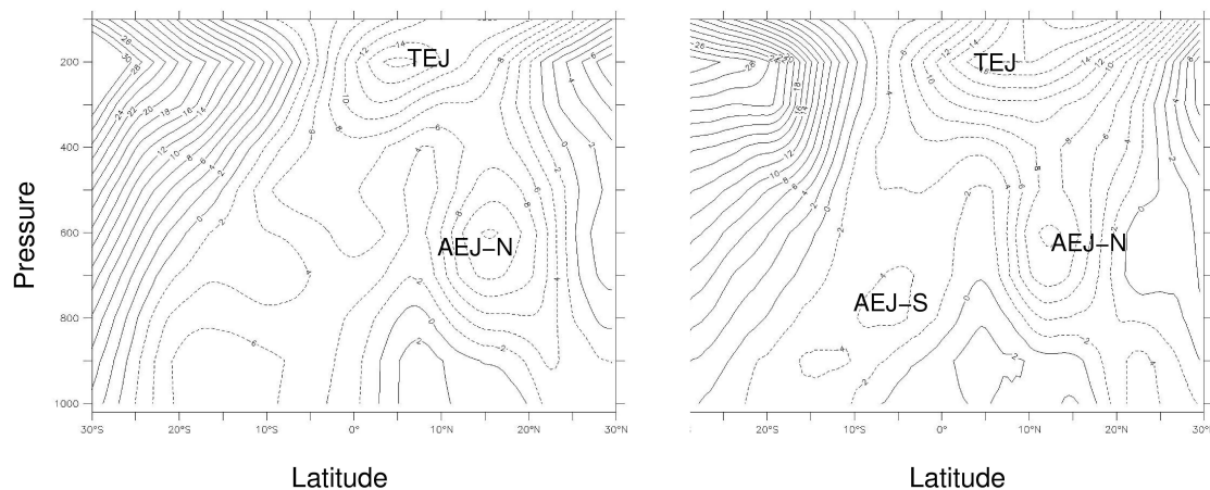
Fig. 1. Latitudinal cross section of ECMWF mean zonal wind speed ( \text{m s}^{-1} ) (a) for 25 July to 31 August, averaged between 30^\circ \text{W} and 10^\circ \text{E} , (b) for 25 July to 31 August, averaged between 10 and 30^\circ \text{E} .
