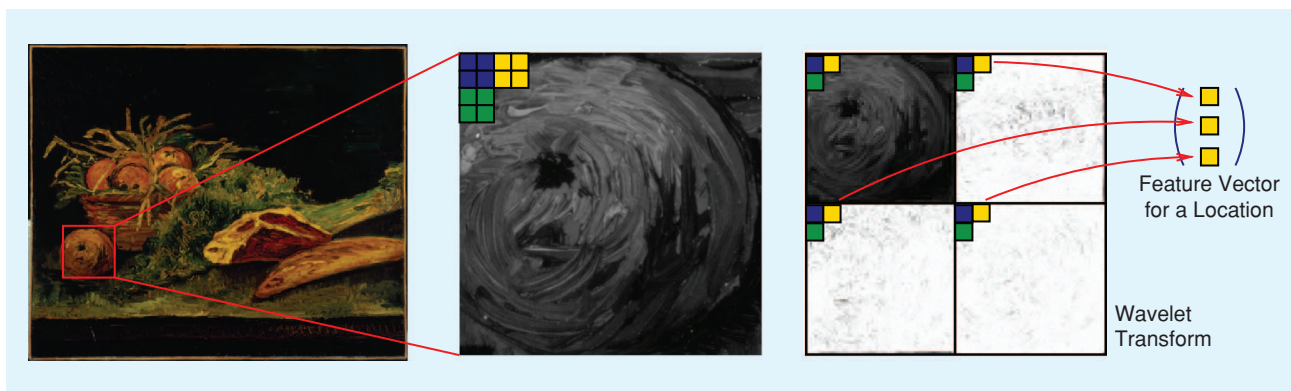
[FIG3] The formation of the texture feature vector based on the wavelet coefficients. The van Gogh painting F219 ( Still Life: Basket with Apples, Meat and a Breadroll ) is shown.
