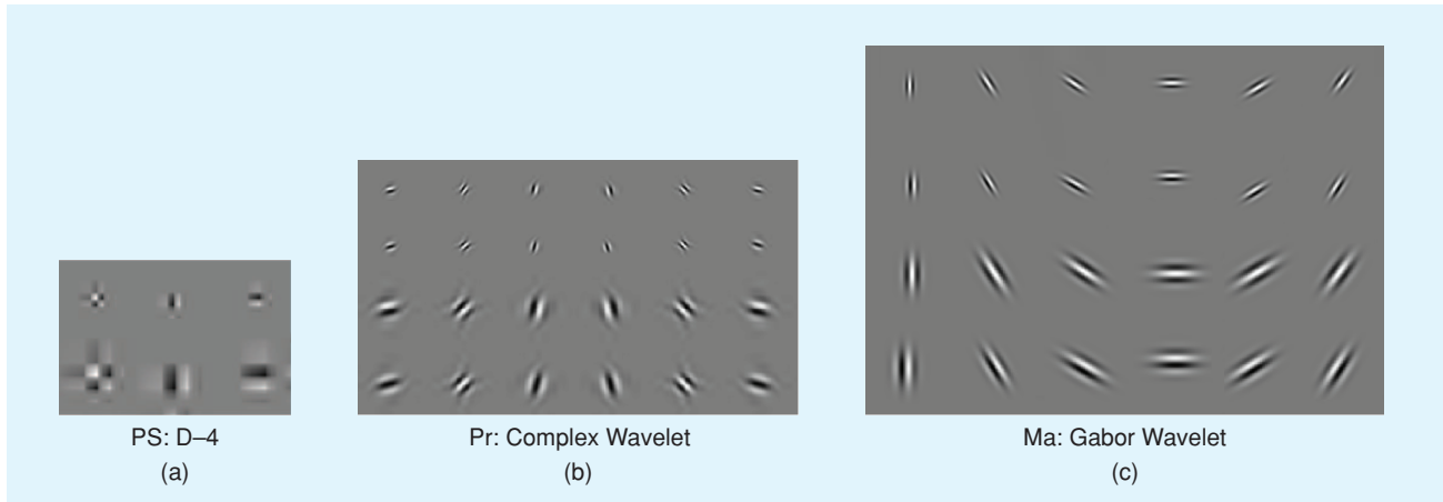
[FIG2] The three different choices for the wavelet templates (shown at the same size); in each case, wavelets are shown for two successive scales and at all the orientations.
