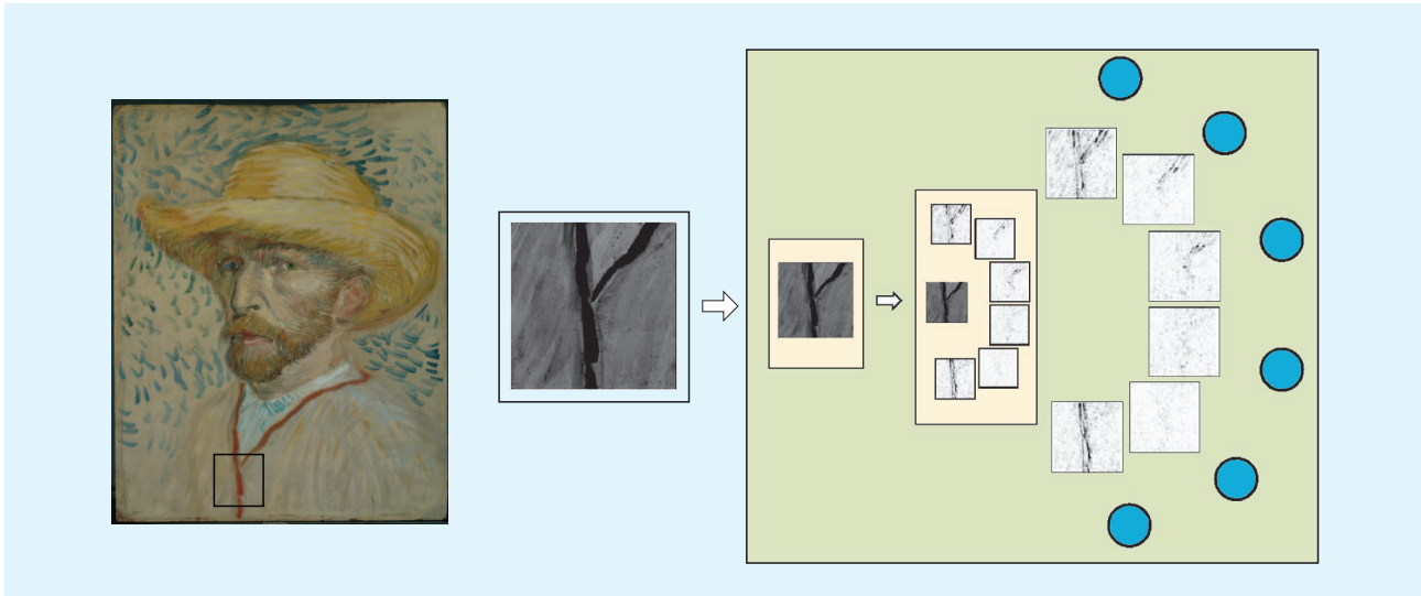
[FIG6] One patch in F469 ( Self Portrait with Straw Hat ) by van Gogh and two layers of its wavelet transform, along the six orientations, and its subsampled low-pass version. (Wavelet coefficients with larger/smaller magnitudes in darker/lighter gray.) For each scale s , there are four times more wavelet coefficients than for the next coarser scale ( s - 1 ).
