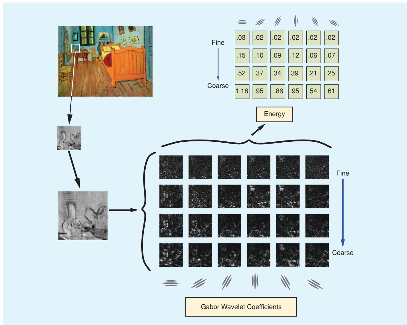
[FIG8] The image patch on the left, taken from F482 ( Vincent's Bedroom in Arles ), is decomposed by the Gabor wavelet transform into four scales and six orientations visualized on the right, where the rows represent scales (top to bottom: fine to coarse) and the columns orientations (left to right: counterclockwise from horizontal to almost horizontal). The numbers in each scale-orientation square give the energy value in each orientation-scale combination.
