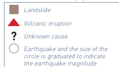
The four images above show confirmed tsunami source locations in the Pacific Ocean, Indian Ocean, Mediterranean Sea, and Caribbean Sea. The symbols indicate cause of the tsunamis: Brown Square is a landslide, Red Triangle is a volcanic eruption, Question Mark is an unknown cause, and White Circle is an earthquake and the size of the circle is graduated to indicate the earthquake magnitude. Source: NGDC / WDS-Geophysics.
