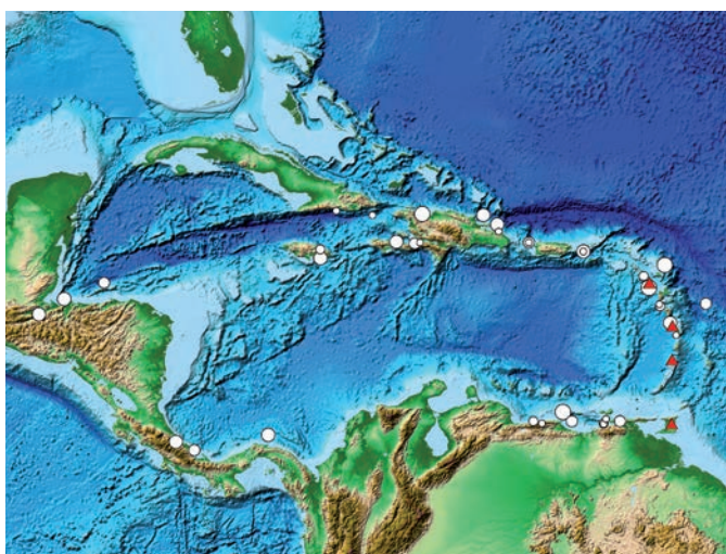
The four images above show confirmed tsunami source locations in the Pacific Ocean, Indian Ocean, Mediterranean Sea, and Caribbean Sea. The symbols indicate cause of the tsunamis: Brown Square is a landslide, Red Triangle is a volcanic eruption, Question Mark is an unknown cause, and White Circle is an earthquake and the size of the circle is graduated to indicate the earthquake magnitude. Source: NGDC / WDS-Geophysics.
