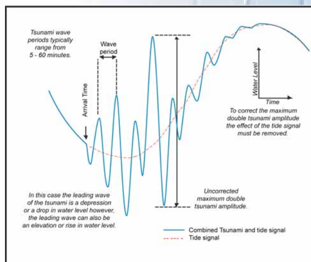
Mareogram (sea level) record of a tsunami.
