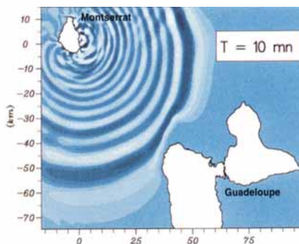
Numerical modelling snapshots of the water surface 10 minutes after a pyroclastic flow on the southeastern part of Montserrat Island led to a submarine landslide and the generation of a tsunami.
