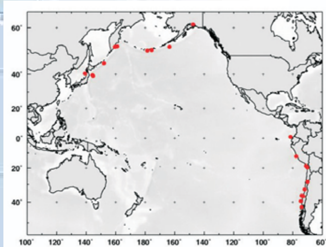
More than 80% of the world's tsunamis are observed in the Pacific where large earthquakes occur as tectonic plates are subducted along the Pacific Ring of Fire. Top: Epicentre of all tsunamigenic earthquakes. Middle: Epicentre of tsunamis causing damage or casualties. The Southwest Pacific is a source area of local and sub-regional destructive tsunamis. Bottom: Epicentre of tsunamis causing damage or casualties more than 1,000 km away. These are the tsunami hazard zones for destructive Pacific-wide tsunamis based on historical records. Source: Pacific Tsunami Warning Center.
