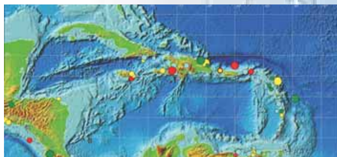
Earthquakes generating tsunamis in the Caribbean and adjacent seas. Source: ITDB, 2005.
