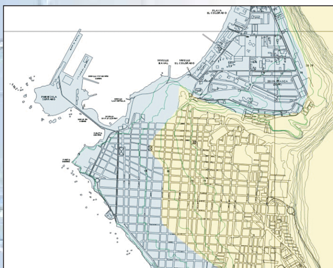
Estimated tsunami inundation at Iquique, Chile, based on numerical model results.
