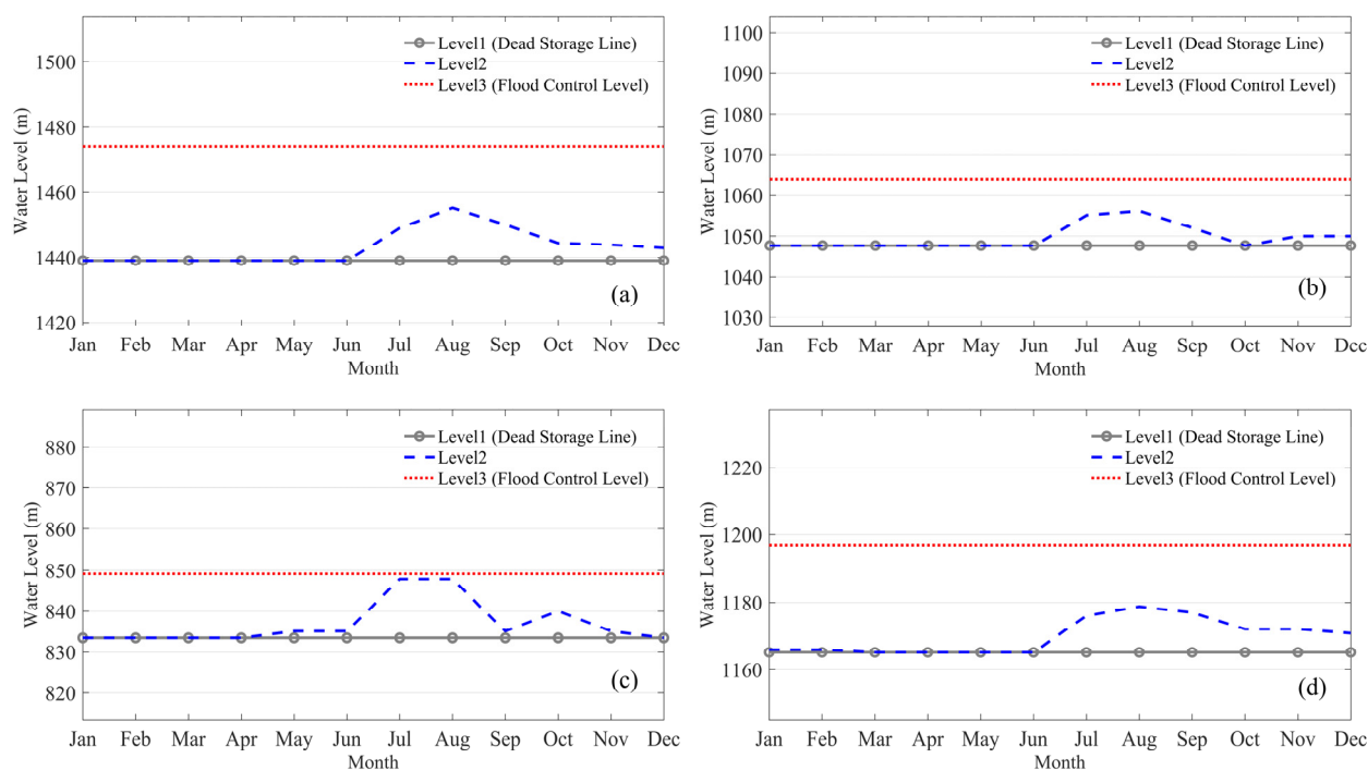
Figure 3 Regulation curves of four reservoirs for three rivers, a) the Ertanggou (ETG), b) the Kekeya (KKY), c) KKY2, and d) the Kanerqi (KEQ).
