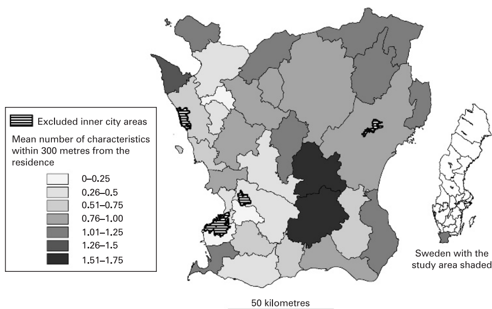
Figure 1 Mean number of recreational values of the natural environment within 300 metres distance from the residence in each of the 33 municipalities in the Scania region (range 0.08 for Staffanstop municipality in the southwest to 1.68 recreational values on average for Hörby municipality in the middle of Scania).
