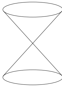
FIGURE 8.3. The cone \text{Spec } k[x, y, z]/(z^2 - x^2 - y^2) .
