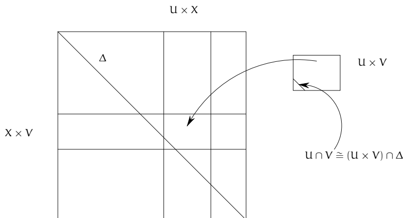
FIGURE 10.2. Small Proposition 10.1.6
