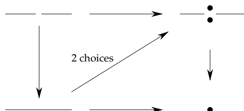
FIGURE 12.6. The line with the doubled origin fails the valuative criterion for separatedness
