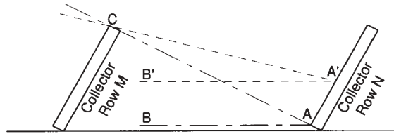
Figure 1.9.3 Section of two rows of a multirow collector array.
