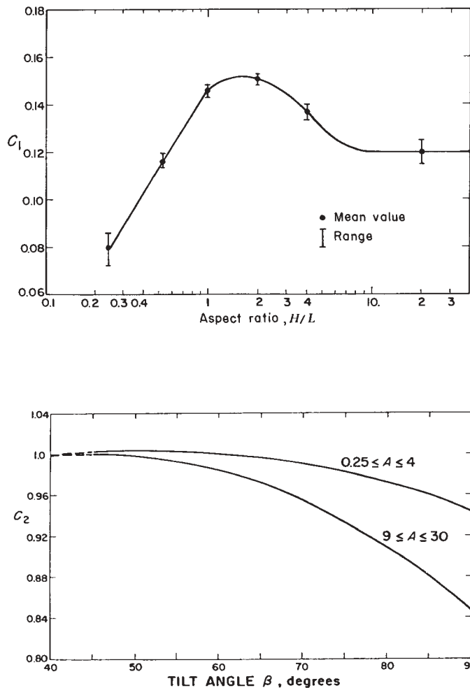
Figure 3.12.2 Coefficients C_1 and C_1 for use in Equation 3.12.1. From Meyer et al. (1978).
