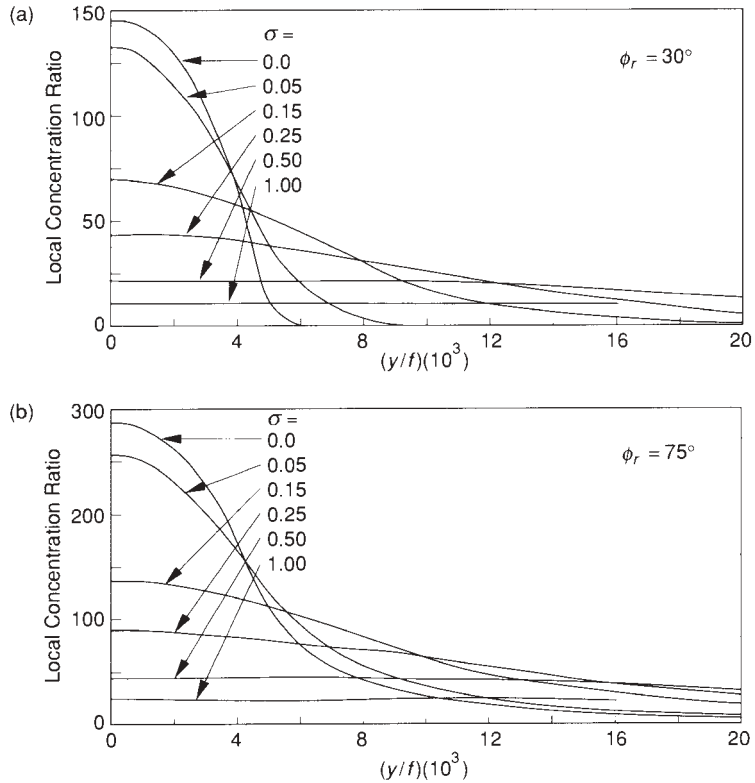
Figure 7.11.1 (a) Image distributions for imperfect reflectors for 30° rim angle for various standard deviations of normally distributed reflector slope errors, (b) Image distributions for imperfect reflectors for 75° rim angle for various standard deviations of normally distributed reflector slope errors. From Evans (1977).
