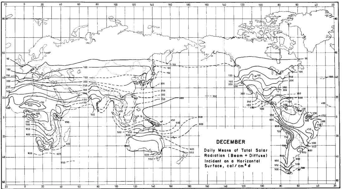
Figure 2.5.2 Average daily radiation on horizontal surfaces for December. Data are in \text{cal/cm}^2 , the traditional units. Adapted from deJong (1973) and Lóf et al. (1966a).
