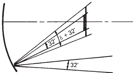
Figure 7.11.2 Schematic of a portion of a concentrator with a dispersion angle \delta added to the 0.53° solar intercept angle.
