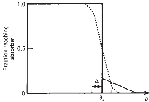
Figure 7.6.2 Fraction of radiation incident on the aperture of a CPC at angle \theta which reaches the absorber surface if \rho = 1 : \theta_c = acceptance half-angle, \Delta = angular surface error. (—) Full CPC with no surface errors; (-----) truncated CPC with no surface errors; (·····) full CPC with surface errors. Adapted from Rabl (1976b).
