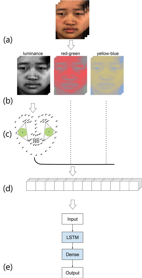
LSTM model
