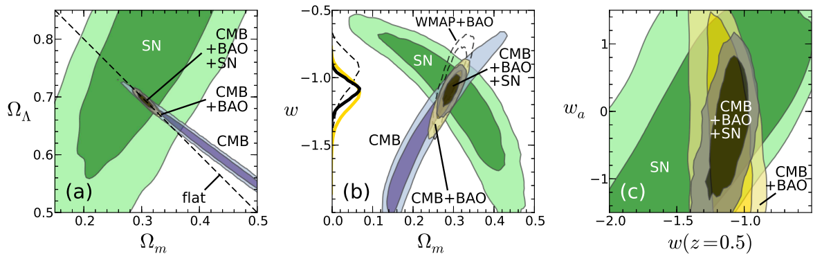
Figure 26.2: Constraints on the present matter fraction \Omega_m and dark energy model parameters. Dark and light shaded regions indicate 68.3% and 95.4% confidence levels, respectively. “CMB” is Planck+WP, “BAO” is the combination of SDSS-II, BOSS, and 6dFGS, and “SN” is Union2. (a) The present dark energy fraction \Omega_\Lambda vs. \Omega_m , assuming a \Lambda CDM model. CMB data, especially when combined with BAO constraints, strongly favor a flat universe (diagonal dashed line). (b) The dark energy equation of state w vs. \Omega_m , assuming a constant value of w . The dashed contours show the 68.3% and 95.4% CL regions for the combination of WMAP9 and BAO data. Curves on the left vertical axis show the probability distributions for w (normalized arbitrarily), after marginalizing over \Omega_m , for the CMB+BAO and CMB+BAO+SN combinations (yellow and black, respectively), using Planck+WP CMB data, and for the WMAP9+BAO combination (dashed black). (c) Constraints on the two parameters of the dark energy model with a time-dependent equation of state given by Eq. (26.4): w(z = 0.5) and w_a = -dw/da .
