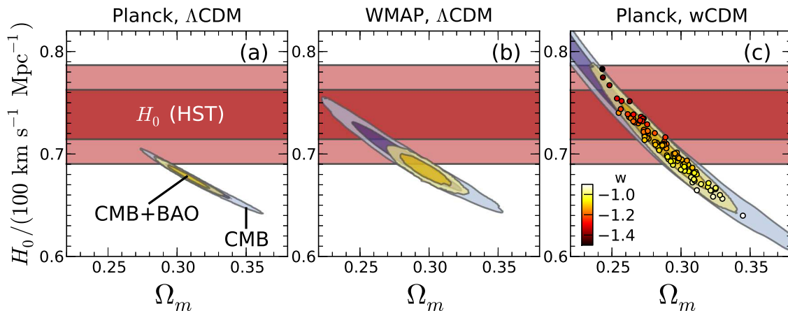
Figure 26.3: Constraints on the present matter fraction \Omega_m and the Hubble constant H_0 from various combinations of data, assuming flat \Lambda CDM (left and middle panels) or a constant dark energy equation of state w (right panel). Dark and light shaded regions indicate 68.3% and 95.4% confidence levels, respectively. The right panel also shows 100 Monte Carlo samples from the CMB+BAO constraints with the value of w indicated by the colors of the dots. “CMB” is Planck+WP in the outer panels and WMAP9 in the middle panel, “BAO” is the combination of SDSS-II, BOSS, and 6dFGS, and “ H_0 (HST)” is the HST constraint from [40].
