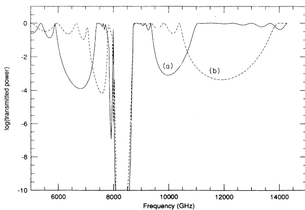
FIG. 3. The transmitted power vs frequency in a similar system as in Fig. 1 for E -polarized EM wave and two different lattice constants (a) d = 7.54 \mu\text{m} , (b) 5.65 \mu\text{m} . The dielectric constant is frequency dependent and is given by Eq. (8).
