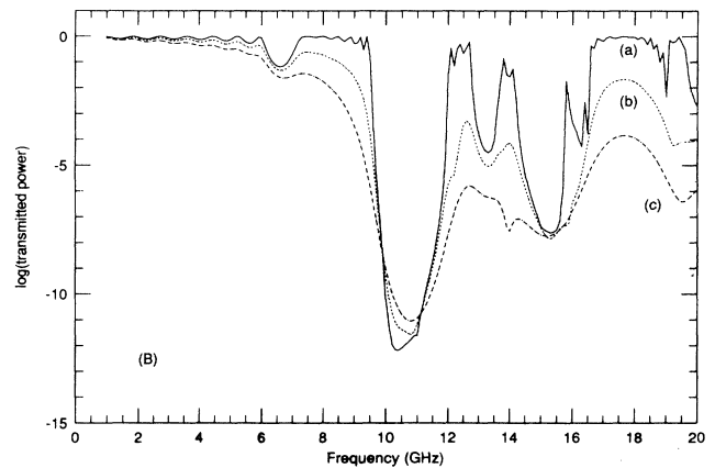
FIG. 1. The transmitted power vs frequency for a 2D square lattice consisting of cylinders with f = 0.449 surrounded by air for E - and H -polarized EM waves (A and B panels, respectively) propagating along the (1,0) direction (there are eight layers of cylinders along this direction); the real part of \epsilon is 9 and the imaginary part is 0 (a); 0.4 (b); 1 (c); d = 1.27 cm. Power is in arbitrary units.
