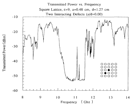
FIG. 6. The experimental power vs frequency for a 2D square lattice consisting of ( 9 \times 18 ) cylinders with f = 0.449 and \epsilon=9 surrounded by styrofoam ( \epsilon=1.04 ). Two cylinders are removed from near the center of the lattice. [Experiments by Schultz et al. (Ref. 12)].
