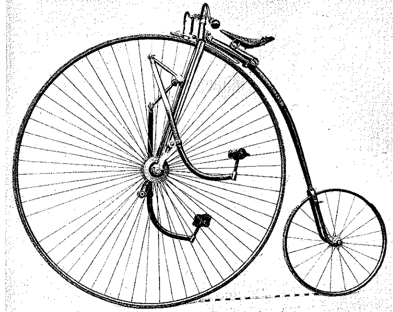
Figure 15 Singer Xtraordinary bicycle (1878). Photograph courtesy of the Trustees of the Science Museum, London.
