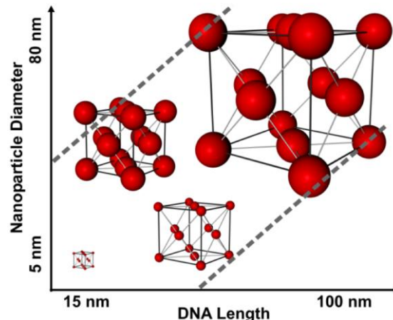
Figure 3.13 Illustration of the “zone of crystallization” (denoted by dashed lines) in which certain combinations of nanoparticle size and DNA length are able to form ordered superlattices. Modeled unit cells are drawn to scale relative to one another (Macfarlane et al. 2010).
