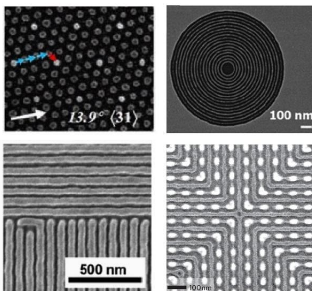
Figure 3.4. Four examples of nanostructure patterns fabricated by directed self-assembly using diblock copolymers (sources: upper left , Bita et al. 2008; upper right , Chai and Buriak 2008; lower left , Galatsis et al. 2010; lower right , Yang et al. 2010).
