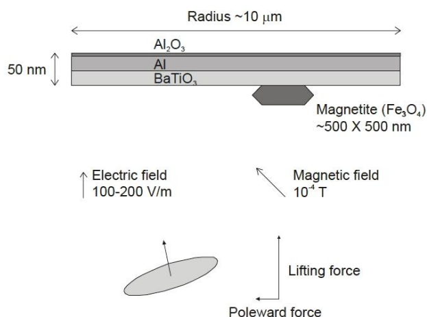
Figure 5.16. Conceptual design of a self-levitated nano-disk for SRM geoengineering (Keith 2008). This nano-disk configuration is theoretically designed to have 3 properties: (1) the aluminum layer ~25 nm thick would be reflective in the visible and transparent in the infrared portion of the electromagnetic spectrum; (2) the nano-disks would self-levitate in the stratosphere due to the interaction of the barium titanate (BaTiO 3 ) with the natural electric-field (100-200 V/m) in the stratosphere; and (3) the nano-disks would “tilt” due to the off-center presence of the magnetic iron oxide (Fe 3 O 4 ) interacting with the Earth’s magnetic field in the stratosphere, leading to the nano-disks being pushed by Brownian forces in the direction of the Earth’s magnetic
