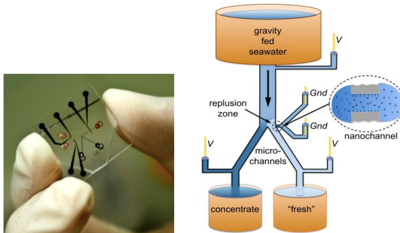
Figure 5.10. A chip-sized nanofluidic device ( left ) desalinates water at an energy use approaching that of a large-scale reverse osmosis desalination system (Kim et al. 2010).
