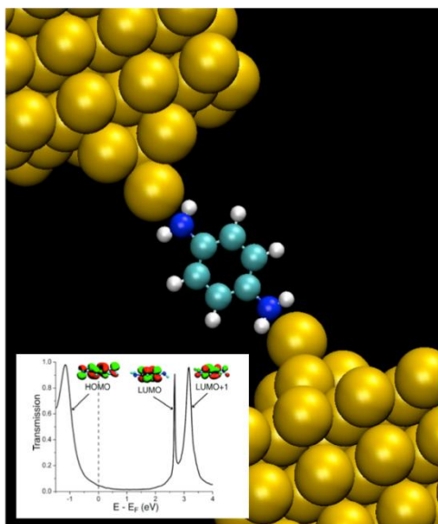
Figure 1.1. First-principles density functional theory (NEGF-DFT) simulations of the conductance of molecular junctions have led to improved understanding and quantitative agreement with experiments. The figure shows the calculated atomic geometry of benzene-diamine suspended between Au electrodes; the inset shows the computed electron transmission vs. energy (Quek et al. 2007).
