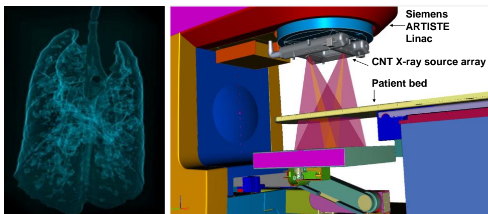
Figure 7.9. Left: Prospective-gated micro-CT image of a mouse lung tumor model (UNC data. Mouse model from Dr. B. Kim). Right: An illustration of a CNT x-ray source array mounted on a radiotherapy machine (image courtesy of J. Maltz of Siemens and P. Lagani of XinRay Systems).
