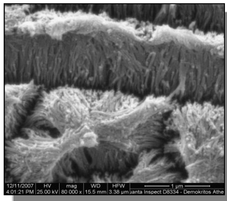
Figure 3.26. Random branching alumina nanotubes (Kokonou 2008).
