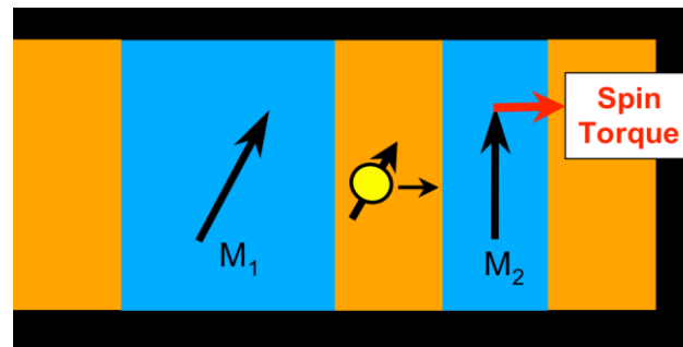
Figure 8.4. Spin-polarized electrons produced by spin filtering from one magnetic layer can apply a strong torque to a second magnetic layer downstream (courtesy of D. Ralph.)
