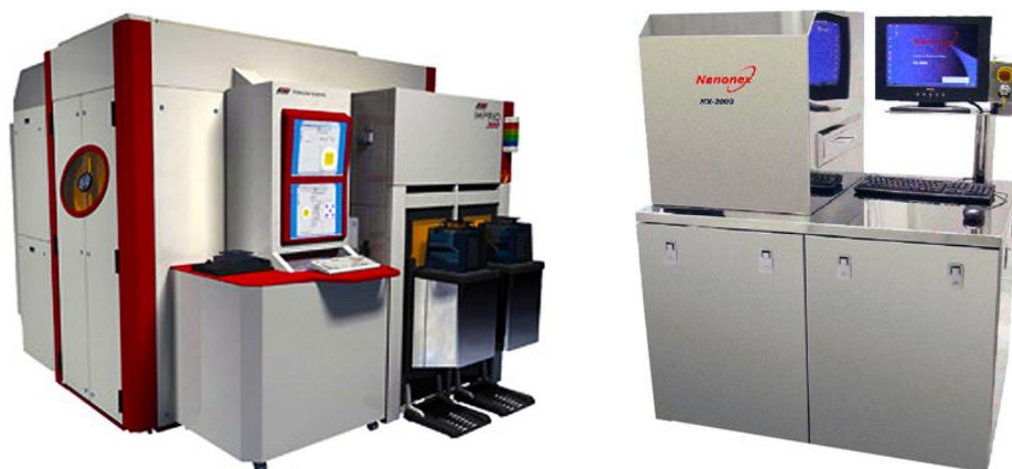
Figure 2.9. Lithography tools for nanoscale manufacturing. (Left) Molecular Imprints, Inc. (left, Imprio® 300, http://www.molecularimprints.com/products.php ). (Right) Nanonex Corp. (right, NX-2000, http://www.nanonex.com/machines.htm ).
