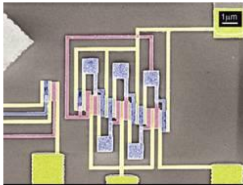
Figure 8.7. Implementation of a CMOS-type 5-stage ring oscillator on a single carbon nanotube (Chen et al. 2006).
