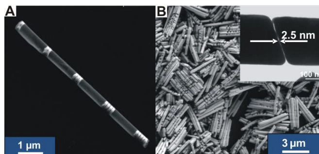
Figure 3.10. Structures made by OWL. (A) Disk arrays (adapted from Qin et al. 2006). (B) Zoomed out image demonstrating uniformity of rods (Qin et al. 2005). (B inset) 2.5-nm gap produced by means of OWL (Qin et al. 2007).
