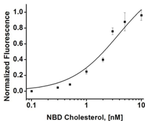
Figure 7.16. Binding isotherm of a fluorescent cholesterol analogue to HDL-AuNPs. NBD cholesterol was titrated into a 5 nM solution of HDL-AuNPs. The fluorescence vs. NBD-cholesterol concentration was used to calculate the K_d of HDL-AuNPs (courtesy of C.S. Thaxton).
