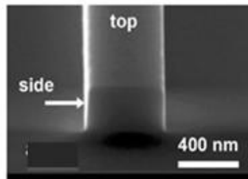
Figure 9.10. Silicon waveguide.
