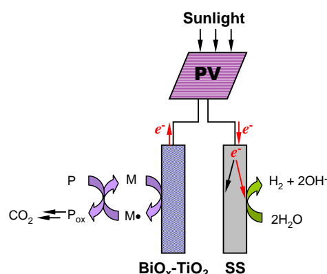
Figure 5.11. Solar-powered photocatalytic systems for sustainable water reuse.
