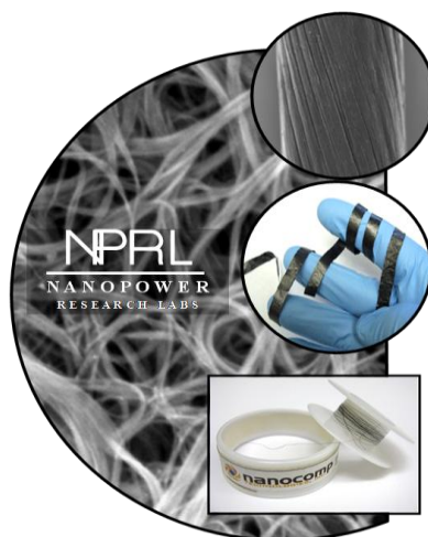
Figure 3.24. Scanning electron micrograph of SWCNTs with insets. Cross-section of a wire ( top ); single-wall carbon nanotube ribbon cable ( middle ); carbon nanotubes thread ( bottom ). (courtesy of Nanopower Research Labs at Rochester Institute of Technology: http://www.sustainability.rit.edu/nanopower/ ).
