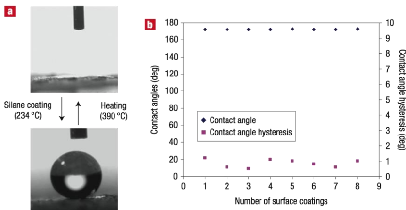
Figure 5.13. Nanowire membranes with tunable surface wetting properties (Yuan et al. 2008). (a) Reversible transition between superhydrophilic ( top ) and superhydrophobic ( bottom ); (b) contact angles and hysteresis measurements between cycles.
