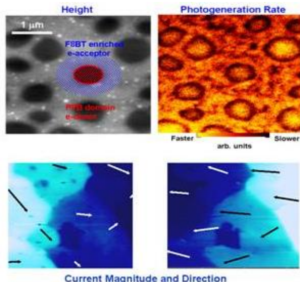
Figure 2.3. ( Top ) Simultaneous imaging of structure and photo current generation in an organic solar cell (Coffee and Ginger 2006), and ( bottom ) imaging of current magnitude (size of vector) and direction across an operating oxide device (Bonnell and Kalinin 2001).
