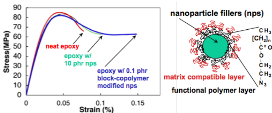
Figure 11.13. Improved epoxy nanocomposites for electrical insulation have increased strain-to-failure, fatigue resistance, electrical breakdown strength (30%), thermal conductivity, and endurance strength (x10), and lower constant of thermal expansion (CTE).
