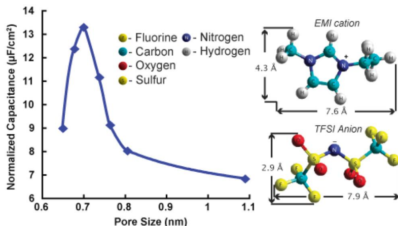
Figure 3.20. Normalized capacitance change versus the pore size of the carbide-derived carbon samples tested in an ionic liquid electrolyte. Normalized capacitance is obtained by dividing the gravimetric capacitance by the specific surface area. HyperChem models of the structure of ethyl-methylimidazolium (EMI) and bis(trifluoro-methane-sulfonyl)imide (TFSI) ions show a size correlation (Largeot et al. 2008).
