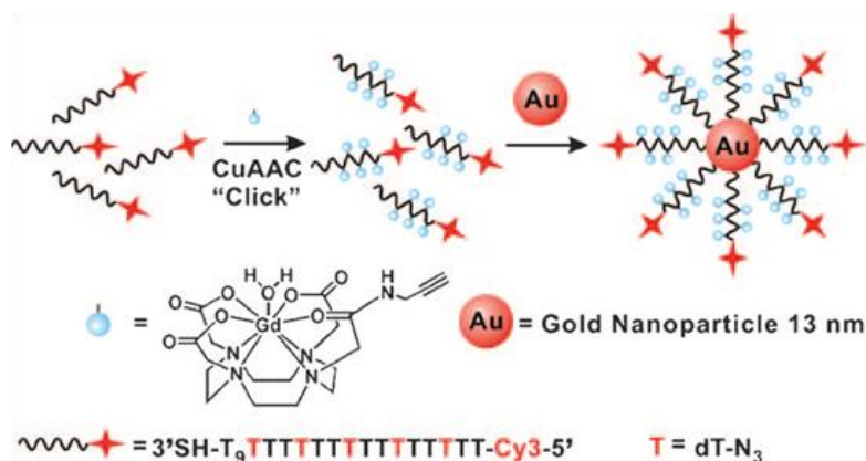
Figure 7.10. Schematic of Cy3-DNA-GdIII@AuNP conjugates. Gd(III) complexes are covalently attached to fluorescent DNA using click chemistry and conjugated to Au nanoparticles. The resulting nanoconjugate is stable, multimodal (MR, fluorescence, and CT), and cell permeable (Song et al. 2009).
