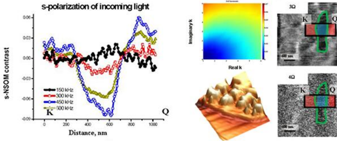
Figure 2.12. The scattered NSOM signal profiles ( left ) and images ( right ) are compared to a model of the complex dielectric function of a molecular layer ( top, right ) and the topographic structure ( bottom, right ) (Nikiforov et al. 2009).
