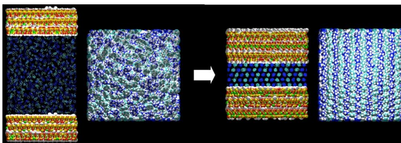
Figure 1.12. Upon sufficient nanoconfinement, cyclohexane undergoes a rapid and abrupt transition to a layered and hexagonal ordered, solid-like structure. In the configurations, the mica sheets are shown and the cyclohexane rendered in stick form on the left, so that it is easy to see through the confined fluid; the confined fluid, rendered in full size without mica, is shown on the right, looking down from above. Cyclohexane molecules (H atoms white, C atoms shades of blue) are colored in two different shades of gray, making the resulting order apparent (from Docherty et al. 2010).
