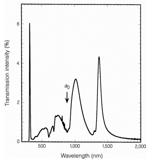
Figure 9.3. Zero-order transmission spectrum for a square array of 150 nm holes with a period of 900 nm in a 200 nm thick Ag film. The maximum transmitted intensity occurs at 1370 nm, nearly ten times the diameter of an individual hole in the array (Ebbesen 1998).
