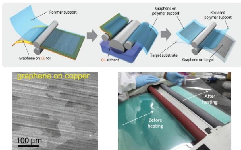
Figure 3.16. Images of large scale production of graphene grown on copper foils and transferred to a polymer layer for use in large area display applications (from Li et al. 2009 and Bae et al. 2010).
