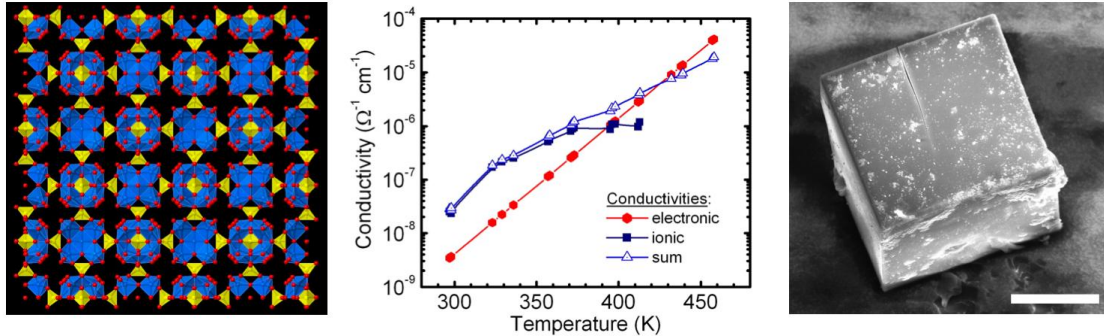
Figure 3.21. (Left) Zeoate framework structure with [(As_6VIV_{12}VV_3O_{51}) - 9Z]_{\infty} composition, where vanadium is blue, arsenic is yellow, and oxygen is red. The material crystallizes in a cubic space group with cell edge of 1,600 pm. (Middle) Plot of measured conductivities as a function of temperature (data from Soghomonian and Heremans 2009). (Right) Scanning electron micrograph of zeoate material from left panel; scale bar is 50 \mu\text{m} (courtesy of V. Soghomonian, Virginia Polytechnic Institute and State University).
