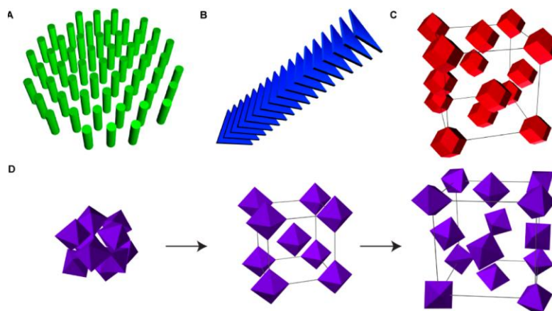
Figure 3.14. Models of superlattices derived from DNA-mediated assembly of anisotropic nanostructures. (A) 2D hexagonal arrangement of nanorods. (B) 1D columnar ordering of triangular nanoprisms. (C) Face-centered cubic ordering of rhombic dodecahedra. (D) Illustration of the transition from disordered to BCC to FCC ordering with increasing linker length in the assembly of octahedra (Jones et al. 2010).
