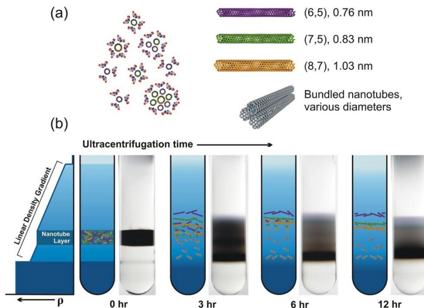
Figure 11.8. (a) Cross-sectional schematic of surfactant-encapsulated SWNTs; three specific SWNT chiral vectors and respective diameters are identified. (b) Schematic representation and corresponding photographs of an ultracentrifuge tube at four different points in the DGU process (courtesy of Mark Hersam, Northwestern University).
