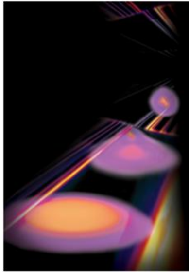
Figure 1.13. Conductance spectroscopy through a nano-scaled transistor dominated by a single impurity. One of several measured Coulomb diamonds is depicted in the background with three different gate-field-dependent single-electron wave functions bound to a single impurity (after Lansbergen, Rahman et al. 2008).
