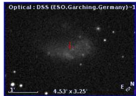
Fig. 6: Irregular galaxy NGC1427A.
