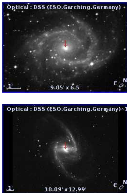
Fig. 4: Spiral galaxies NGC2997 (Sc, top) and NGC1365 (SBb, bottom).
