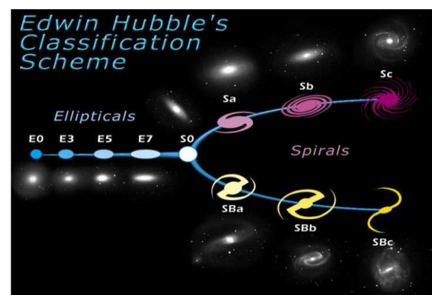
Fig. 1: The Hubble Sequence: a morphological classification scheme for galaxies.
