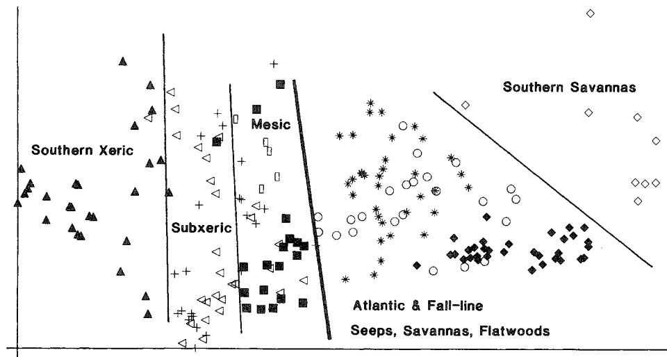
Figure 3. Ordination 1 contains all samples used in the final analysis. The first axis corresponds primarily to a moisture gradient with Xeric Longleaf Woodlands on the left, and moist savannas and flatwoods on the right. Among the moist sites, the Southern Longleaf Savannas (◇) are most distinctive and extreme, but Atlantic Longleaf Savannas (◆) separate from the Fall-line Longleaf Seepage Savannas (○) and Atlantic Longleaf Flatwoods (*). While Southern Xeric Longleaf Woodlands (▲) are well separated, the Atlantic (+) and Fall-line Xeric Longleaf Woodlands (+) are inter-mixed with the Subxeric Longleaf Woodlands (◻). Piedmont/Upland Subxeric Longleaf Woodlands (◻) are mixed with the Mesic Longleaf Woodlands (■).
