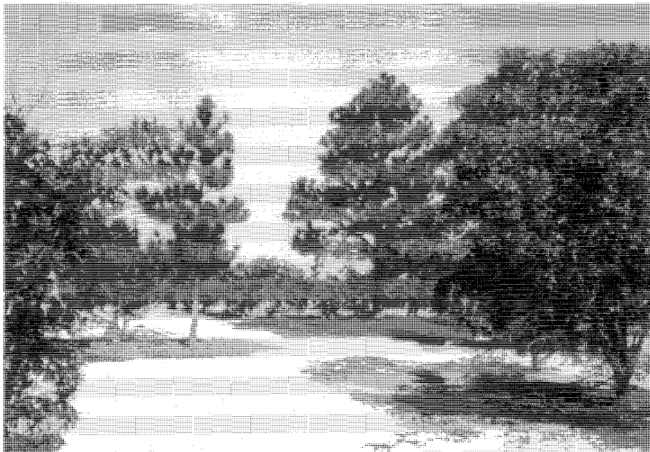
Figure 7. Atlantic Xeric Longleaf Woodland. The xeric extreme of longleaf vegetation on the Atlantic coastal plain is found on the eolian dune sands along the northeast sides of Carolina bays and major rivers. Salters Lake, Bladen County, North Carolina.
