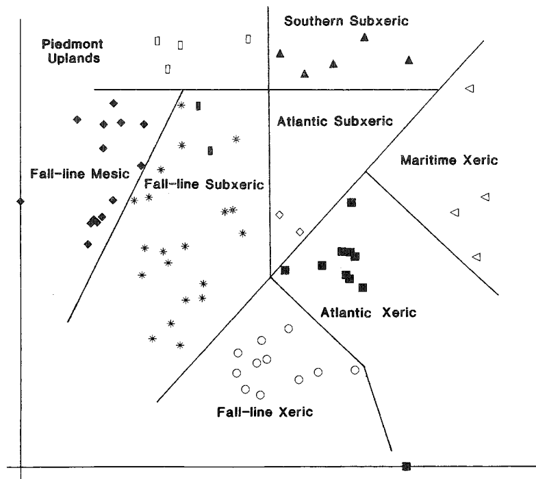
Figure 5. Ordination 3 resulted after reordinating the dry site dataset after removal of the Southern Xeric Longleaf, Subxeric Longleaf-Palmetto, and Southern Mesic Longleaf sites (defined by the bold lines in Figure 4) and the single Serpentine Subxeric Longleaf sample. A moisture gradient runs from the Xeric Longleaf Woodland sites in the lower right (○ = Fall-line; ■ = Atlantic; △ = Atlantic Maritime) to the Fall-line Mesic (♦) and Piedmont/Upland (◻) sites in the upper left. The perpendicular gradient is principally geographic with Fall-line Slope (■) and Subxeric sites (*) in the lower left and Southern (▲) and Atlantic Subxeric sites (◻) in the upper right. At this point the various Xeric and Subxeric types are distinct and separate from the Mesic sites.
