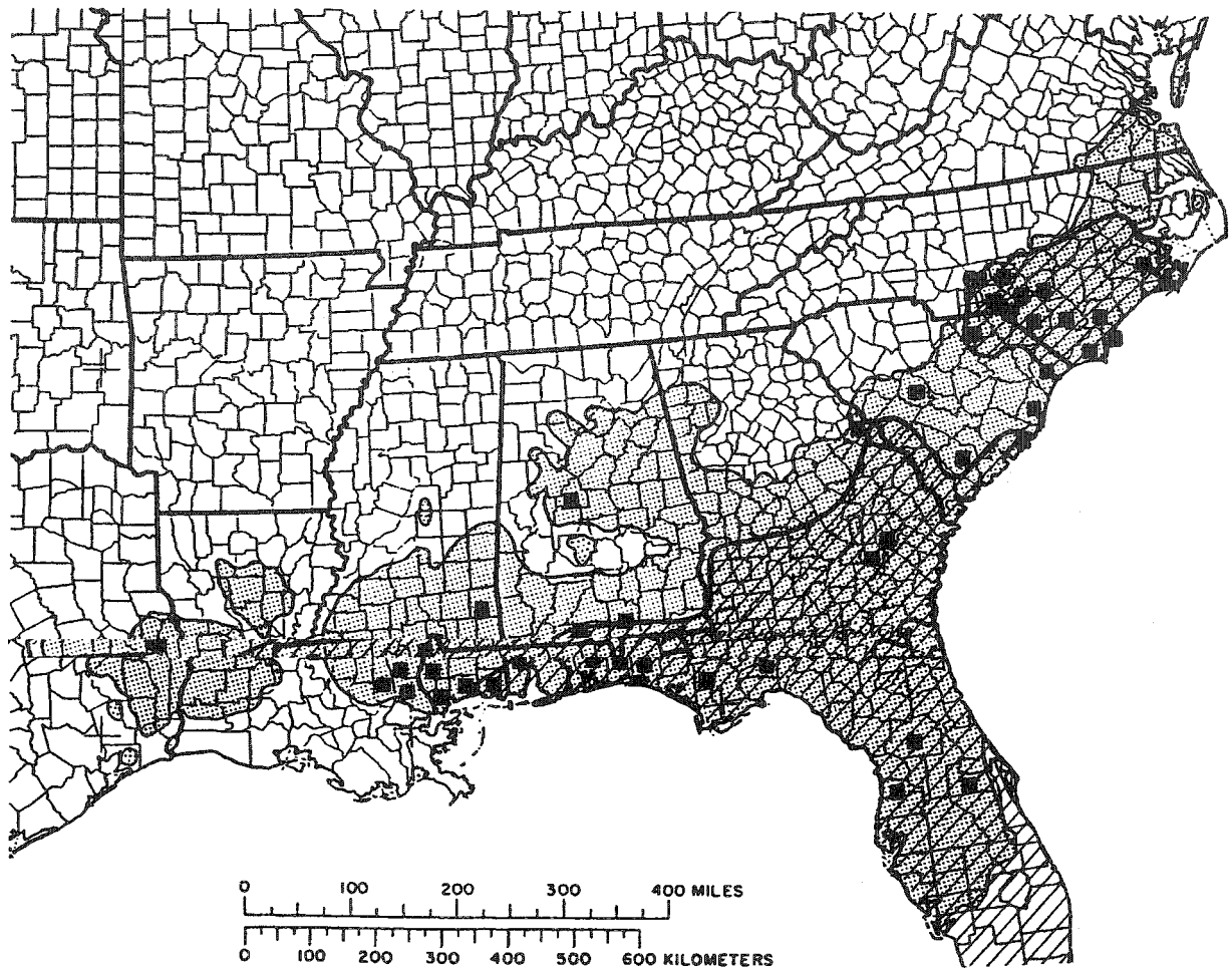
Figure 1. The 216 sample sites used in our final analysis were located in 44 counties scattered throughout much of the range of longleaf pine ( Pinus palustris ) east of the Mississippi River. The range of longleaf pine is indicated by stipples (after Little 1971 and Frost 1993) and the range of wiregrass ( Aristida stricta and A. beyrichiana ) by diagonal shading (after Peet 1993).
