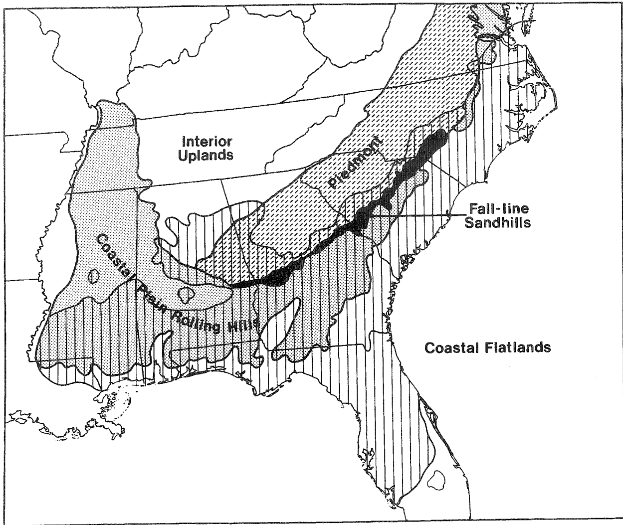
Figure 2. Longleaf pine (vertical lines) is distributed across several physiographic provinces, each with relatively distinct, longleaf-dominated communities (longleaf distribution after Little 1971 and Frost 1993; physiographic provinces modified from Hammond 1964 and Hodgkins 1965).
