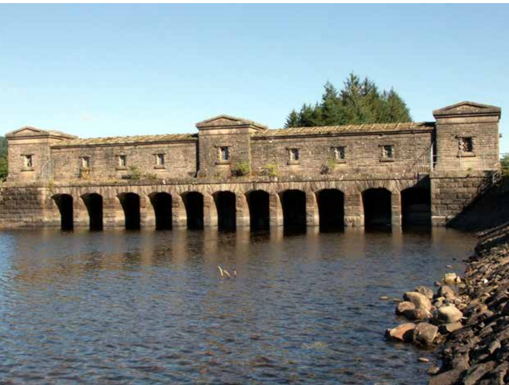
Loch Venacher sluice house controls the water flow along the Loch Katrine scheme designed by civil engineer John Frederic Bateman for the Glasgow Waterworks in 1856-59. (© Sheila Winstone, Creative Commons)
