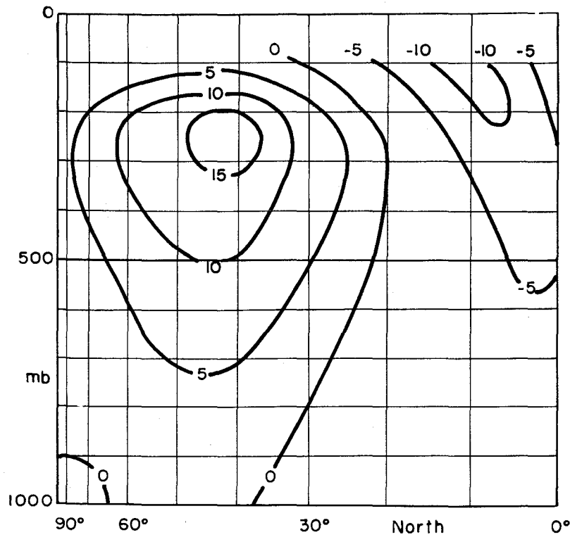
Figure 8. — The time-and-longitude averaged zonal wind [\bar{u}] in northern summer (June-August) as estimated by Mintz (1954). Values are in m\ sec^{-1}
