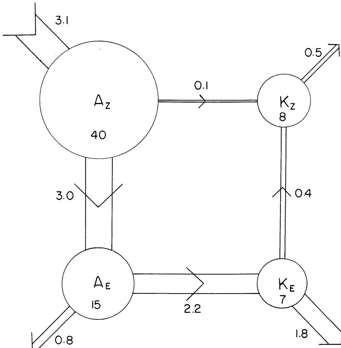
Figure 54. — The energy cycle of the atmosphere as estimated by Oort (1964a). Values of energy are in units of 10^9 \text{ joules m}^{-2} , and values of generation, conversion, and dissipation are in \text{watts m}^{-2} . The estimated value of conversion from A_z to K_z is smaller than the probable error of the estimate
