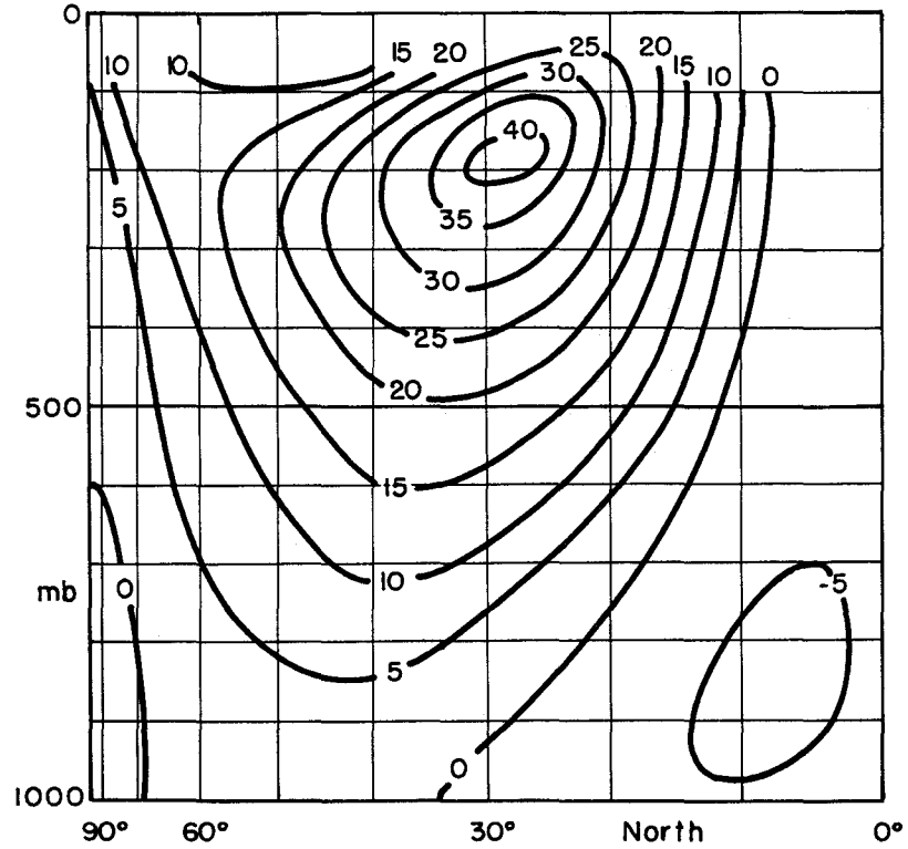
Figure 7. — The time-and-longitude averaged zonal wind [\bar{u}] in northern winter (December-February) as estimated by Mintz (1954). Values are in m\ sec^{-1}
