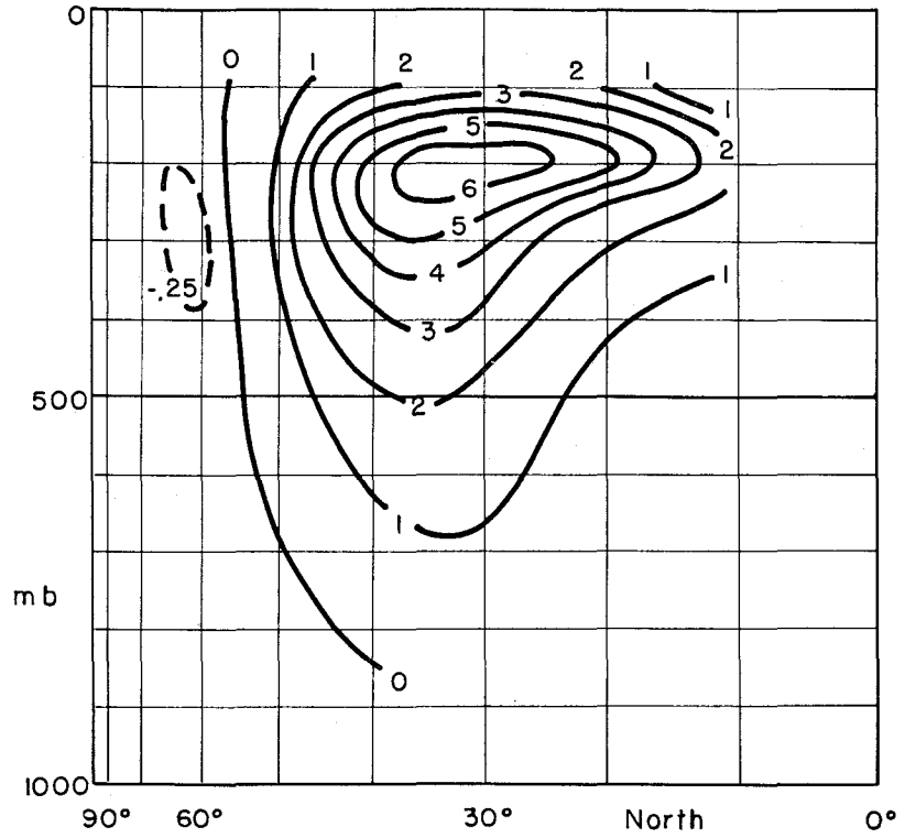
Figure 48. — The vertical distribution of the average northward transport of angular momentum by the eddies as estimated by Holopainen (1966). The unit is 10^{25} g \text{cm}^2 \text{sec}^{-2} per 100 mb layer
