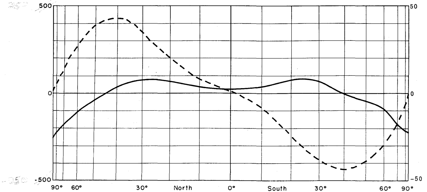
Figure 28. — The average net gain of energy from environment by the atmosphere (solid curve), as given by Sellers (1966) in \text{watts m}^{-2} (scale on left); and the northward transport of energy by the atmosphere required for balance (dashed curve), in units of 10^{14} watts (scale on right)
