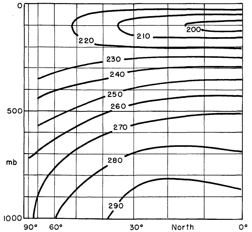
Figure 11. — The time-and-longitude averaged temperature \bar{T} in northern summer (April-September) as estimated by Peixoto (1960) (1000 mb-100 mb) and Peng (1963, 1965) (100 mb-30 mb). Values are in degrees K
