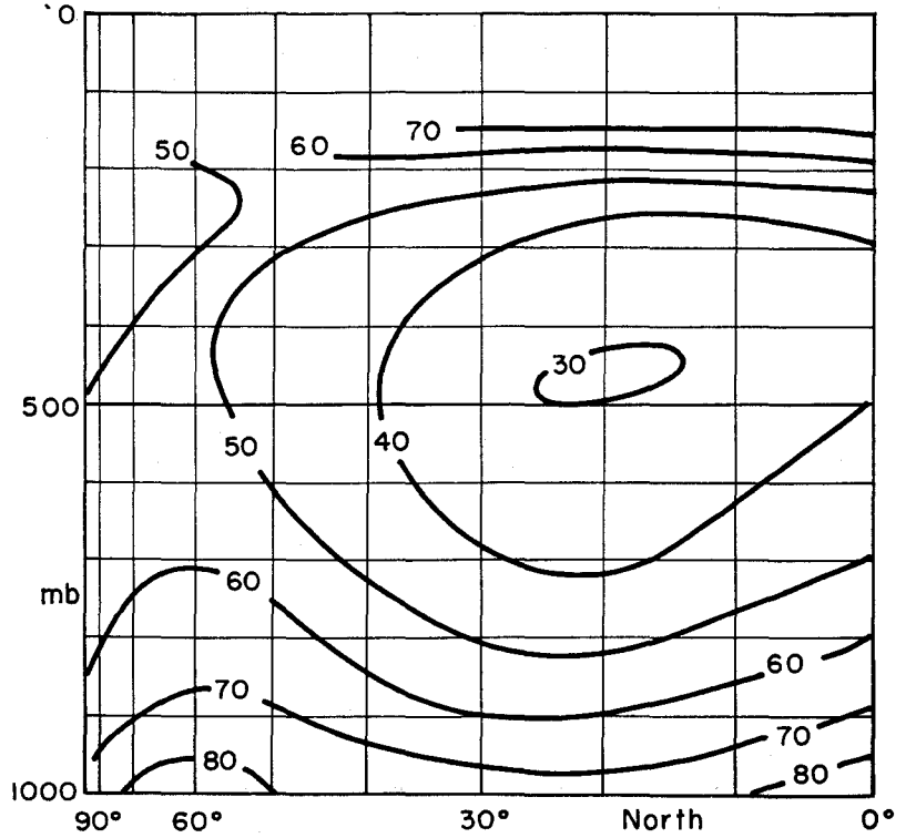
Figure 16. — The time-and-longitude averaged relative humidity [q/q_s] in northern winter as estimated by London (1957). Values are in per cent
