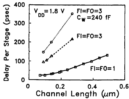
Fig. 11. Measured delay versus channel length for the high-performance L = 0.15 \mu\text{m} CMOS technology ( W_n = W_p/2 = 15 \mu\text{m} ).
