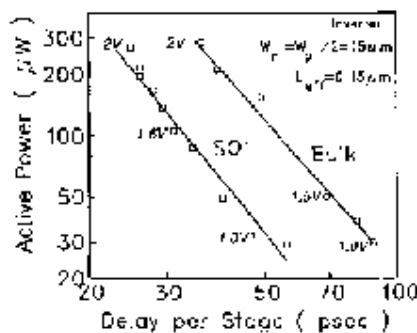
Fig. 15. Measured power versus delay for t_f = 0.15 \mu\text{m} SOI and bulk CMOS with varying voltage.
