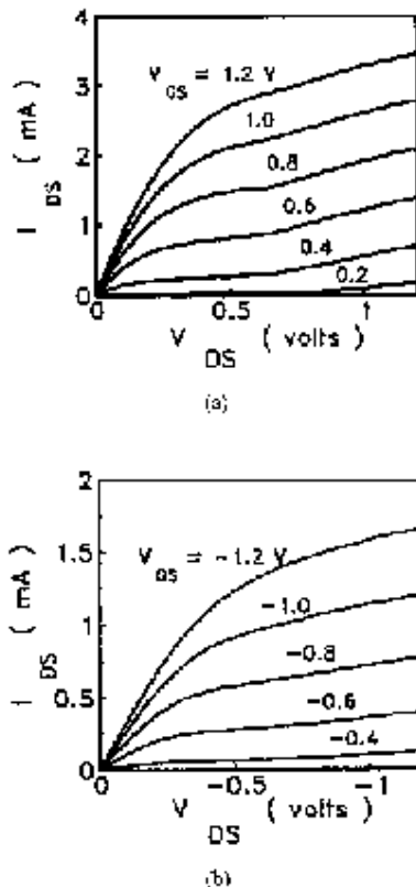
Fig. 14. Device characteristics of 0.1 \mu\text{m} CMOS on SOI ( t_f = 10 \mu\text{m} ). (a) nPEL, (b) pPEL.
