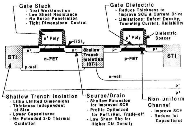
Fig. 8. Key technology elements for deep-submicron CMOS.
