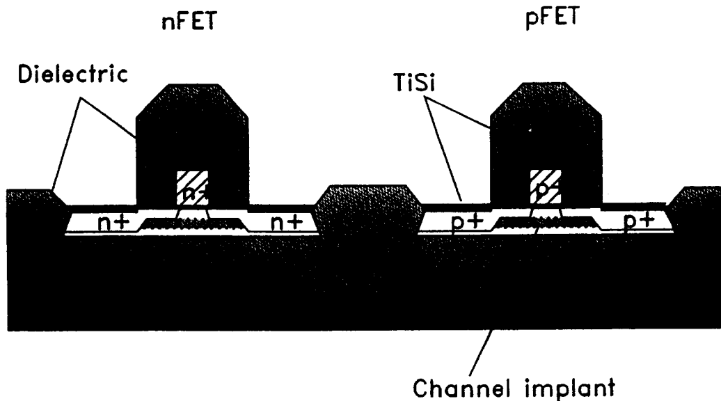
Fig. 13. 0.1 \mu\text{m} CMOS on SOI schematic cross section.
