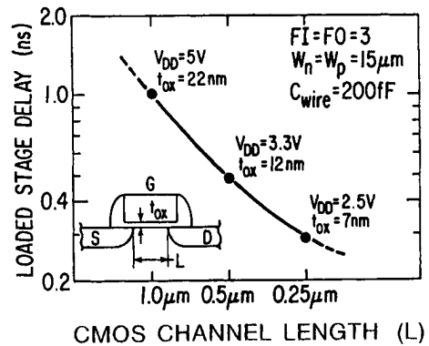
Fig. 2. Scaling of high-performance CMOS technology.
