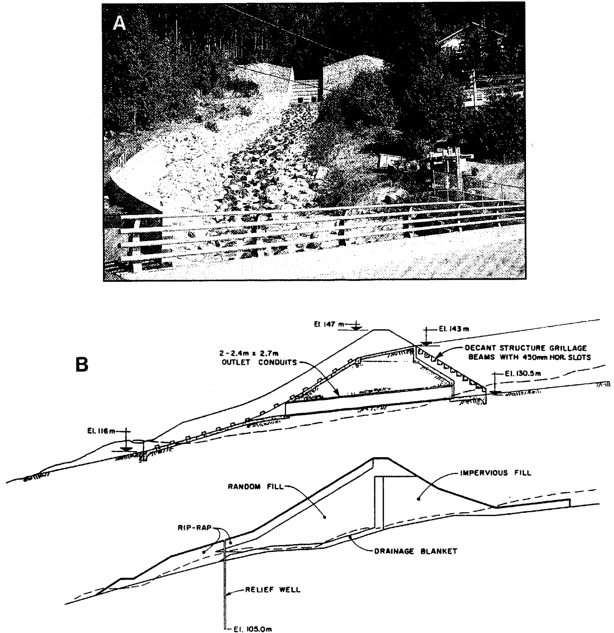
Figure 39. Debris flow retention dam at Harvey Creek, Lions Bay, Howe Sound. A) View upstream; GSC 1994-709K B) Structural cross-section (after Hung and Skermer, (1992) from a sketch drawing by Ker Priestman Associates).
