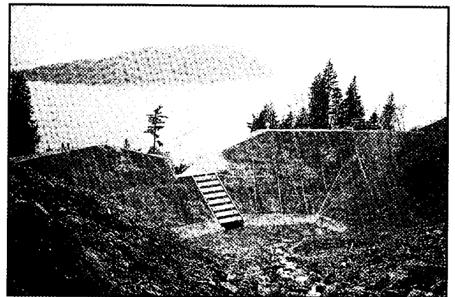
Figure 38. Debris flow retention structure on Charles Creek, Howe Sound constructed in the mid-1980s; view downstream. GSC 1991-298
