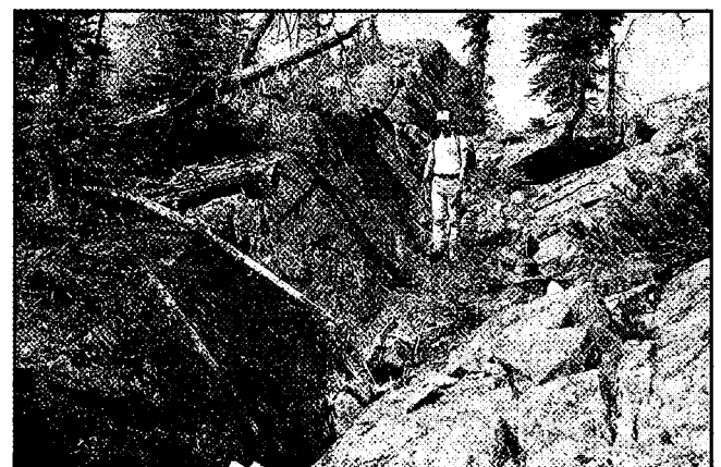
Figure 16. Antislope scarp formed by toppling on southern margin of Mystery Creek rock avalanche. Downslope is to the left. GSC 1994-709E
