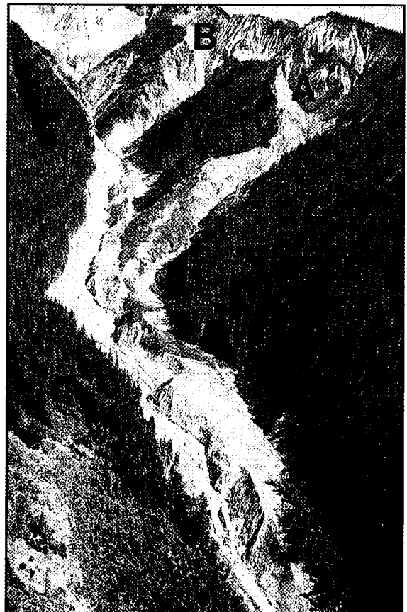
Figure 32. Aerial view of historic debris avalanches in Turbid Creek on the western slopes of Mount Cayley volcano; "A" is the source of the 1963 debris avalanche and "B" is the source of the 1984 event. Both landslides involved initial failure in Pleistocene pyroclastic rocks. This photograph, taken in 1985, shows the swath cut through the tree cover by the 1984 debris avalanche. GSC 204857-F
