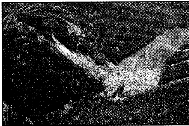
Figure 17. Landslide dammed lake in the Nahatlatch River watershed. The rock avalanche occurred in plutonic rocks. GSC 1992-0815
