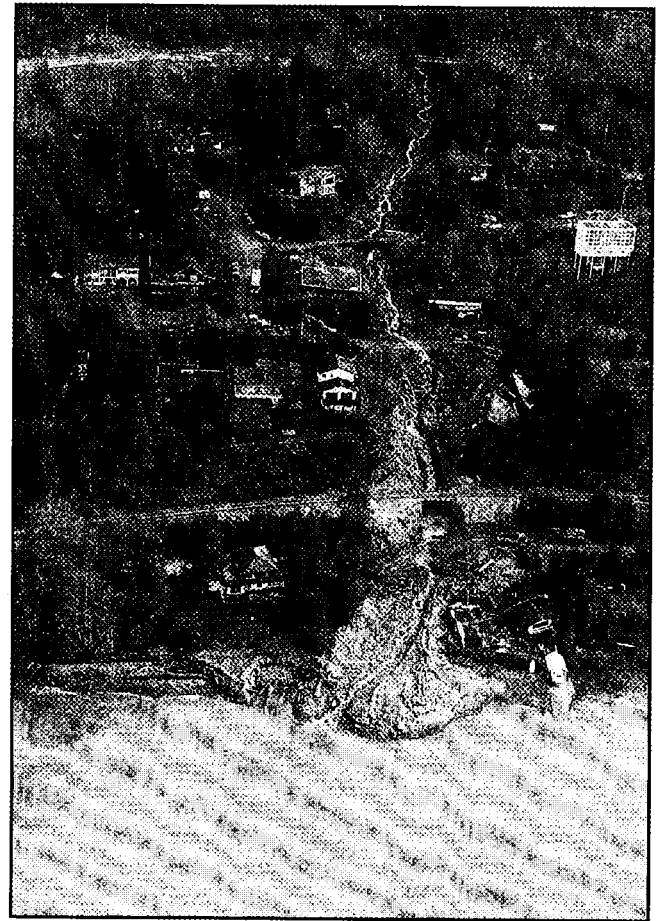
Figure 37. Alberta Creek debris flow, Lions Bay, which occurred on February 11, 1983. Note damaged buildings and bridges (photo courtesy of British Columbia Ministry of Highways and Communications).
