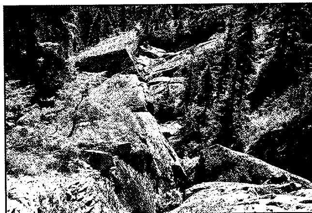
Figure 21. Displaced rock masses resulting from mountain slope deformation, Mt. Breakenridge, Harrison Lake. GSC 1994-709G
