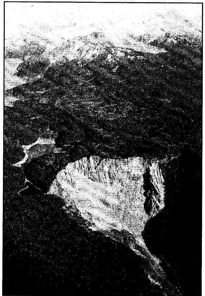
Figure 26. Aerial view of The Barrier , a steep rock face formed by the successive failure of the margin of the Clinker Peak lava flow, the most recent failure being the 1855-56 rock avalanche. Clinker Peak is visible as the obvious source of the lava flow. Mount Garibaldi is visible in right background. GSC 1991-300
