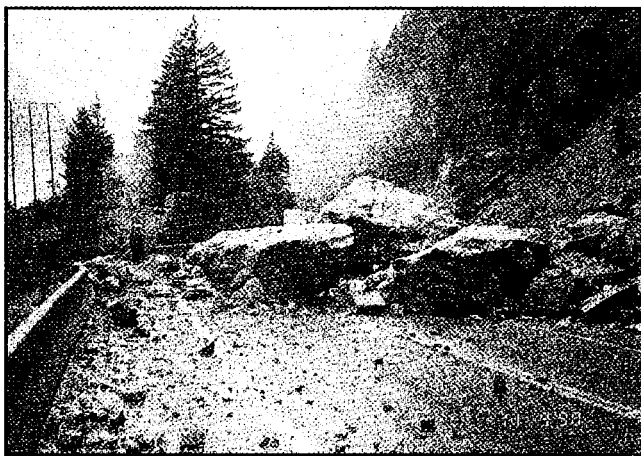
Figure 4. Rockfall on Trans-Canada Highway, Fraser Canyon, near Yale (courtesy of D. Wyllie).
