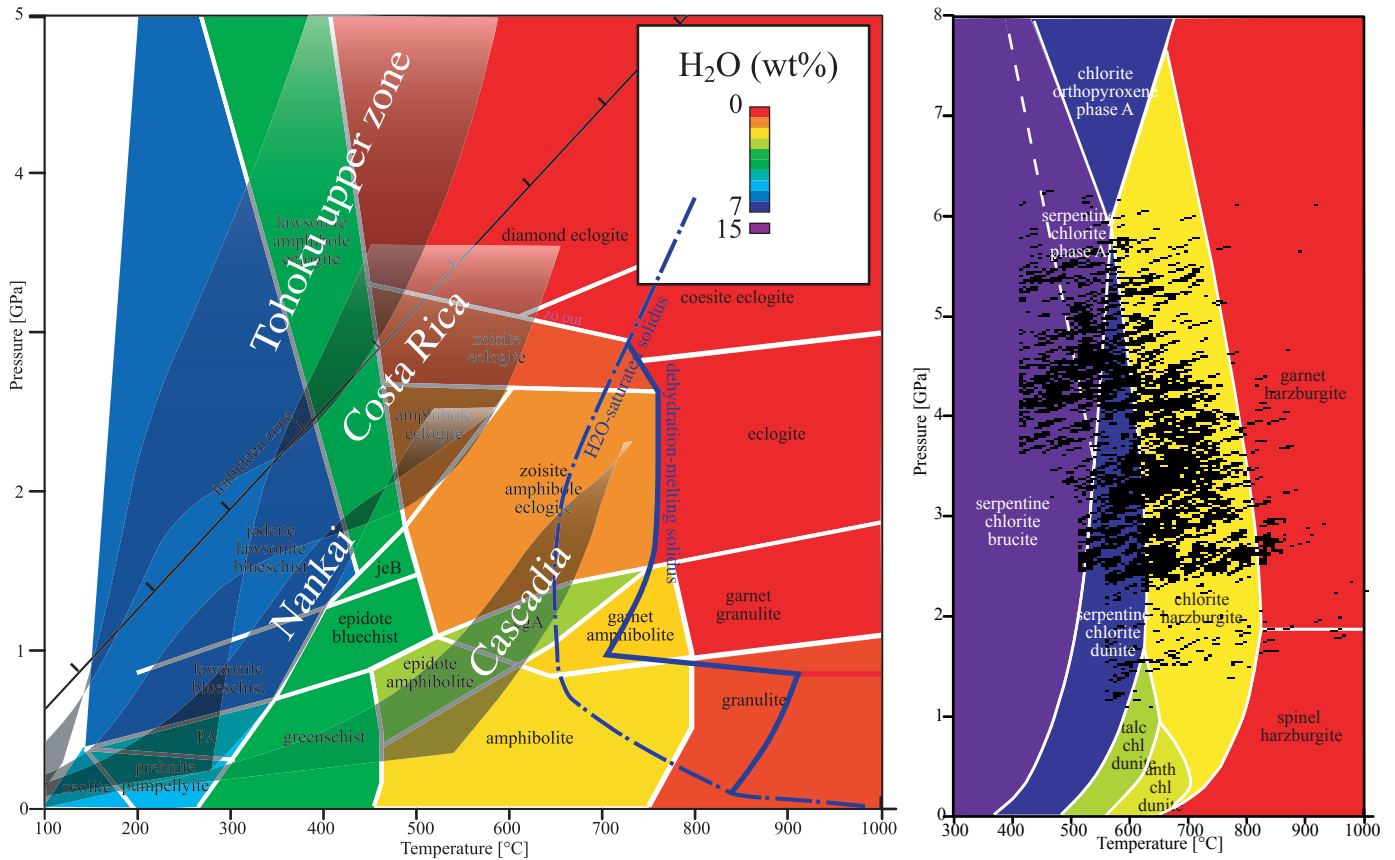
Figure 7. (a) Metamorphic facies and maximum H 2 O contents for mid-ocean-ridge basalt [Hacker et al., 2003] and slab crust PT regimes corresponding to depths of intermediate-depth earthquakes. (b) Metamorphic facies and H 2 O contents for harzburgite [Hacker et al., 2003] and intermediate-depth earthquakes in the lower seismic zone beneath Tohoku. PA, prehnite-actinolite; eA, epidote amphibolite; eB, epidote blueschist; jeB, jadeite-epidote blueschist.
