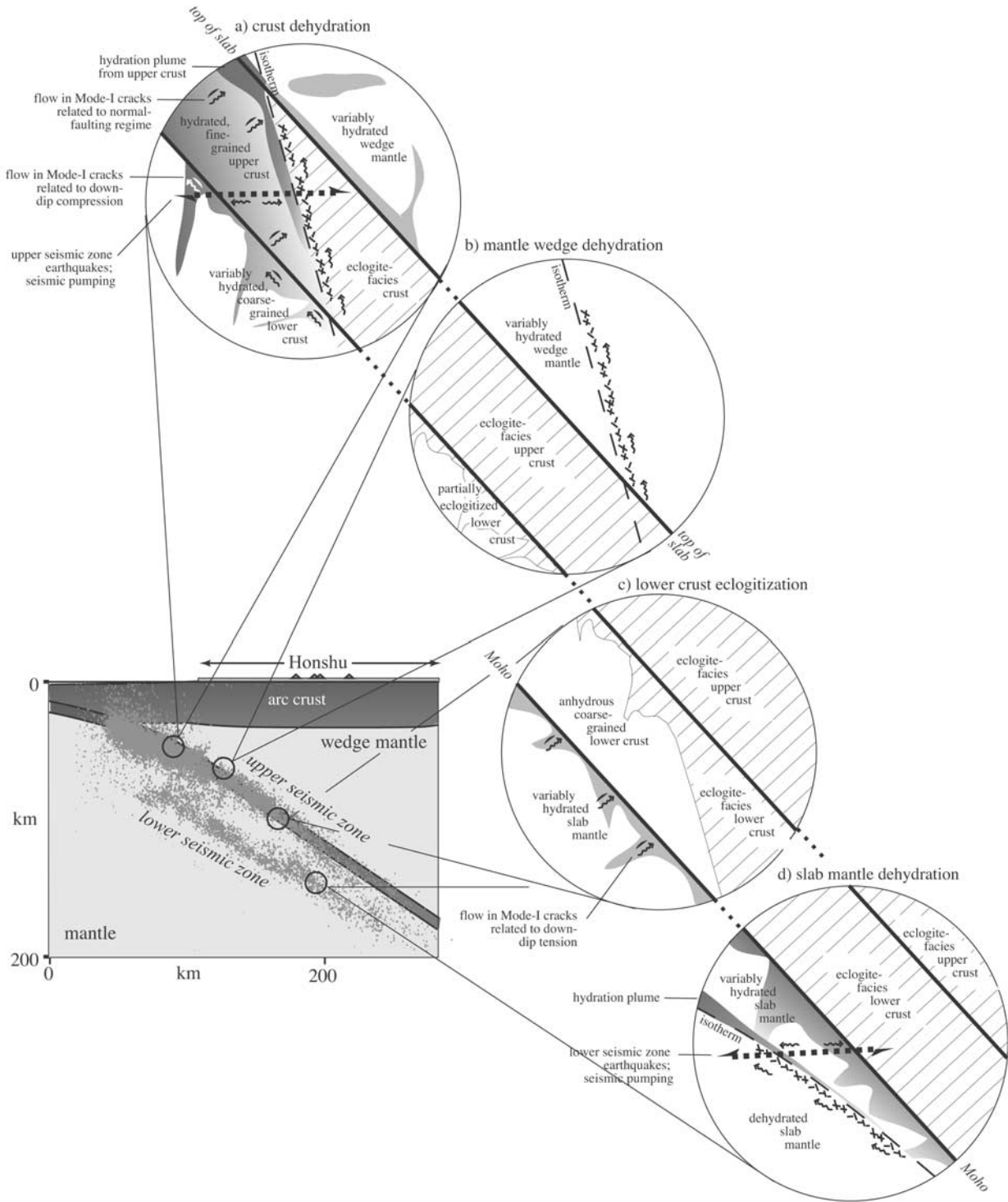
Figure 9. Model for fluid flow in subducting slabs. Upper crust is assumed to be completely hydrated. Mantle and lower crust are assumed to be incompletely hydrated. Depths >70 km where the uppermost earthquakes are normal faulting events. Isotherm shown applies to depth shallower than onset of influence of wedge convection; at deeper levels, coldest part of slab lies 5–20 km beneath the top of the slab. Large dashed arrows indicate earthquakes; small arrows show fluid flow; and crosses indicate reaction zones with microearthquakes, densification, and high permeability. Gray scale shows schematic H 2 O content.
