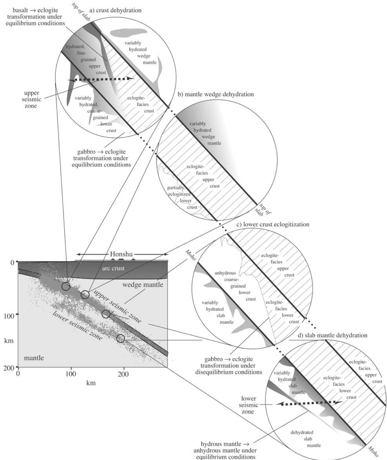
Figure 1. Schematic (not to scale) illustration of subducting crust, showing transformation from hydrated basalt and gabbro → eclogite under equilibrium conditions and kinetically overstepped transformation from anhydrous gabbro → eclogite. No horizontal or vertical scale is implied. In reality, the boundary between upper and lower crust is not sharp, the transformation from basalt or gabbro → eclogite involves many intermediate mineralogical changes, and grain size and hydration state are variable throughout the crust. The subduction zone cross section from Tohoku (true scale) shows a double seismic zone (data of Igarashi et al. [2001]).
