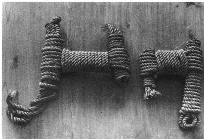
135 Just two of the dozens of different knots that held together the various sections of the Royal Ship – and that, reconstructed in modern rope, continue to hold her together today.
