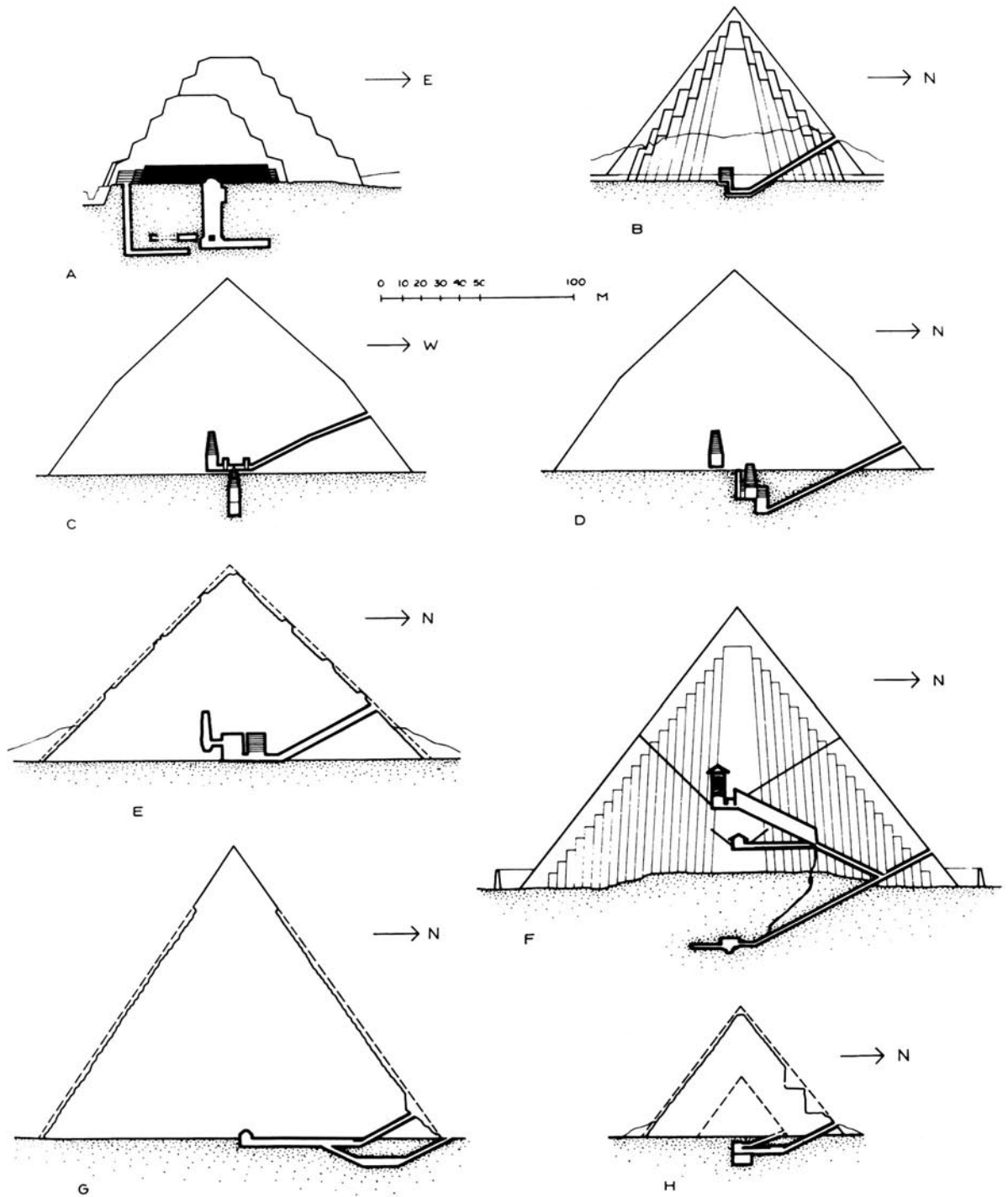
16 The most important Old Kingdom pyramids shown in section with their entrances and burial chambers. A, the Step Pyramid of Zoser at Saqqara; B, the now-ruined pyramid of Meidum; C, the western, and D, the northern entrances to Sneferu's Bent Pyramid at Dahshur; E, the Red or Northern Pyramid of Sneferu at Dahshur; F, the Great Pyramid of Cheops at Giza; G, Chephren's pyramid at Giza; H, the pyramid of Mycerinus at Giza.
