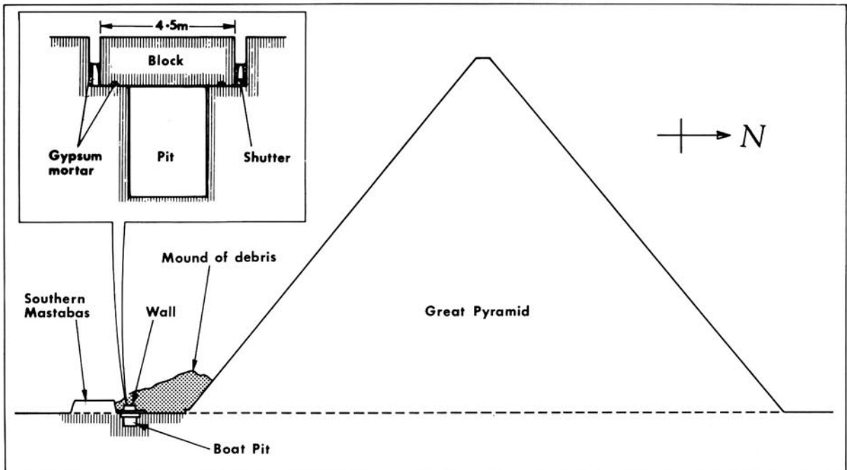
26 Section through the Great Pyramid, showing the mound of debris that covered the two south-face boat-pits before their discovery in 1954, and, in the inset, the pit that contained the Royal Ship, sealed by great limestone blocks with shutters.
