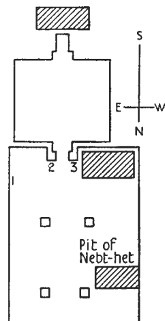
MEIR. Tomb B 3. Senbi. From KAMAL in Ann. Serv. xi, p. 10, fig. 1.
