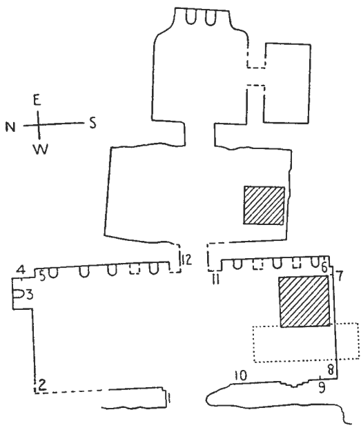
Tomb 3. Meru, called Bebi. From DAVIES, pl. xviii.
