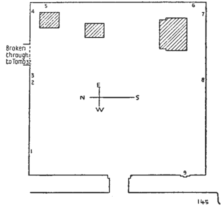
Tomb 33. Bağt II. From NEWBERRY and GRIFFITH, Beni Hasan , ii, pl. xxxiv.
