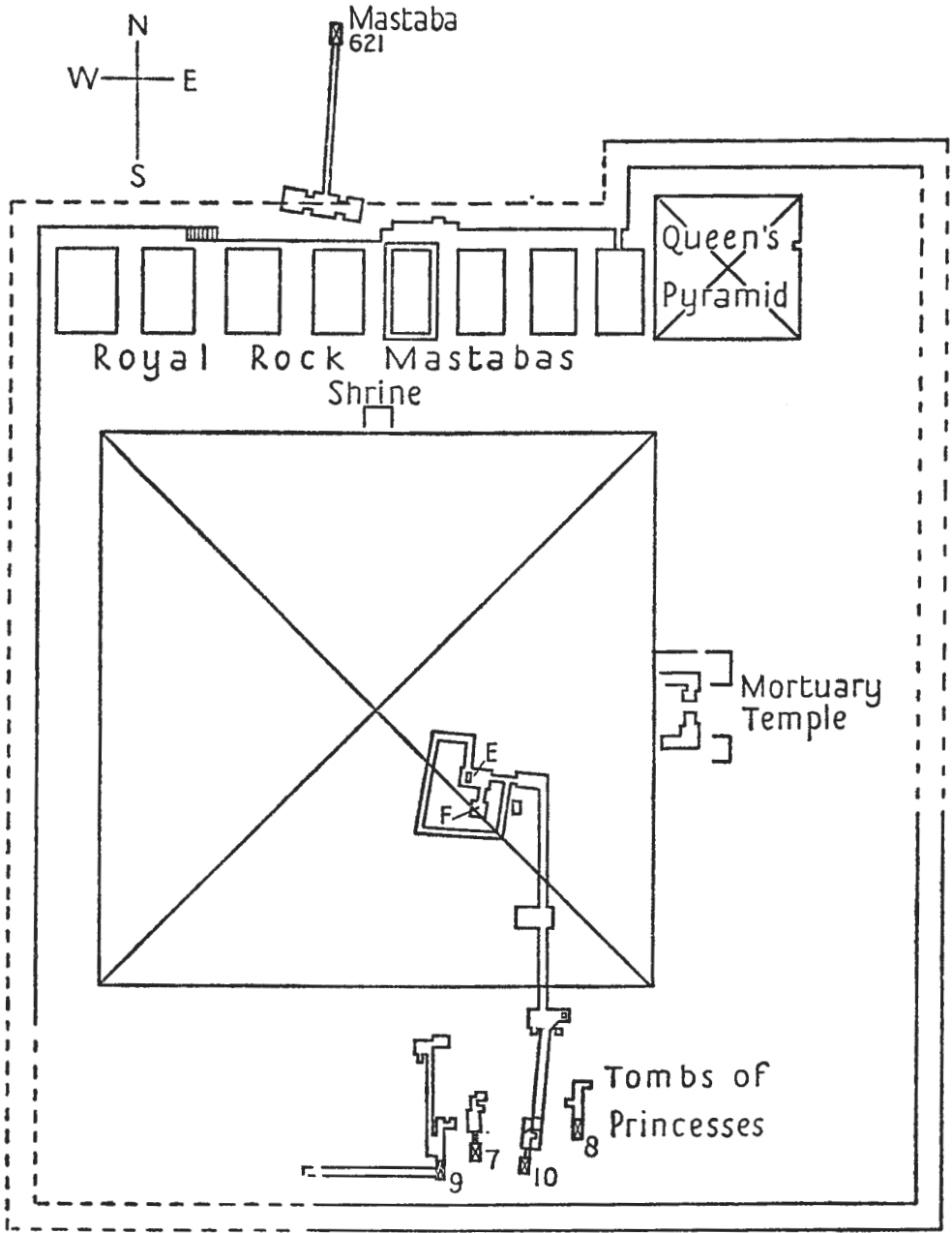
EL-LÂHÛN. PYRAMID. SESOSTRIS II. From PETRIE, BRUNTON and MURRAY, Lahun , ii, pl. viii.
