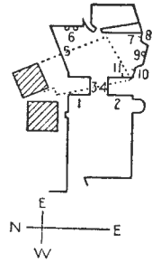
QUSEIR EL-'AMARNA. Khuenekh. From QUIBELL in Ann. Serv. iii, p. 254, fig. 1.
