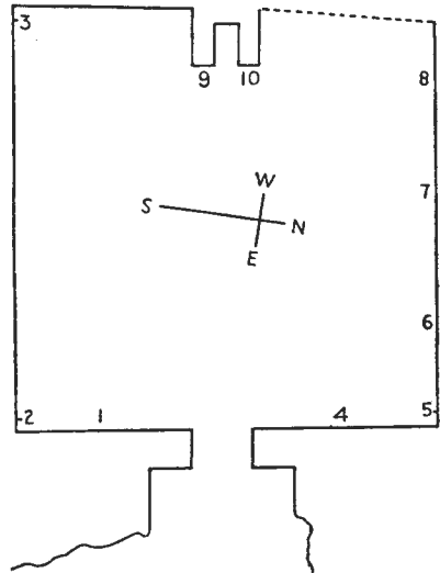
MEIR. Tomb B 1. Senbi. From BLACKMAN, The Rock Tombs of Meir , i, pl. i.
