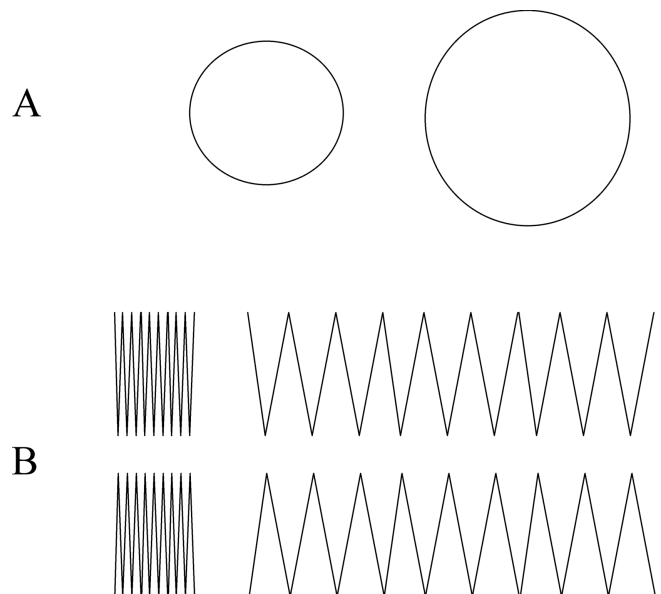
Fig. 5. Two of the four possible shapes proposed by Gil et al. (1979) by means of which the architecture of the alveolus can be modified with respiratory movements. A: balloonlike increase/decrease in alveolar size. B: crumpling of the alveolar surface, similar to the folding of an accordion.
