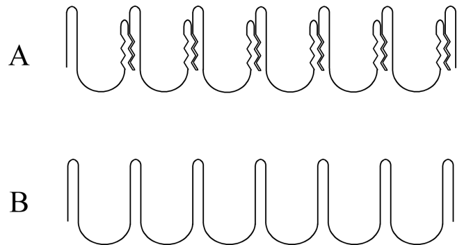
Fig. 3. Schematic representation of alveolar recruitment. At the beginning of inspiration the lung is partially swollen. Microscopically, there are more closed than open (derecruited than recruited) alveoli. A: At the beginning of inspiration the walls of the closed alveoli are stuck to one another. B: When the transpulmonary pressure is increased, the lung volume increases and the alveoli are recruited by unfolding their walls.
