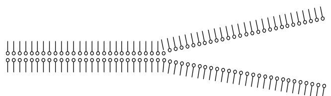
Fig. 9. Schematic representation of two adhered membranes that become unstuck at the right end. This mechanism is similar to what occurs with velcro: the energy that is used to unstuck the two velcro surfaces is not recovered when they are restuck.
