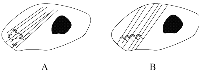
Fig. 8. Schematic representation of the cytoskeleton actin filaments. A: non-organized filaments. B: filaments aligned by the application of forces. The alignment of actin filaments consumes energy.
