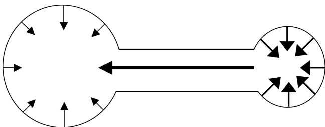
Fig. 6. Schematic representation of the consequence of Laplace's Law. When two bubbles of different sizes are connected, the bubble with the greatest surface tension, the small bubble, deflates to the benefit of the large bubble.
