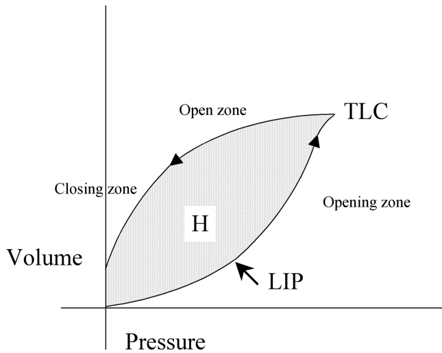
Fig. 1. Representation of the pressure-volume curve. The ascending part applies to inspiration and the descending part to expiration. The dotted area is the hysteresis area. TLC: Total Lung Capacity. H: Hysteresis area. LIP: Lower Inflexion Point. Beginning of the opening zone. Opening zone: first part of inspiration; the peripheral airways are opened exponentially. Open zone: second part of expiration, the peripheral airways remain open. Closing zone: third part of expiration; the peripheral airways close.
