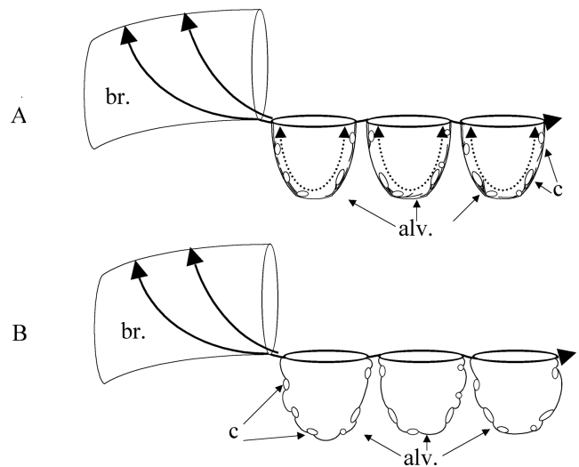
Fig. 7. Schematic representation of the network that spreads around the bronchi (br) and vessels and surrounds the mouths of the alveoli (arrows with continuous line). A: When the lung slackens, the tension of this network opens the mouths of the alveoli; the surface tension (arrows with dotted lines inside the alveoli) tenses the alveolar wall and folds appear in it. B: When the alveolus does not have surface tension, the network tenses the mouths, opening the alveoli. The lack of surface tension makes the alveolar walls flaccid. Wilson and Bachofen (1982). c: capillaries.
