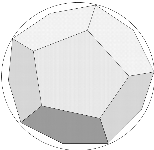
Fig. 4. Model of alveolus with regular dodecahedron shape. When the lung is inflated, the dodecahedron shape becomes spherical.
