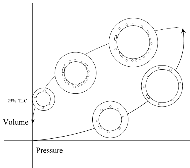
Fig. 10. Schematic representation of bronchial hysteresis. In inspiration, the bronchial lumen increases and decreases when the transpulmonary pressure is raised and dropped. The bronchial lumen is always greater in expiration than in inspiration. In expiration, the bronchial wall increases when the transpulmonary pressure is dropped to 25% of the TLC; from this point on, the bronchial wall decreases. The small circles, which represent epithelial microcirculation, proliferate during expiration, causing the bronchial wall to increase in size.
