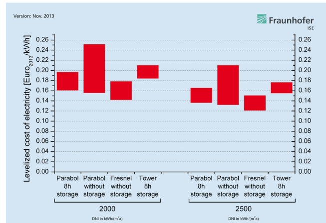
Figure 23: LCOE of CSP plants with a nominal capacity of 100 MW, by plant type and irradiation (DNI in kWh/(m 2 a)) in 2013
