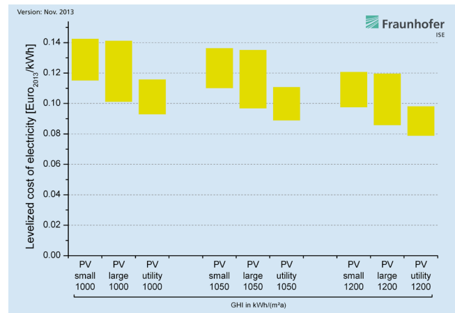
Figure 8: LCOE of PV plants in Germany based on system type and irradiation (GHI in kWh/(m²a)) in 2013.
