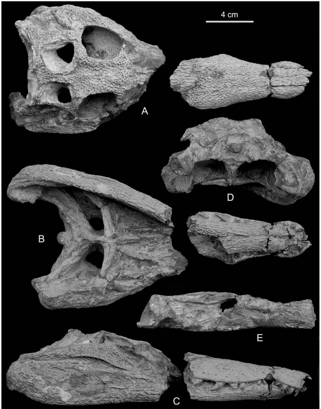
Fig. 1 Skull and lower jaws of Hsisosuchus chowi sp. nov. (ZDM 0146) in dorsal (A), ventral (B), right (C) and posterior (D) views, and posterior portion of left lower jaw in medial view (E)
