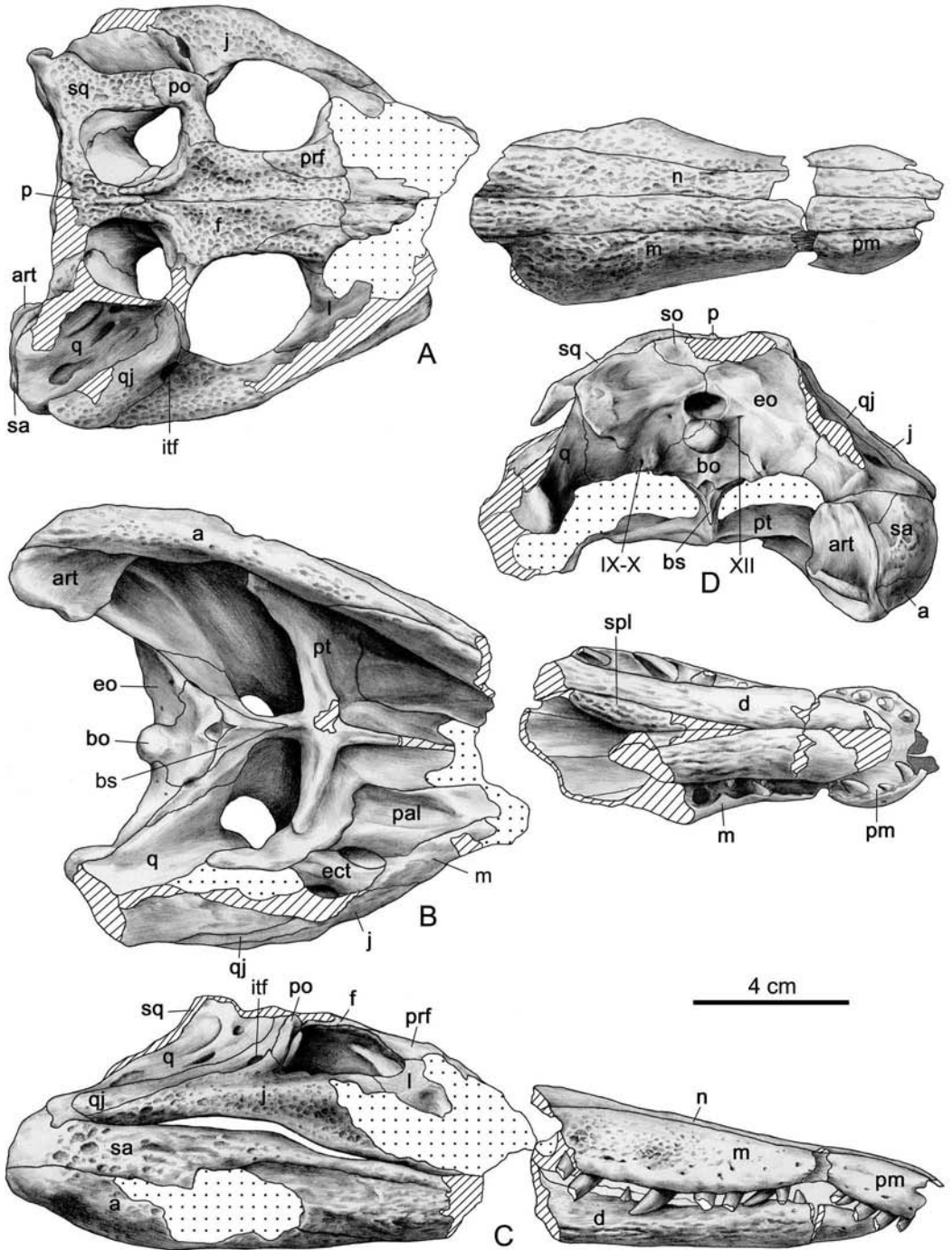
Fig. 2 Drawing of the skull and lower jaws of Hsisosuchus chowi sp. nov. (ZDM 0146) in dorsal (A), ventral (B), right (C) and posterior (D) views
