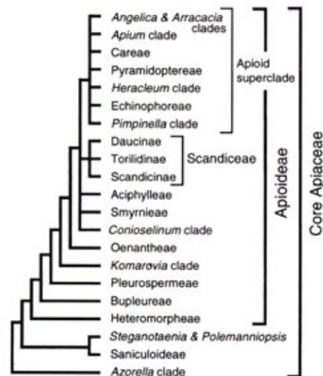
FIG. 5. Summary of relationships among the tribes (Table 2) and informally recognized clades (Table 3) of Apiaceae subfamily Apiioideae as revealed by phylogenetic analyses of molecular data (this study; Downie & Katz-Downie, 1999; Downie et al. , 1998, 2000a,b,c). Not all genera examined to date have been assigned to a particular group (Table 4); many of these genera, however, are contained within the apioid superclade.
