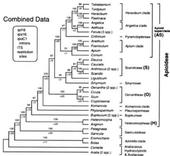
FIG. 3. Single minimal length 3929-step tree derived from maximum parsimony analysis of combined DNA sequence ( rpl16 intron, rps16 intron, rpoC1 intron, ITS) and restriction site data (CI, excluding uninformative characters = 0.482; RI = 0.639). Numbers above nodes are bootstrap estimates for 1000 replicate analyses; numbers below nodes are decay values for trees up to 20 steps longer than those most parsimonious. The Ferula , Anthriscus , Oenanthe , Bupleurum and Aralia species examined in each of the separate analyses were not identical; however, because each group of species is monophyletic (as revealed by our earlier, more comprehensive analyses), data for each genus were combined and treated as a single exemplar. Data for genera not included in any separate analysis were scored as missing data. Complete species names are indicated in Table 5. The bracketed tribes and clades are those listed in Tables 2 and 3; the abbreviations AS, S, O and H are the same as outlined in Fig. 2.
