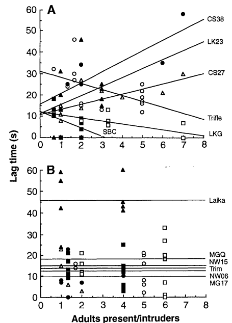
Fig. 1. Lag times of the 12 laggards plotted against the number of adults present on the playback divided by the number of "intruders." Inclusion of both individual intercepts ( F_{1,11,07} = 3.39, P = 0.0006 ) and slopes ( F_{1,11,96} = 2.27, P = 0.016 ) significantly improved the overall model. Two other factors were tested but found not to be significant: the total number of adults in the pride (but not necessarily present) and the number of subadults present. (A) All laggards with nonzero slopes ( P < 0.05 ). Open circles, Trifle; solid circles, CS38; open triangles, CS27; solid triangles, LK23; open squares, LKG; and solid squares, SBC. (B) All laggards with constant lagging times. Open circles, Trim; solid circles, MG17; open triangles, MGQ; solid triangles, Laika; open squares, NW15; and solid squares, NW06.
