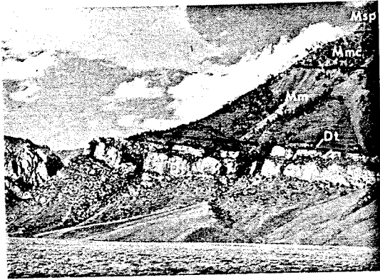
FIG. 20.—Slope-forming argillite, siltite, and minor quartzite of Lower Mississippian Milligen Formation (Mm) of Sandberg and others (1967) in Lost River Range, central Idaho, represents fine-grained flysch in eastern part of foreland trough. Milligen underlain by shaly limestone of upper Upper Devonian Three Forks Formation (Dt) which directly overlies the prominent limestone cliffs of lower Upper Devonian part of the Jefferson Formation (Dj) of carbonate shelf. Milligen overlain by Upper Mississippian slope-forming and cliffy limestone units in upper right (Middle Canyon Formation, Mmc, and Scott Peak Formation, Msp). Photograph by C. A. Sandberg.
