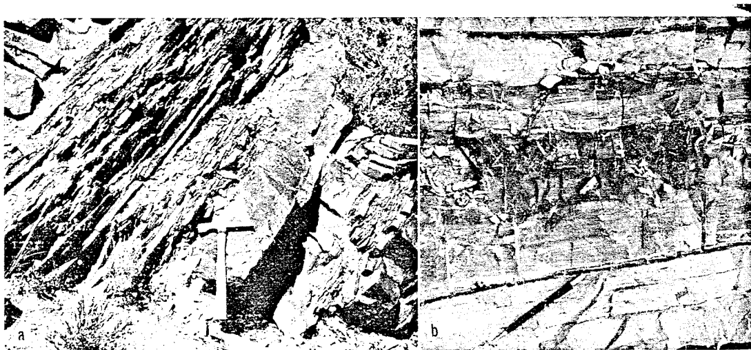
FIG. 5.—Lithology and bedding features of turbidite sequences in fine-grained flysch. a , Interbedded sandstone to coarse-grained siltstone turbidites (ledges) and mudstone interturbidites (recesses) of siliceous basinal flysch in the lower part of the Chainman Shale, Diamond Mountains, central Nevada; hammer is on a sandstone turbidite bed; stratigraphic top is to the right (overturned section). b , Interbedded impure limestone turbidites (dark-colored interval above pencil) and light-colored spicular limestone interturbidites of calcareous flysch in the lower part of the Drummond Mine Limestone, Pioneer Mountains, central Idaho.
