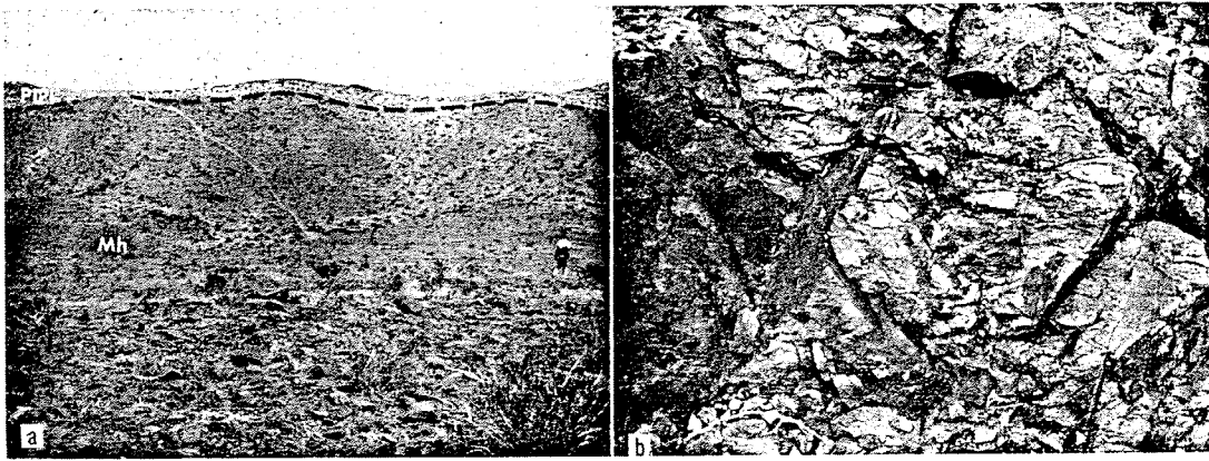
FIG. 3.—Unamed flysch deposits in Shadow Mountains, southwestern Mojave Desert, southern California. a , Metamorphosed dark-colored flysch (mostly hornfels of Mississippian age, Mh) overlain by light-colored limestone (mostly calcite marble of Pennsylvanian and Permian age, P1P1). b , Tectonically stretched quartzite pebbles in a dark-colored conglomeratic quartzite bed within the "schistose rocks" map unit of Troxel and Gundersen (1970).
