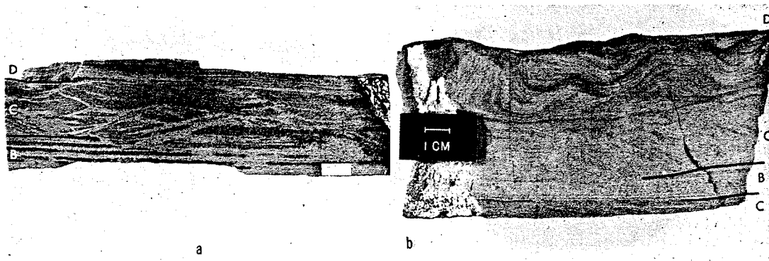
FIG. 8.—Internal structure of distal turbidite beds showing incomplete Bouma sequences. a , Polished slab of sandstone turbidite showing horizontal parallel laminae of division B, current ripple laminae of division C, and upper parallel laminae of division D; specimen from unit C of Eleana Formation, Belted Range, south-central Nevada. b , Specimen of amalgamated limy sandstone-siltstone turbidite sequences showing current ripple laminae of division C directly overlain by horizontal parallel laminae of division B, current ripple laminae, wavy and convoluted laminae of division C, and thin upper parallel laminae of division D; specimen from base of Scorpion Mountain Formation, Pioneer Mountains, central Idaho.
