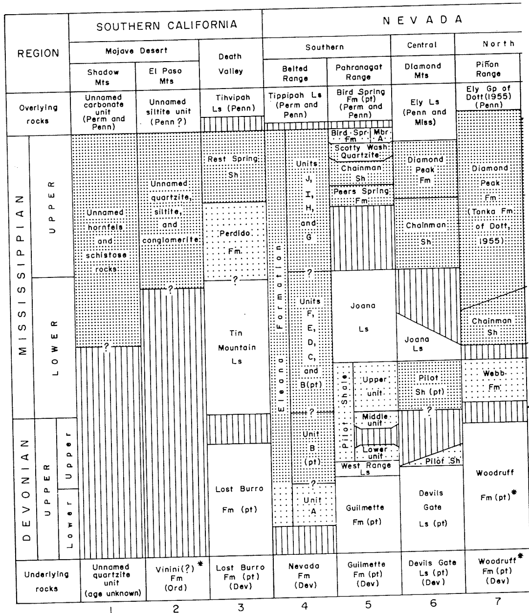
FIG. 2.—Generalized chart showing stratigraphic position and some local names applied to Antler flysch (stippled) and associated rocks in the western United States. Hatching indicates strata absent because of nondeposition or erosion. Compact stippling indicates that strata consist mostly of orogenic sediments; diffuse stippling indicates that strata consist of either minor orogenic sediments or mostly of reworked orogenic sediments. Asterisk (*) indicates allochthonous eugeosynclinal- and transitional-facies rocks in Roberts Mountains Allochthon. Sources of data: 1. Troxel and Gundersen (1970); F. G. Poole and J. H. Stewart (unpub. data); 2. Poole (unpub. data); 3. McAllister (1952); Mackenzie Gordon, Jr., and Poole (unpub. data); 4. Poole, Houser, and Orkild (1961); Poole, Orkild, Gordon, and Duncan (1965); Gordon and Poole (1968); Ekren, Anderson, Rogers, and Noble (1971); Poole and Gordon (unpub. data); 5. Reso (1963); Sandberg
