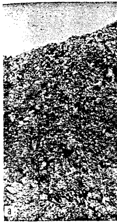
FIG. 6.—Lithology and bedding features of turbidite sequences in coarse-grained flysch. a , Massive conglomerate in the lower part of a flow conglomerate channel in the Antler flysch, overlain by scouring massive sandstone in the upper part of the channel fill.
