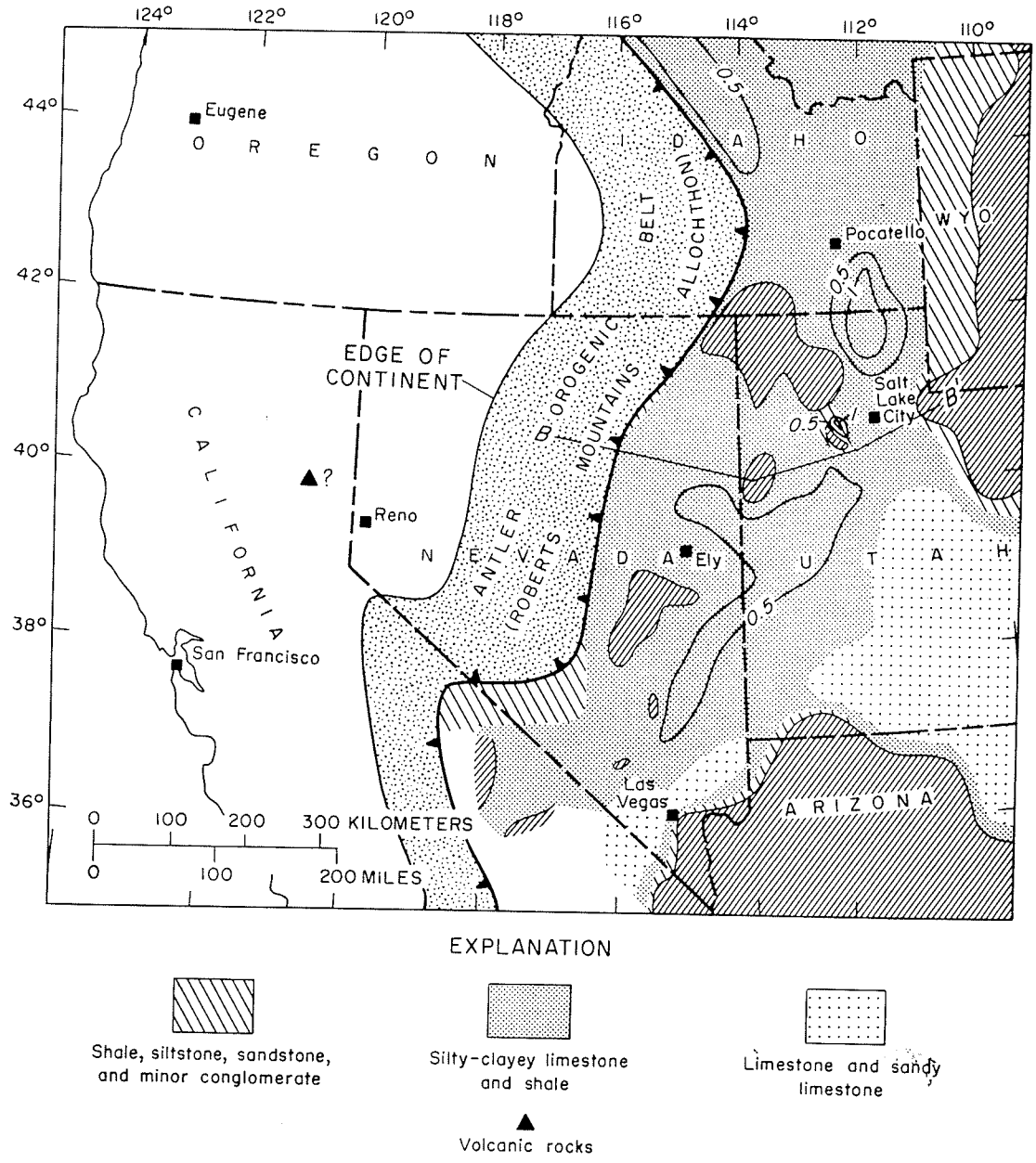
FIG. 15.—Isopach and facies map of upper Upper Devonian rocks (partly restored). Emergent areas shown by compact hatching. Isopachs in thousands of feet. Thickness and facies west of continental edge not shown owing to insufficient stratigraphic data. Roberts Mountains Allochthon emplaced near end of late Late Devonian time. Cross section BB' shown by figure 25b.
