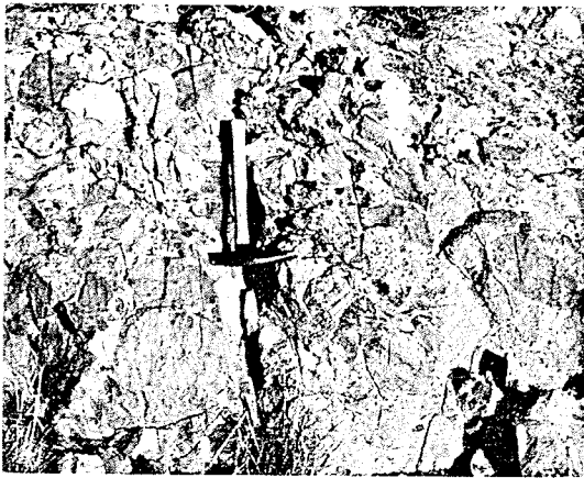
FIG. 16.—Upper Upper Devonian carbonate-clast conglomerate in Stansbury Formation, Stansbury Mountains, northwestern Utah, represents coarse detritus from local Stansbury uplift at outer edge of cratonic platform.
