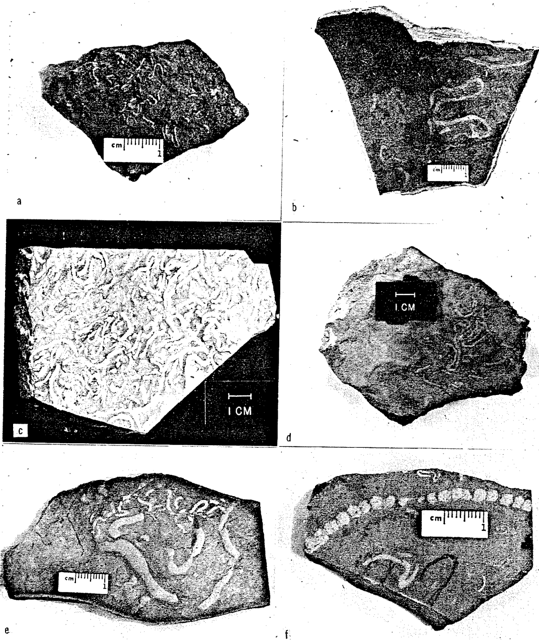
FIG. 10.—Indigenous meandering trails of Nereites community in hemipelagic mudstone and siltstone (division E of Bouma sequence) between sandstone turbidites. a , Meandering trails in Muldoon Canyon Formation, Pioneer Mountains, central Idaho. b , Meandering trails and small fragments of macerated plant debris in Milligen Formation of Sandberg and others (1967), Lost River Range, central Idaho. c , Meandering trails in Chainman Formation, Pequop Mountains, northeastern Nevada. d , Meandering trails in unit D of Eleana Formation, Belted Range, south-central Nevada. e , Narrow and wide meandering trails in Diamond Peak Formation, Diamond Mountains, central Nevada. f , Meandering trails and segmented trail ( Scalartuba? ) in basal beds of Scorpion Mountain Formation, Pioneer Mountains, central Idaho.
