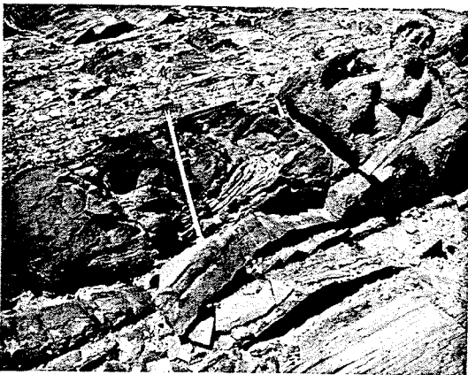
FIG. 17.—Sandy limestone turbidite (ledge 1 m thick in center of picture) that is conglomeratic and contains flute casts, displaced shallow-marine fossils, and slump folds within lower unit of the Pilot Shale in Confusion Range, Utah, near Nevada State line. Note large slump fold behind tape.
