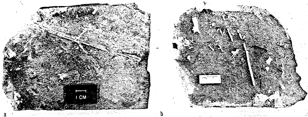
FIG. 11.—Displaced land plants in marine siltstone of Milligen Formation of Sandberg and others (1967), Lost River Range, central Idaho. a , Bedding surface showing relatively large stem with some branch attachments and small fragments of macerated plant debris. b , Bedding surface showing abraded stems with preferred orientation and macerated plant debris.
