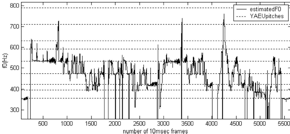
Fig. 3. F0 data in a recording of Tanburi Cemil Bey (Vol 1, Track 2—‘Çeçen kızı’ ( maqam Hüseyini )) plotted together with YAEU tone grid represented as dashed lines.
