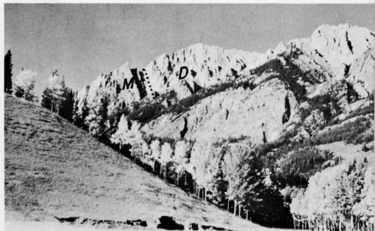
Figure 22. The Sawtooth Range. The sawtooth ridges were formed by water percolating along fractures or joints in the steeply dipping Mississippian (M) and Devonian (D) limestone strata.
