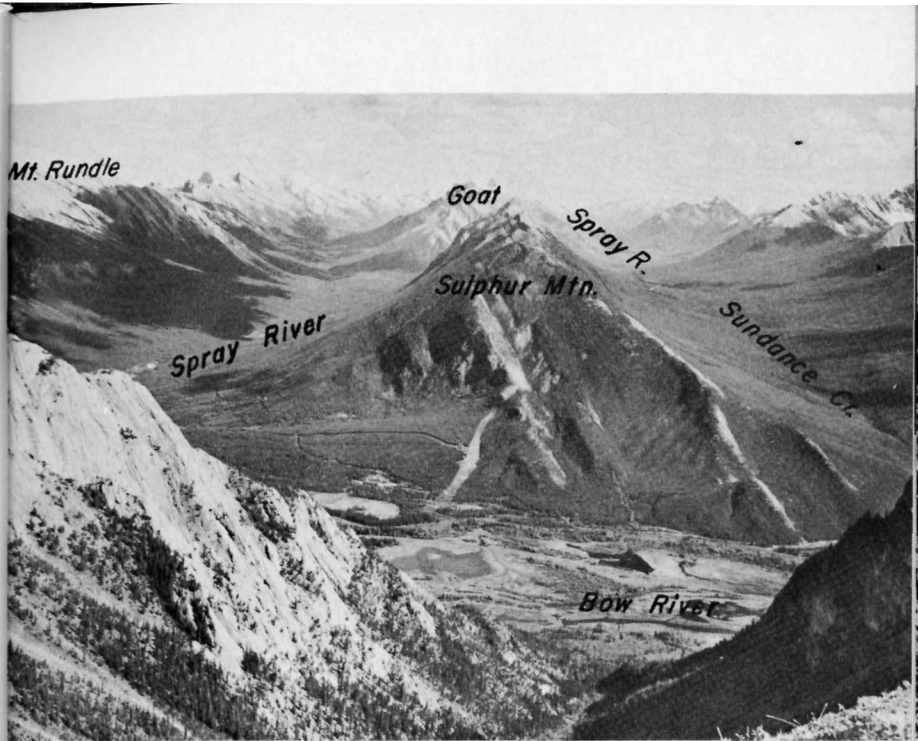
Figure 25. Sulphur Mountain, Spray and Sundance valleys from Mount Norquay with Bow River valley in the foreground. These valleys have a history of stream piracy. The Bow River, as the main stream, cut its valley most rapidly and the waters in the valley east of Sulphur Mountain (the present Spray River) flowed into it. The valley west of Sulphur Mountain (Sundance Creek, now), where once flowed a large stream, the early Spray, was choked by glacial drift. As a result the stream in the lower Spray River valley cut the gap between Sulphur and Goat ranges and captured the headwaters of the Spray, deflecting the main stream to the east of Sulphur Mountain. Hence we find little Sundance Creek occupying the broad valley west of Sulphur Mountain.
