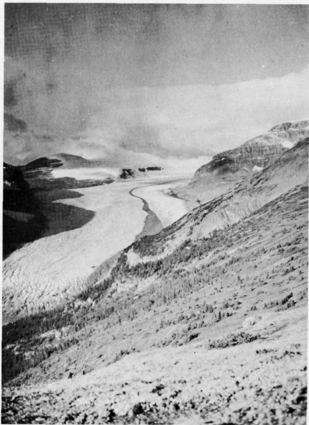
Figure 14. Saskatchewan Glacier. This is a typical valley glacier, flowing eastward from the Columbia Icefield on the Continental Divide. This glacier forms the headwaters of the North Saskatchewan River which flows from here to Nelson River in northern Manitoba. The dark line winding down the middle of the glacier is moraine.
