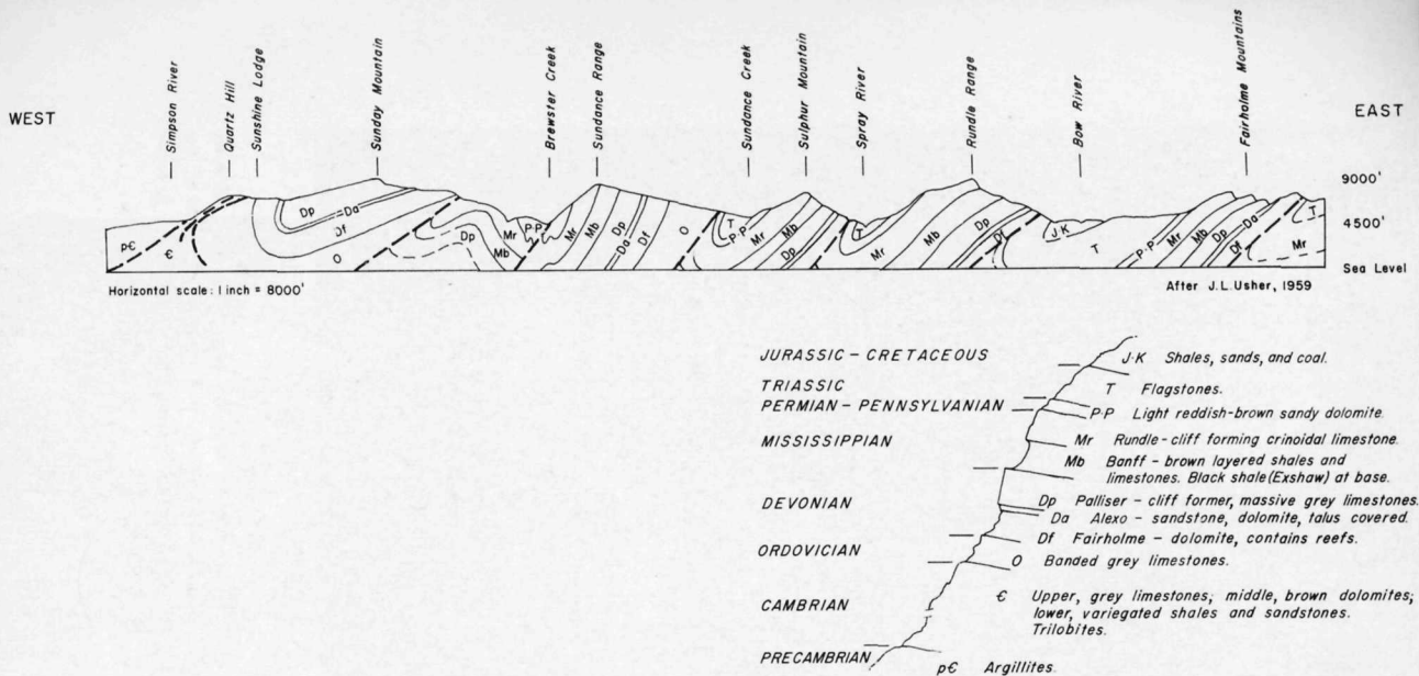
Figure 27. Diagrammatic section across the mountains from the Continental Divide at the headwaters of west flowing Simpson River and the east entrance to Banff National Park. Mount Rundle, as seen from the Hoodoos Viewpoint illustrates the alternating limestone cliffs and layered shale sequence typical of the Front Ranges of the Rocky Mountains east of Mount Eisenhower.
