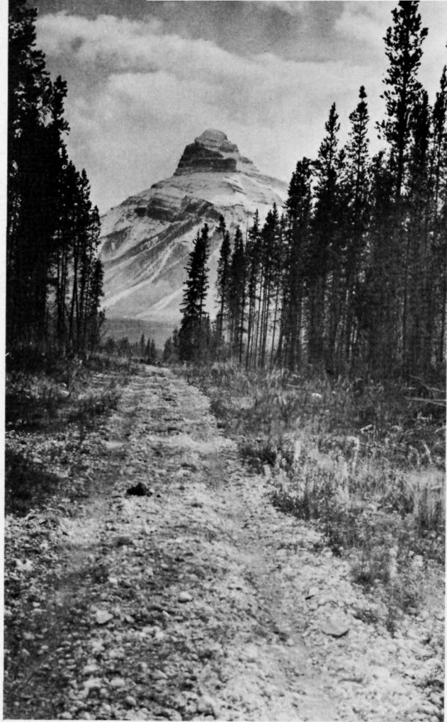
Figure 28. Pilot Mountain may be seen for a long distance up Bow River valley. It is capped by cliffs of the Mississippian Rundle formation that rest on layered Banff shales.
