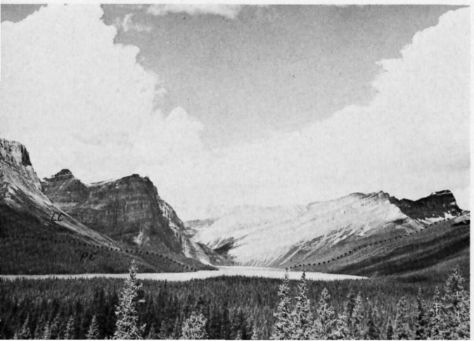
Figure 32. Hector Lake, west of the Banff-Jasper highway, is fed by glaciers along the Continental Divide. The cliffs are Middle Cambrian limestones dipping west away from the centre of Bow anticline.
