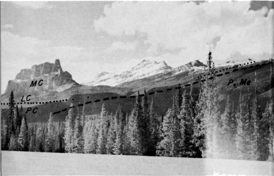
Figure 9. Mount Eisenhower as it appears today. Above the Castle Mountain thrust are Precambrian (PC) and Cambrian (LC and MC) rocks that have ridden up over late Palaeozoic (P) and Mesozoic (Me) rocks.
