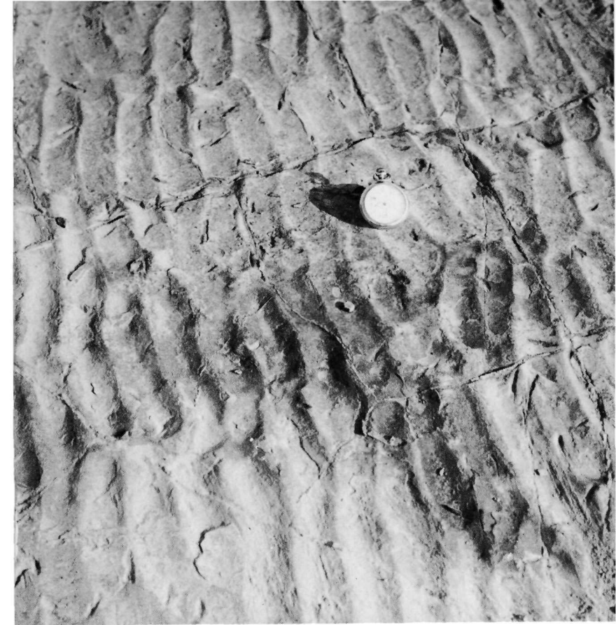
Figure 10. Ripple-marks preserved on a rock surface are like those caused by waves on the bottoms of lakes and along the seashore today.
