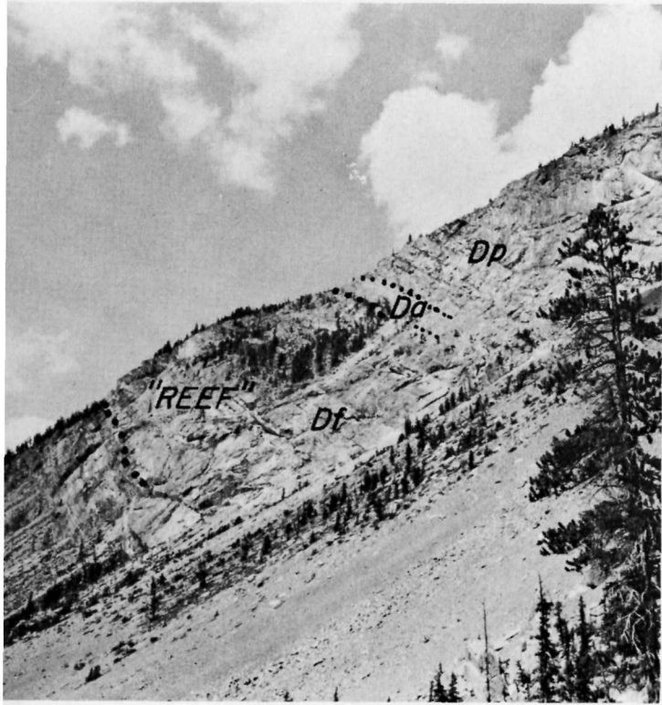
Figure 7. A massive Devonian white dolomite reef in the 'big hill', Sunwapta Pass, Banff-Jasper highway. This is the same type of structure as that from which oil is produced at Leduc, Redwater, Golden Spike and other fields in Alberta. Dp - Palliser limestone; Da - Alexo; Df - Fairholme.
