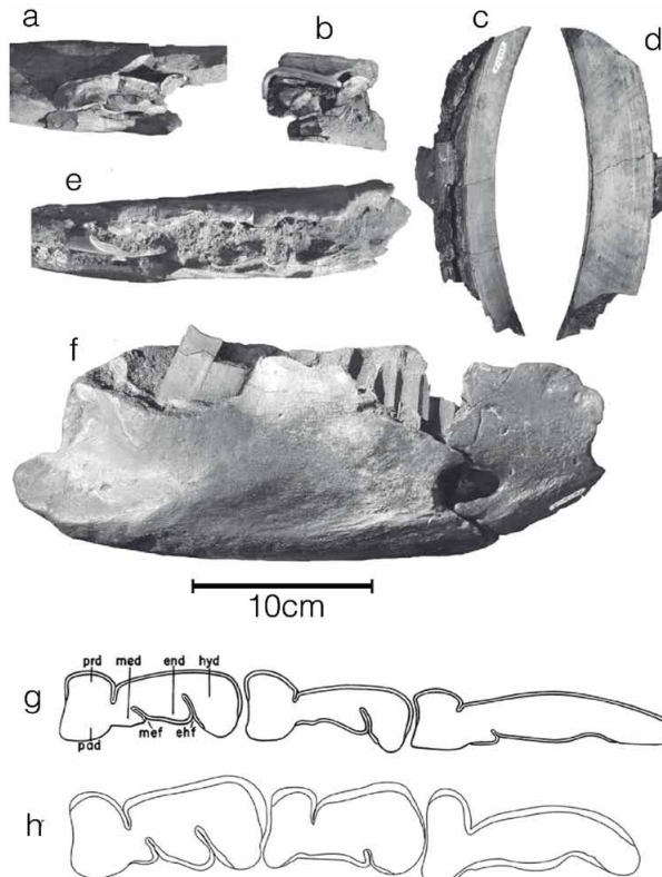
Figure 2. Teeth and lower jaw remains of Mixotoxodon larensis from Mene de Inciarte. a: thirteenth lower molar (MBLUZ-P-3912); b: first lower molar (MBLUZ-P-5896); c: lingual and D: labial view of the thirteenth lower incisor (MBLUZ-P-2335); e: occlusal view of the molar series of Mixotoxodon larensis (MBLUZ-P-3990); f: lower jaw (composed), (MBLUZ-P-4172 and MBLUZ-P-3990); g: oclusal outline of lower molar series of Mixotoxodon larensis from San Miguel after Van Frank 1954; and h, Mene de Inciarte (MBLUZ-P-3990). Abbreviations: ehf: ento-hypoconid fold, end: entoconid, hyp: hypoconid, med: metaconid, mef: meta-entoconid fold, pad: paraconid, prd: protoconid.
