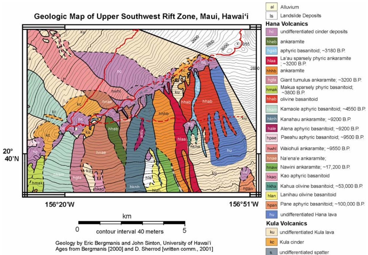
Figure 33. Geologic map of the upper southwest rift zone.
