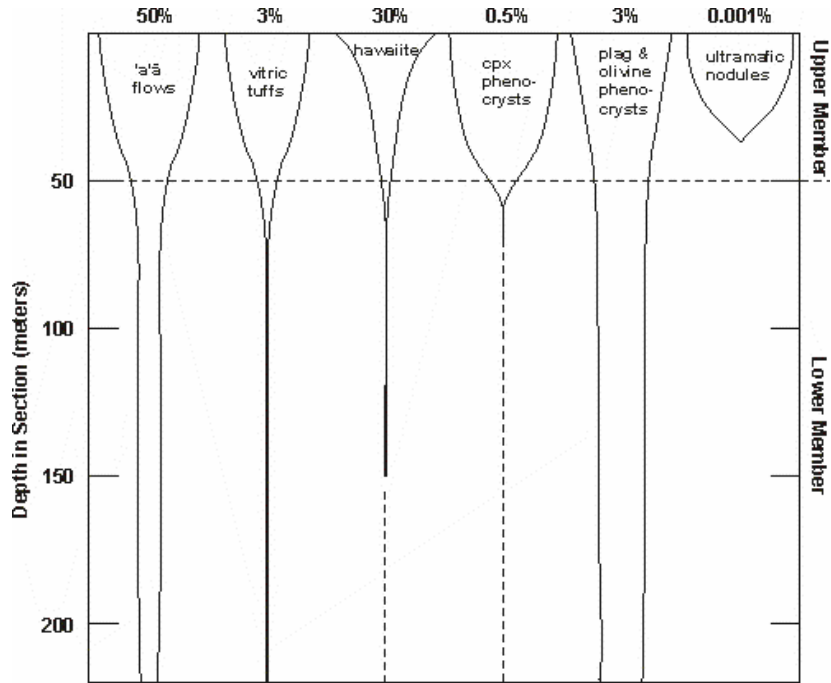
Figure 8. Schematic profiles through the upper part of the Wailuku Basalt, depicting changes in the relative abundances of 'a'ā flows, tuff beds, hawaiites, phenocryst phases and ultramafic xenoliths in the upper 50 m. Approximate maximum absolute values are indicated at the top of each profile. These variations constitute the basis for designating the Upper Member of the Wailuku Basalt (from Diller , 1982; Sinton et al. , 1987).
