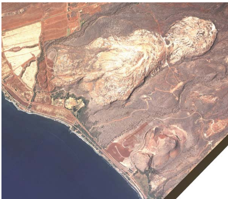
Figure 14. Aerial photograph of region around Launiupoko showing typical, white-weathering Pu‘u Māhanaluanui trachyte dome that formed simultaneously over a SW-trending fissure with another, unnamed dome. See Fig. 14 for flow planes.
