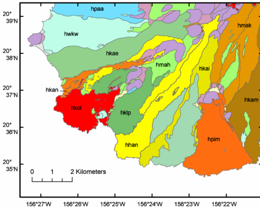
Figure 35. Geologic map of Honuaula area (after Bergmanis et al. [2000]; Sherrod et al. [written comm. 2001].
