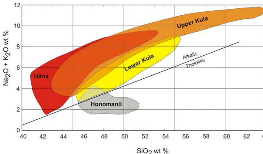
Figure 23. Total alkalis versus SiO 2 for East Maui Volcanic rocks (Sherrod et al. , 2003). Alkalic-tholeiitic dividing line from Macdonald and Katsura [1964] is shown for reference. Honomanū lavas range from tholeiitic to alkalic basalt. Lower Kula lavas are mainly alkali basalt and hawaiite; upper Kula rocks range from basanite to trachyte; Hāna volcanics are mainly basanites with subordinate hawaiite.
