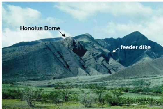
Figure 13. West wall of Ukumehame Valley, showing Honolua trachyte dome and feeder dike, intruding Wailuku basalts.
