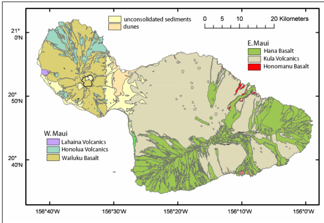
Figure 2. Geologic map of Maui, modified from Stearns and Macdonald, [1942]; Macdonald et al. [1983]; Bergmanis et al. [2000], and Sherrod et al. [2003, in prep.]
