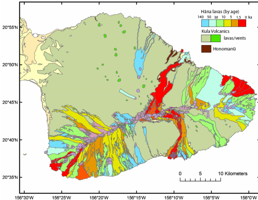
Figure 22. Geologic map of East Maui (after Stearns and Macdonald [1942]; Bergmanis et al. [2000]; and Sherrod et al. [2003; in prep].
