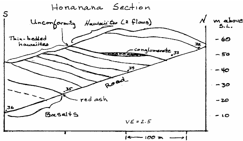
Figure 17. Schematic section of the roadcuts on the west side of Hononana Gulch. All units are in the Upper Member of the Wailuku Basalt.
