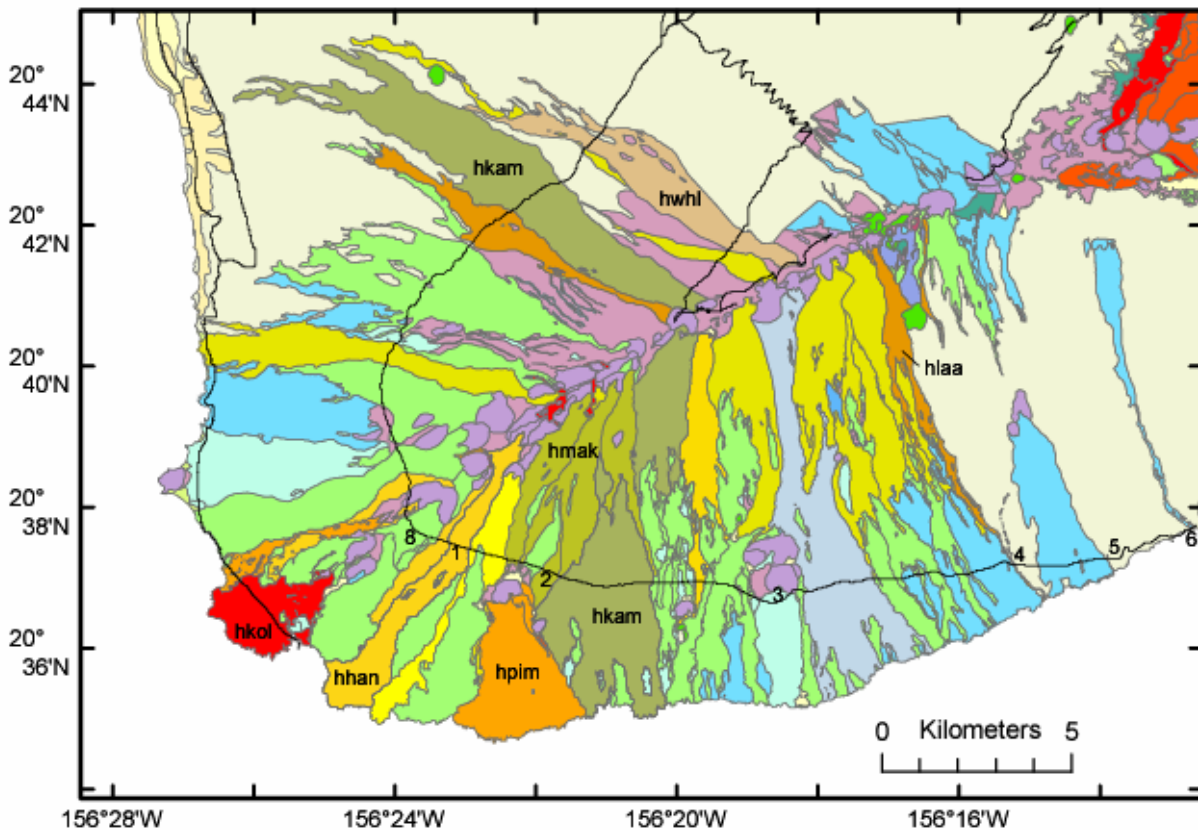
Figure 29. Geologic map of the southwest rift zone, East Maui, (after Bergmanis et al. [2000] and Sherrod et al. [in prep]). Numbers indicate stops referred to in the field guide.
