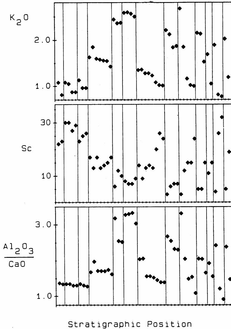
Figure 28. Up-section variations in K_2O , Sc and Al_2O_3/CaO for Kula lavas from the Halemau'u trail section. Vertical lines indicate geochemical discontinuities that reflect individual magma batches. (from West et al. , 1987).
