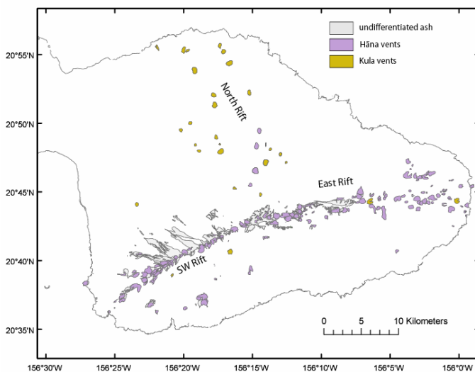
Figure 21. Vent distribution defines three rift zones that intersect near the present summit of East Maui.
