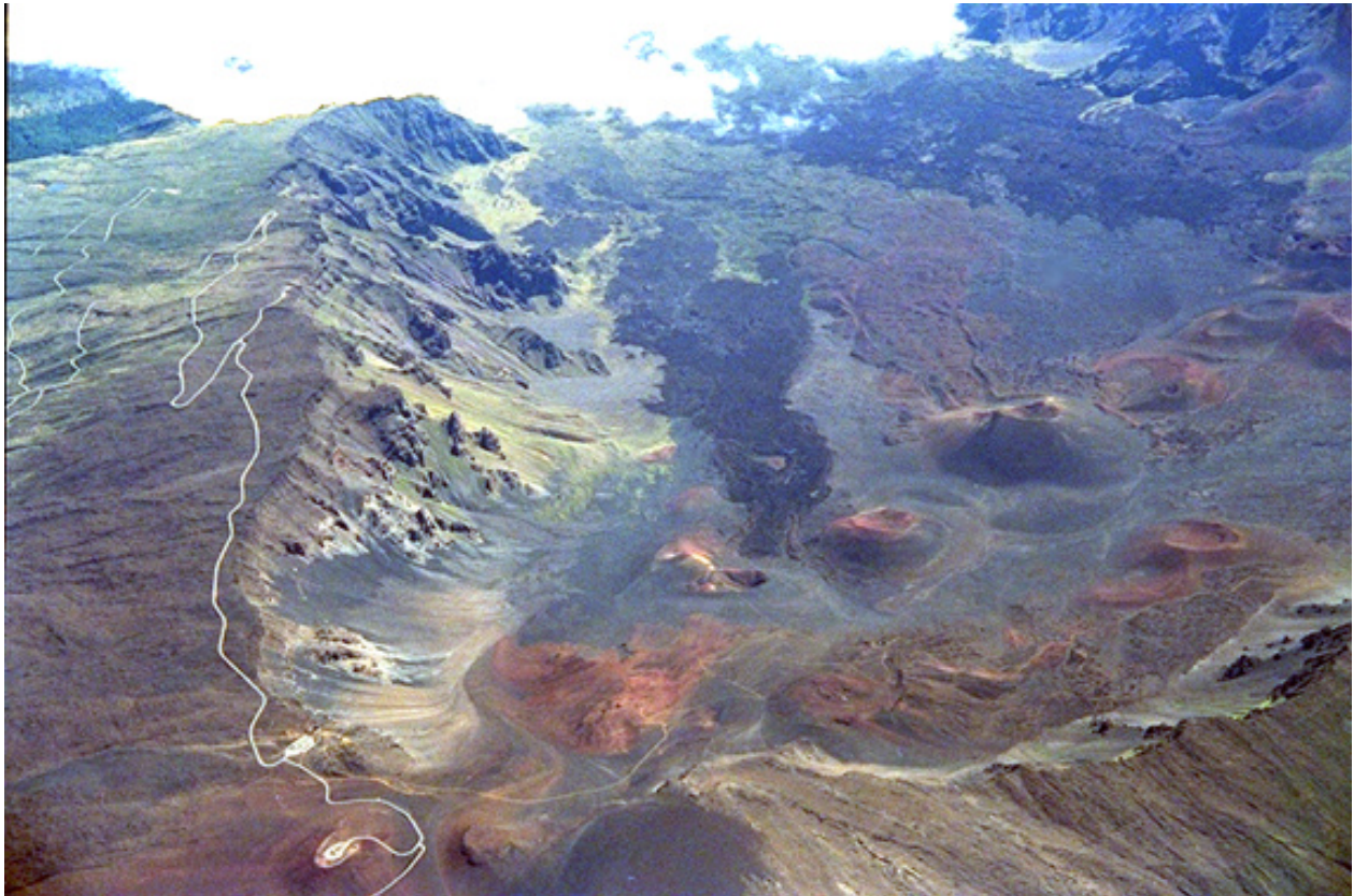
Figure 25. Air view of Haleakalā Crater looking northeast (image courtesy of NASA Virtually Hawai‘i Project). The two dark-colored flows in the center of the picture and along the far side of the crater have been dated by ^{14}\text{C} to 970 \pm 50 and 940 \pm 50 yrs B.P, respectively. ( Sherrod and McGeehin , 1999).
