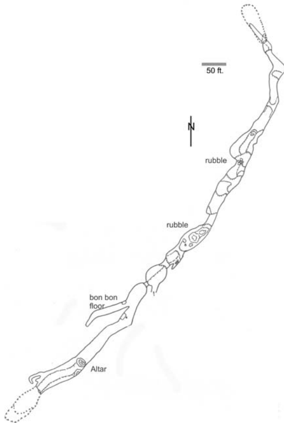
Figure 27. Hōlua lava tube, Haleakalā. [Sinton, Johnson and Mallonee, unpublished].
