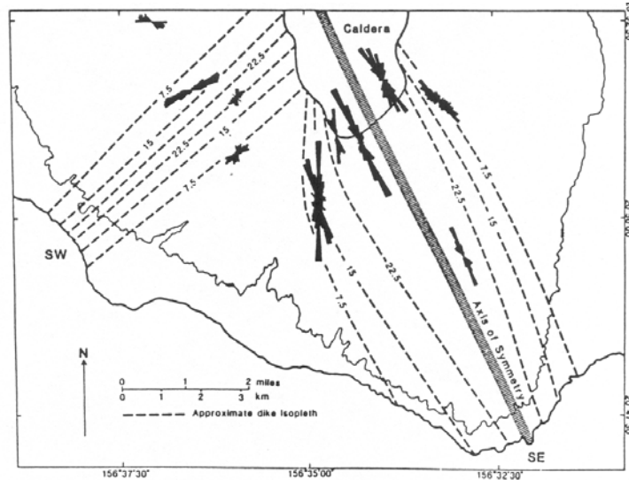
Figure 6. Dike isopleths in intervals of 7.5 dikes/100 m along traverses in the SW part of West Maui. Rose diagrams for various areas indicate dike orientations scaled according to the number of measurements taken, not the number of dikes present (from Diller [1982]).
