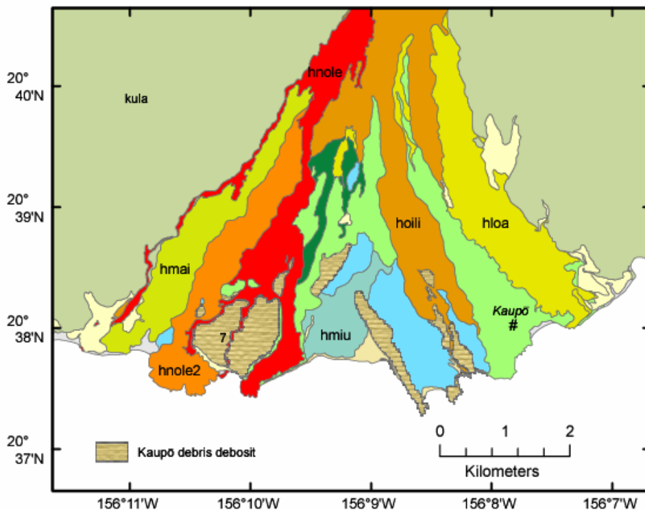
Figure 32. Geologic map of the Kaupō area, showing the distribution of lava flows (all erupted inside Haleakala Crater and flowed down through Kaupō Gap) and the Kaupō debris deposit.
