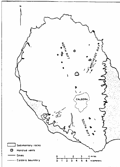
Figure 5. Principal rift zones of West Maui as defined by dike and vent concentrations (from Macdonald et al. [1983])
