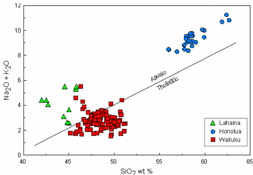
Figure 9. Alkali-silica diagram for West Maui volcanic rocks. Alkalic-tholeiitic dividing line is from Macdonald [1968].
