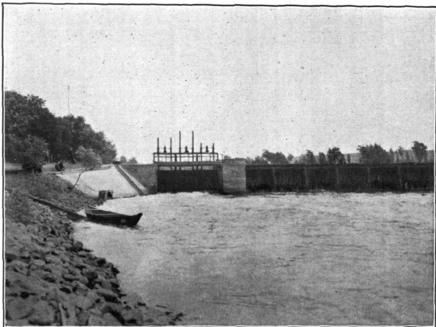
1. The dam in Gruetz on the Havel seen from below; on the right side on the picture the needleweir and on the left side the rampart. Left from it the sloping wall and on its upper edge the trap. (Photographs by Dr. Roehler.)
