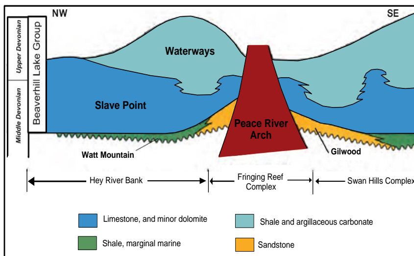
Figure 3: Schematic strata showing the location of the Peace River Arch and the overlying Devonian strata. The bedrock, the bedrock interface, and the Watt Mountain and Gilwood formations are the prime targets for fluid production for geothermal purposes. The Duvernay is stratigraphically above the Beaverhill Lake Group.
