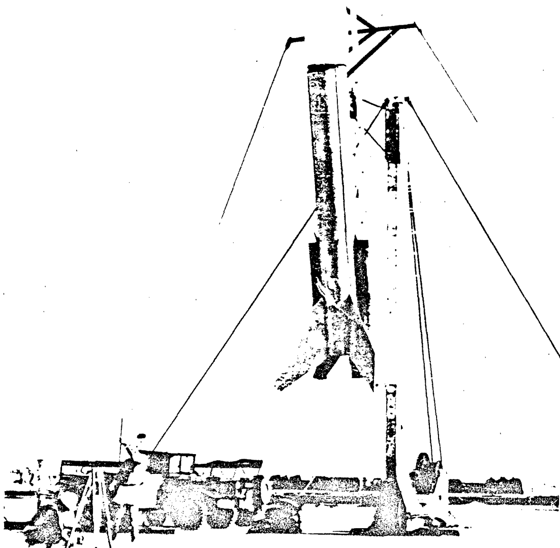
Figure 88. Stryl missile with Recruit boosters used for CHECKMATE shot, Operation DOMINIC.
