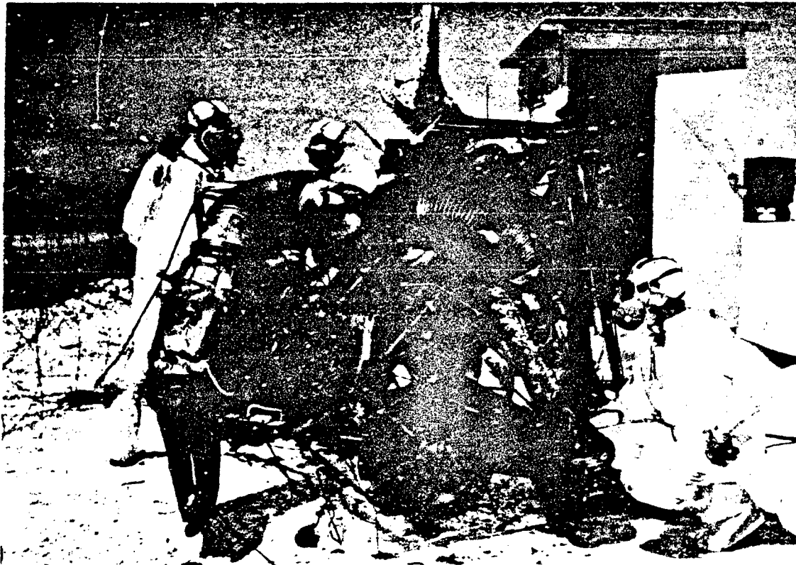
Figure 98. Inspection of Thor engine parts following BLUEGILL Prime fire on Johnston Island, Operation DOMINIC.
