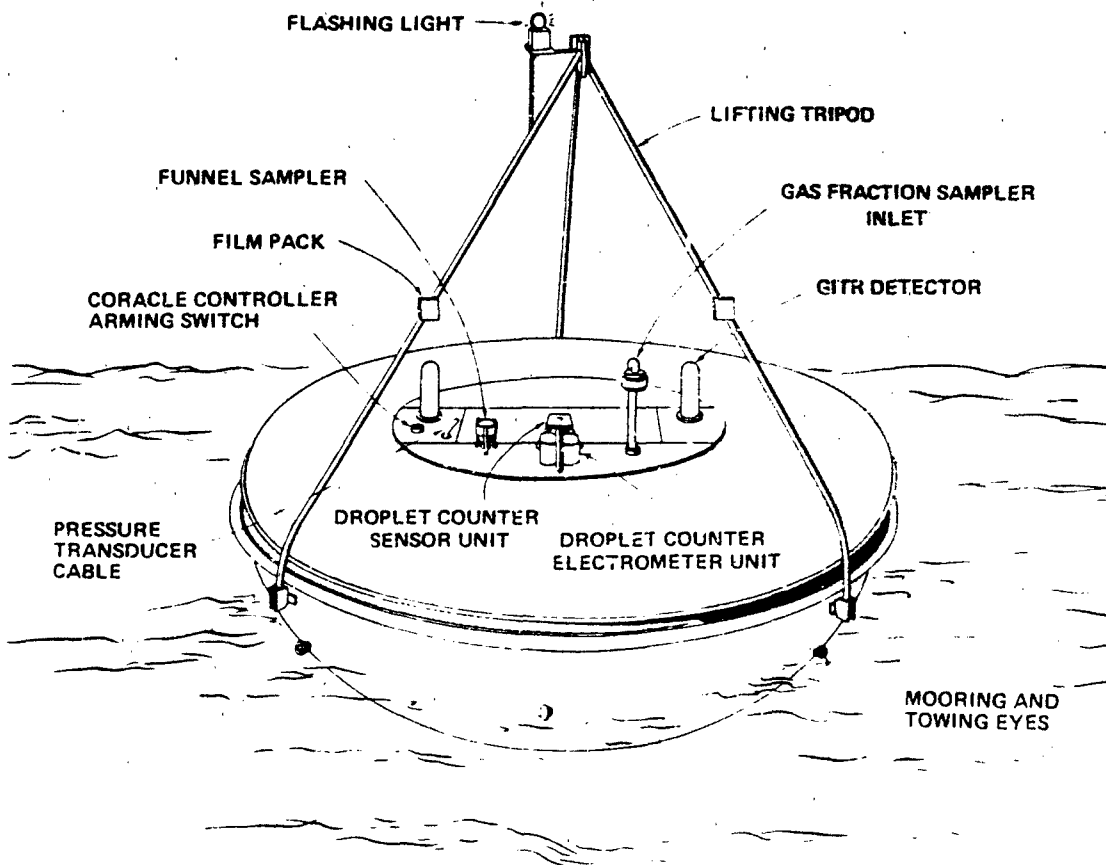
Figure 77. Coracle used for DOMINIC, SWORDFISH.
