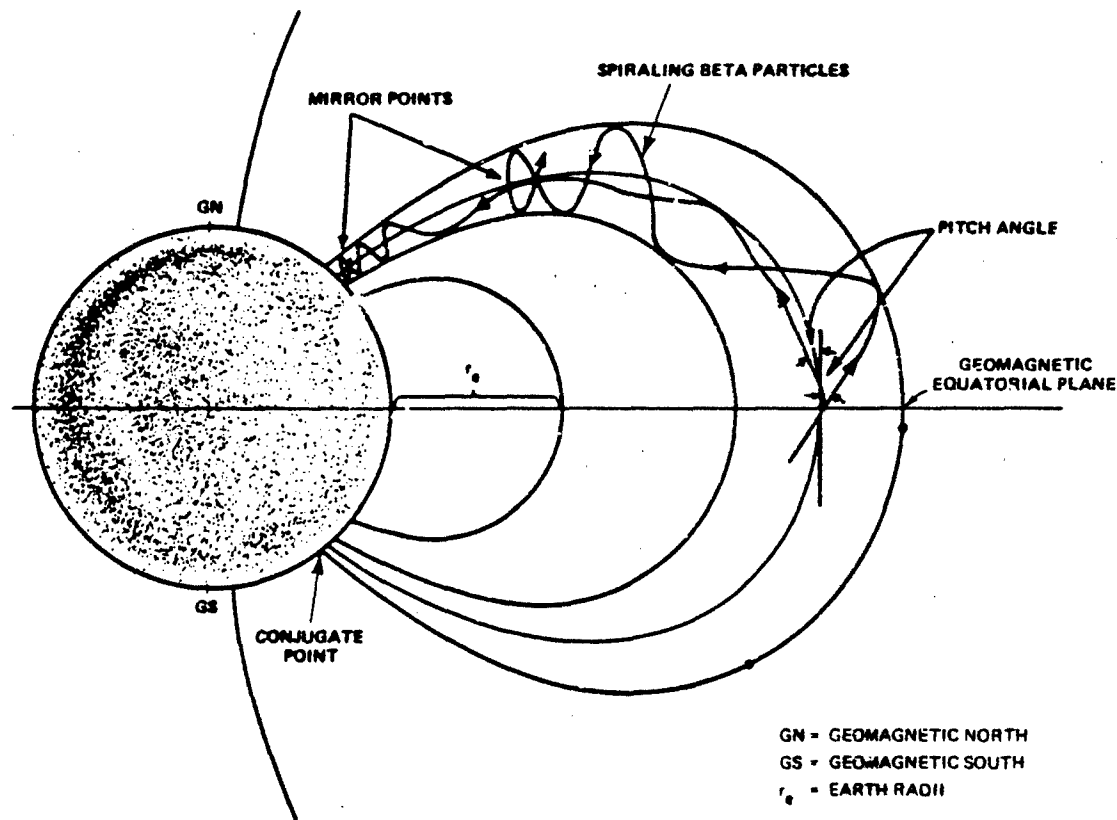
Figure 86. Earth's magnetic field.
