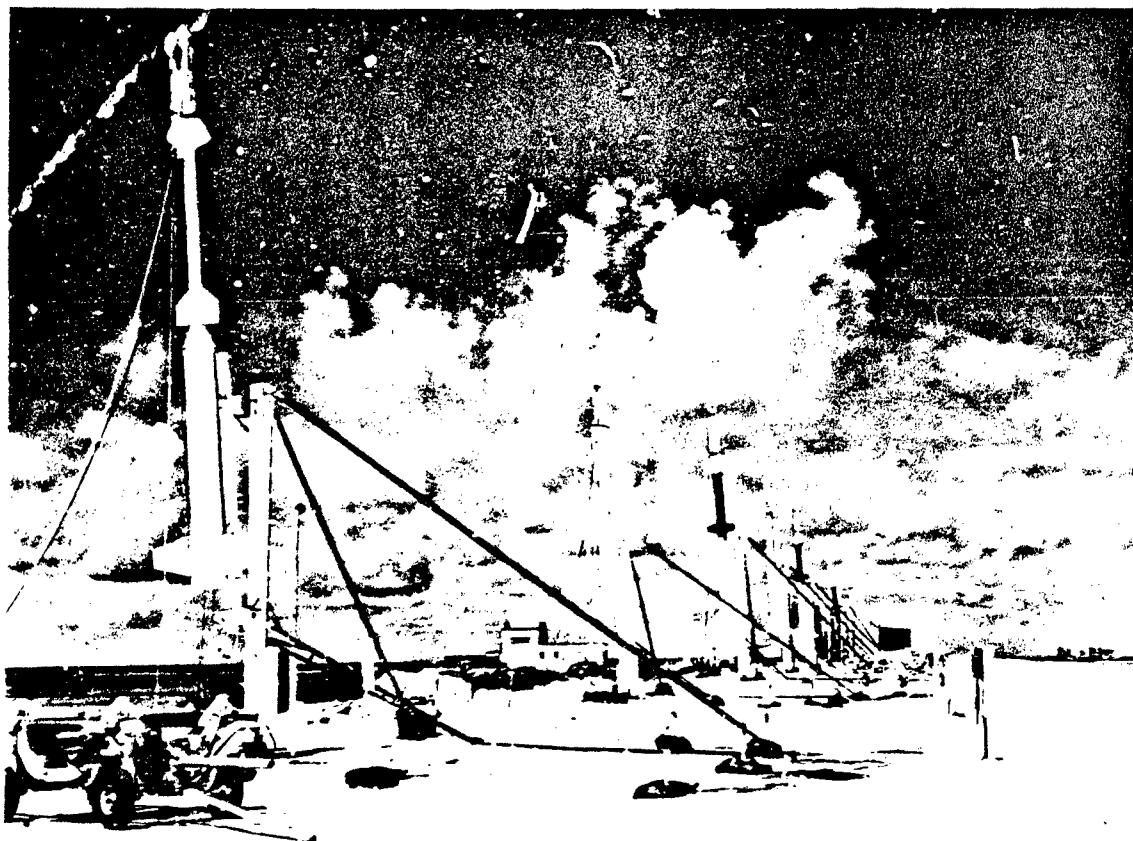
Figure 89. Array of instrument rockets used during Operation DOMINIC at Johnston Island.
