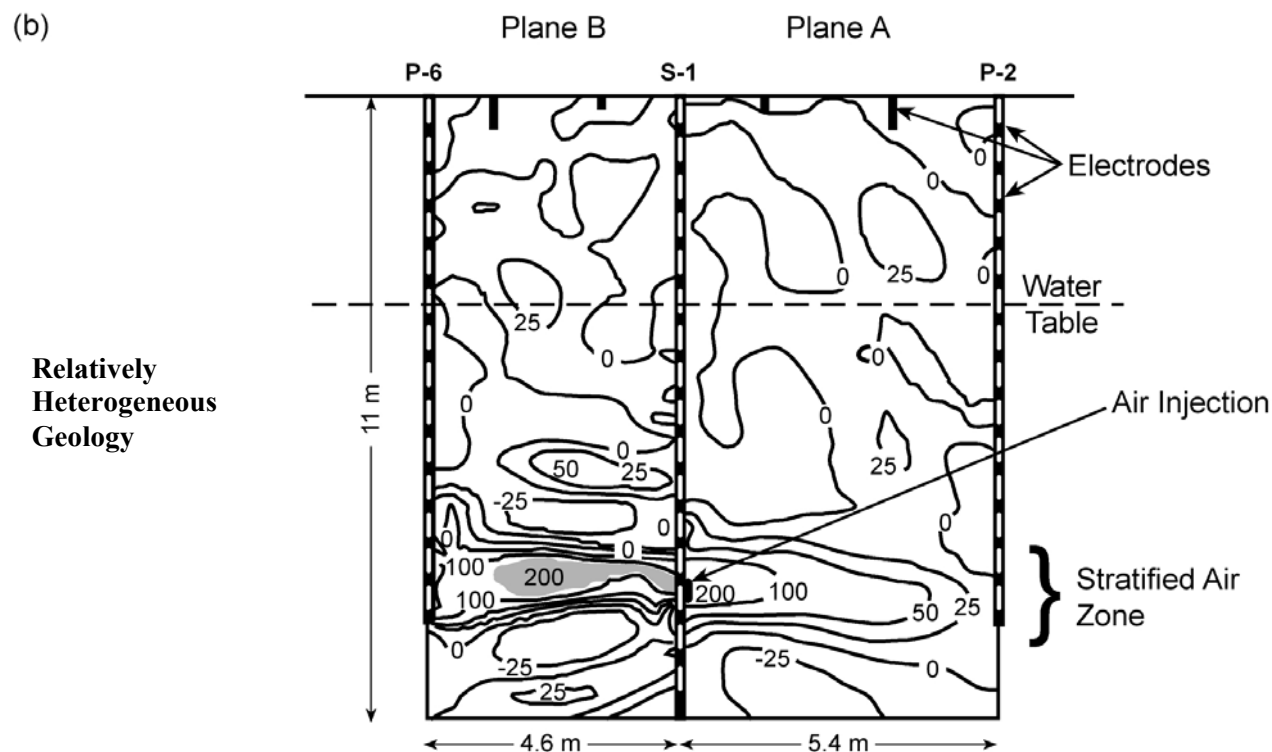
Figure 2. Air Flow Distributions in Homogeneous and Heterogeneous Hydrogeologic Settings
