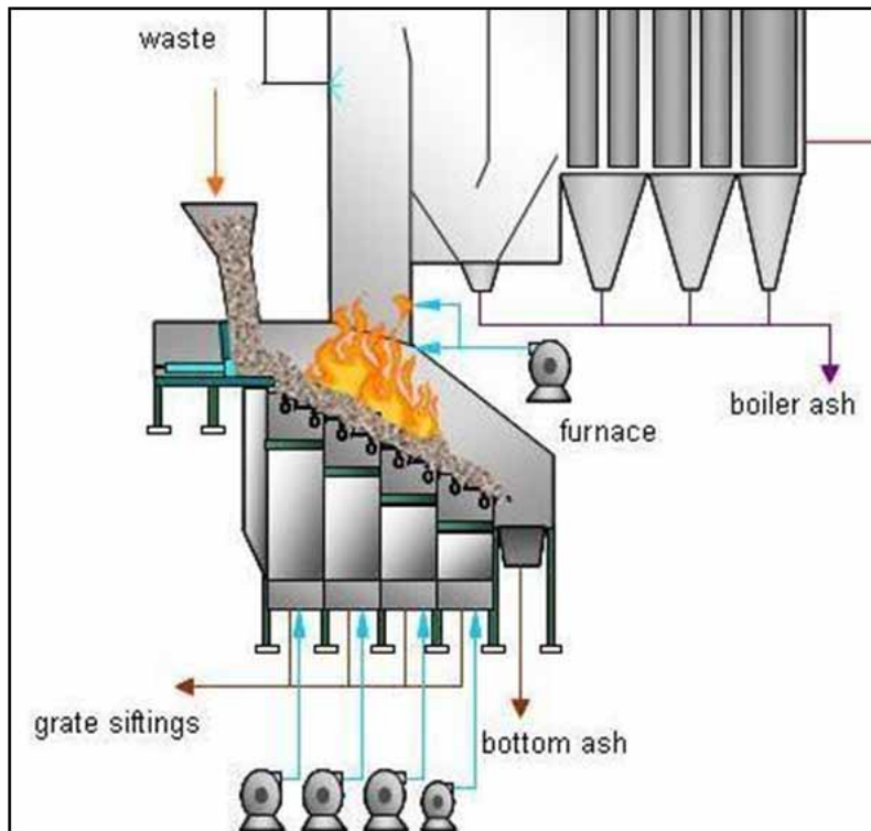
Figure 9. Incineration grate.
