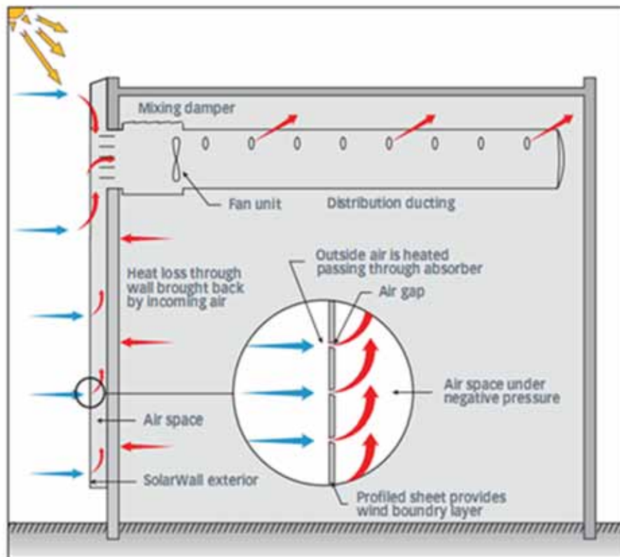
Figure 13. Interior fan system.
