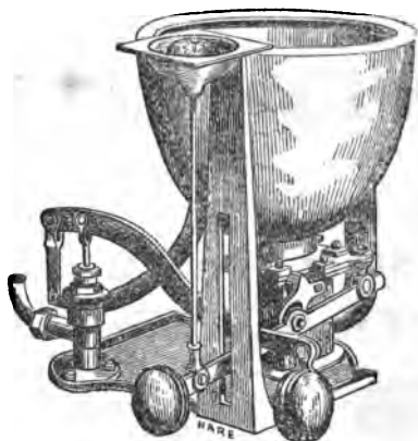
Valve Closet, With Howard's Patent Regulator.
