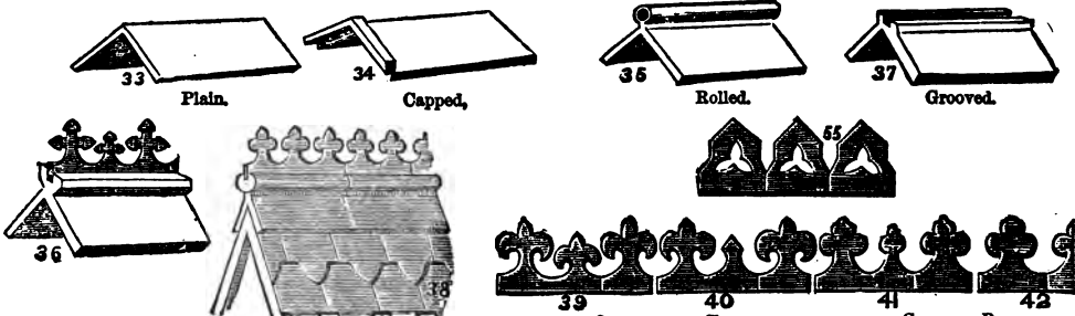
ORNAMENTAL TOPS TO BE INSERTED IN GROOVED RIDGES
