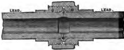
SECTION OF LEAD COUPLING.
