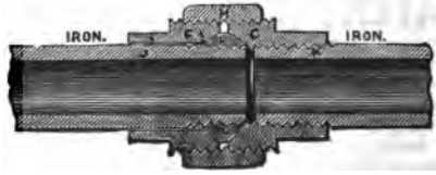
SECTION OF IRON UNION. (L) Lead Ring.
