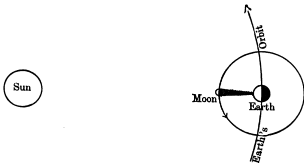
Fig. 15. Total Eclipse of Sun.
