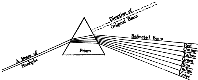
Fig. 9. Refraction and Dispersion.
