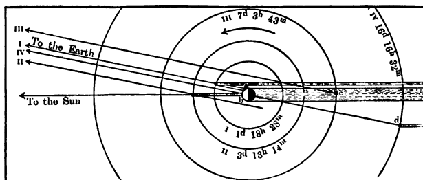
Fig. 22. Transits, Eclipses, and Occultations of Jupiter's Satellites.
