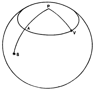
Fig. 5. Right Ascension and Declination.
