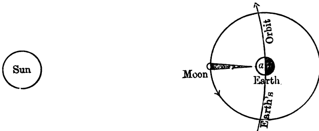
Fig. 16. Annular Eclipse of Sun.
