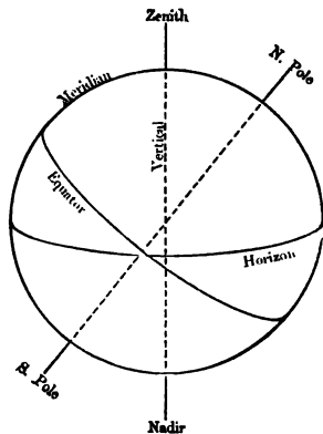
Fig. 4. The Celestial Sphere.
