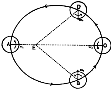
Fig. 17. Libration of the Moon in Longitude.
