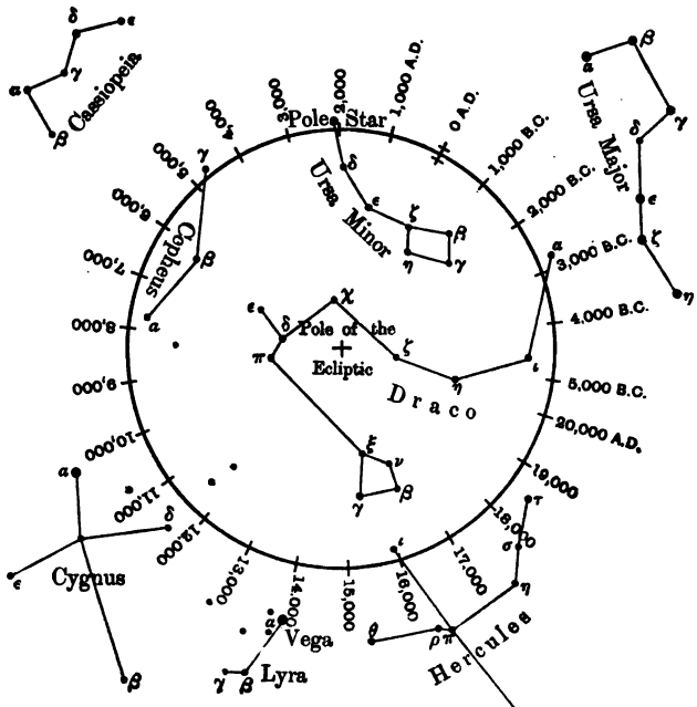
Fig. 23. Precessional Movement of the Pole.
