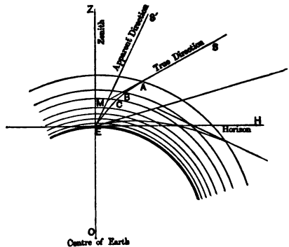
Fig. 1. Atmospheric Refraction.
