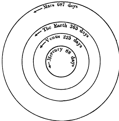
Fig. 19. The Inner Planets.
