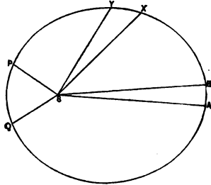
Fig. 18. The Ellipse and Kepler's Laws.
