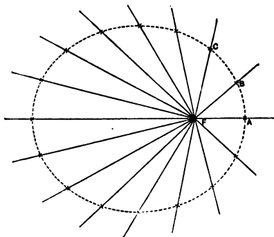
Fig. 12. Apparent Track of the Sun.
