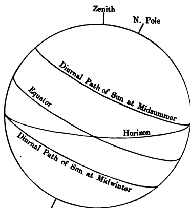
Fig. 11. Arctic Day and Night.
