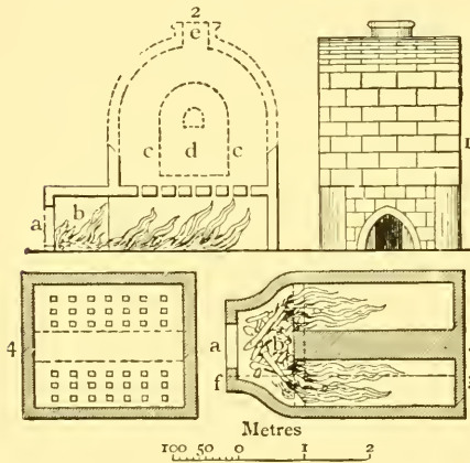
FIG. 212. ROMAN KILN FOUND AT HEDDERNHEIM, GERMANY.
