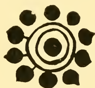
FIG. 169. ROSETTE (RHODIAN).
