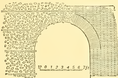
FIG. 189. CONCRETE ARCH; HALF WITH BRICK FACING REMOVED.
