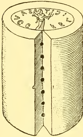
FIG. 201. TERRACOTTA COIN-MOULD.
