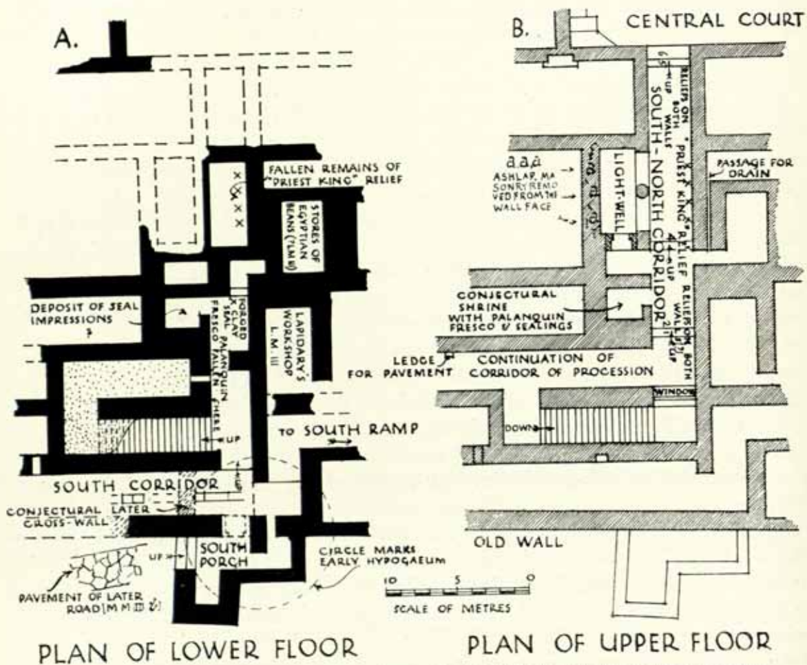
FIG. 490. A, B, PLANS SHOWING APPROACH FROM SOUTH PORCH AND 'SOUTH-NORTH CORRIDOR'.
