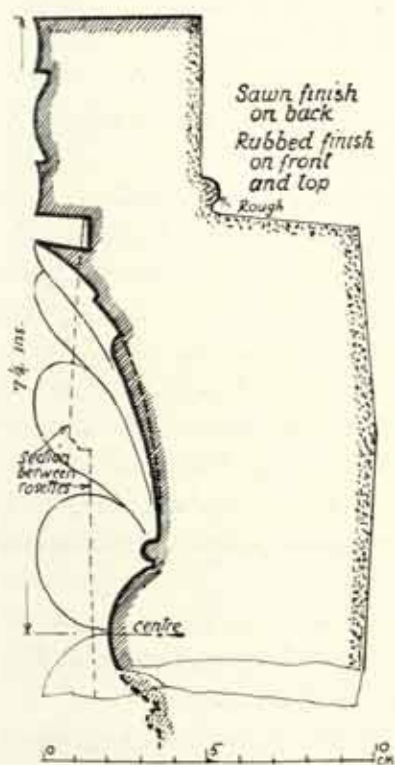
FIG. 437. SECTION OF ROSETTE. THEODORE FYFE.
