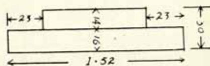
FIG. 530. INTERMEDIATE COLUMN-BASE OF 'STEPPED PORCH', RESTORED.
