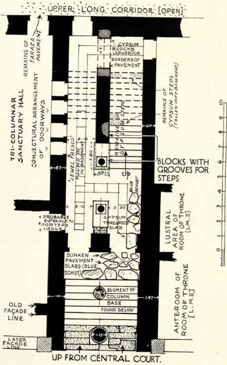
FIG. 536. RESTORED PLAN, SHOWING STEPPED PORCH WITH THROUGH CORRIDOR TO LEFT, AND CENTRAL STAIRS TO RIGHT.
