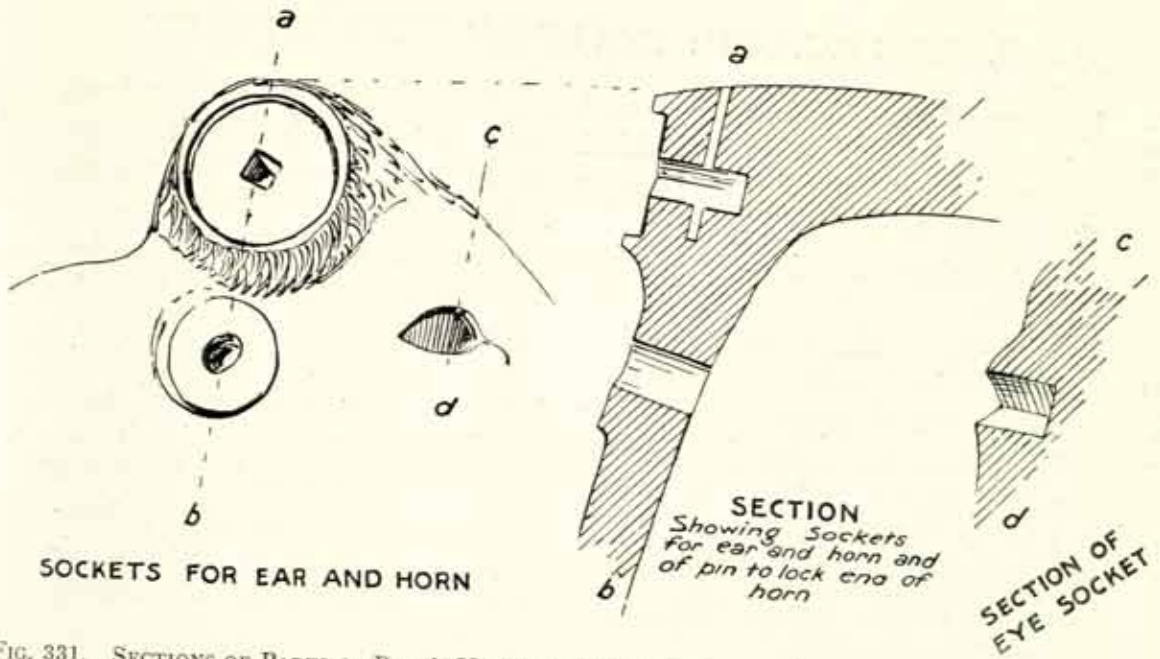
FIG. 331. SECTIONS OF PARTS OF BULL'S HEAD SHOWING SOCKETS FOR ATTACHMENT OF EAR AND HORN, AND EYE SOCKET.
