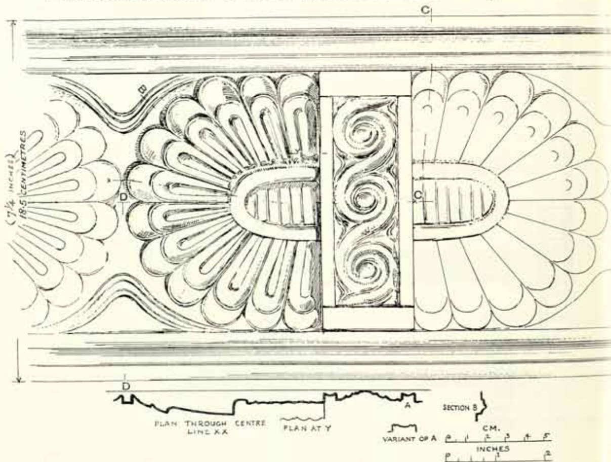
FIG. 370. PLAN AND SECTION OF PART OF TRIGLYPH AND HALF-ROSETTE BAND. BY THEODORE FYFE. (SEE ALSO HIS SECTION IN SUPPL. PL. XXII.)
