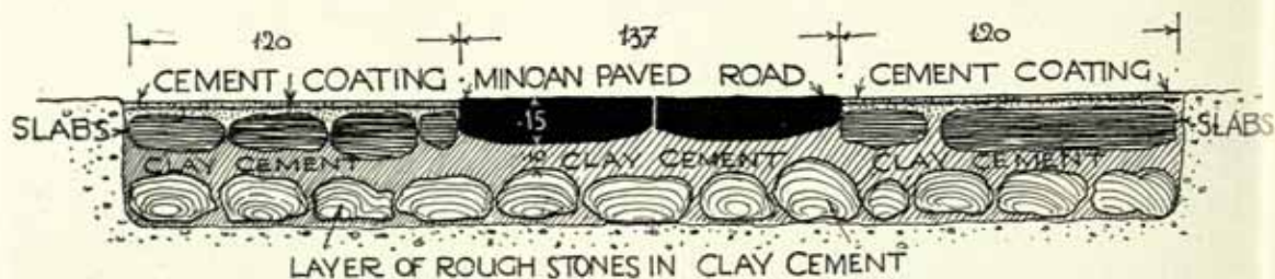
FIG. 359. SECTION OF MINOAN PAVED WAY (THE 'ROYAL ROAD').
