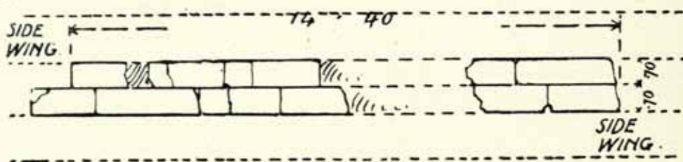
FIG. 358. PLAN OF PART OF PAVING OF MINOAN WAY.
