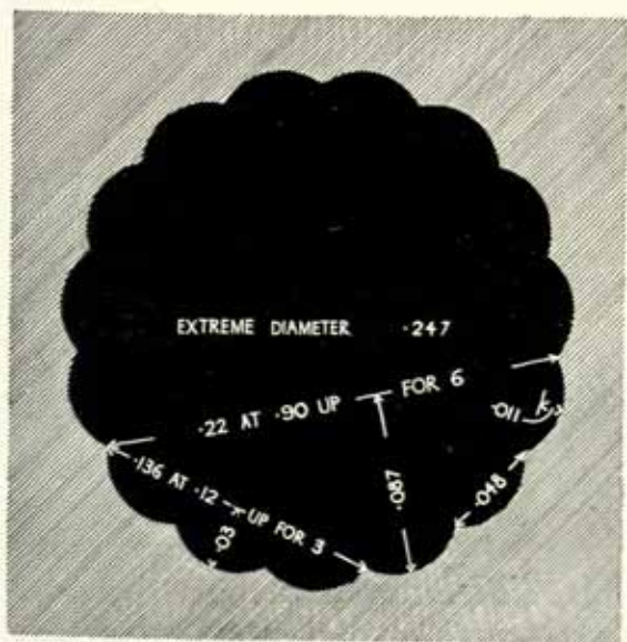
FIG. 324. SECTION OF RESTORED COLUMN OF 'LUSTRAL AREA'. CHRISTIAN C. T. DOLL.
