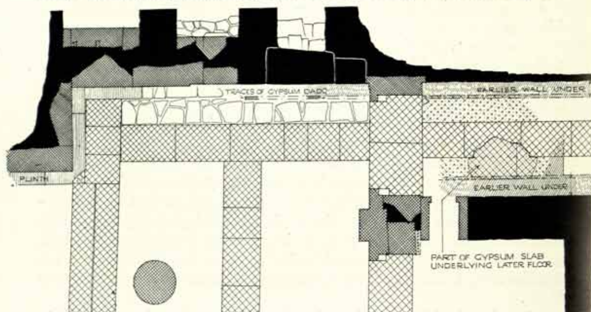
FIG. 425. PLAN OF SECTION OF WEST ENTRANCE SHOWING LINES OF EARLIER DADO AND OF WALLS OF NARROWER PASSAGE.
