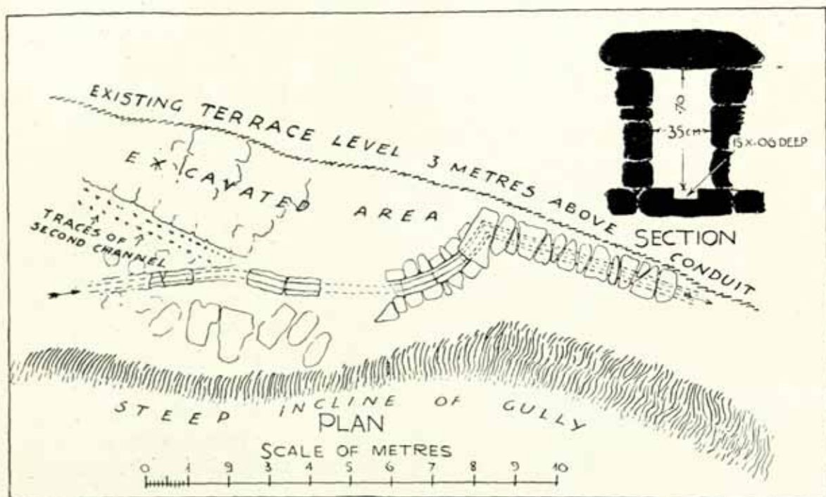
FIG. 273. PLAN OF SECTION OF MINOAN CONDUIT NEAR THE MAVROKOLYBO SOURCE, WEST OF KNOSSOS.
