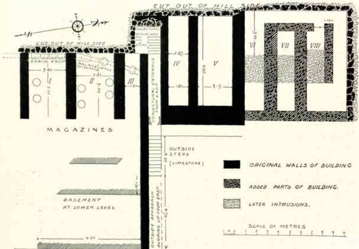
FIG. 240. BASEMENT PLAN OF NORTH-EAST HOUSE.
