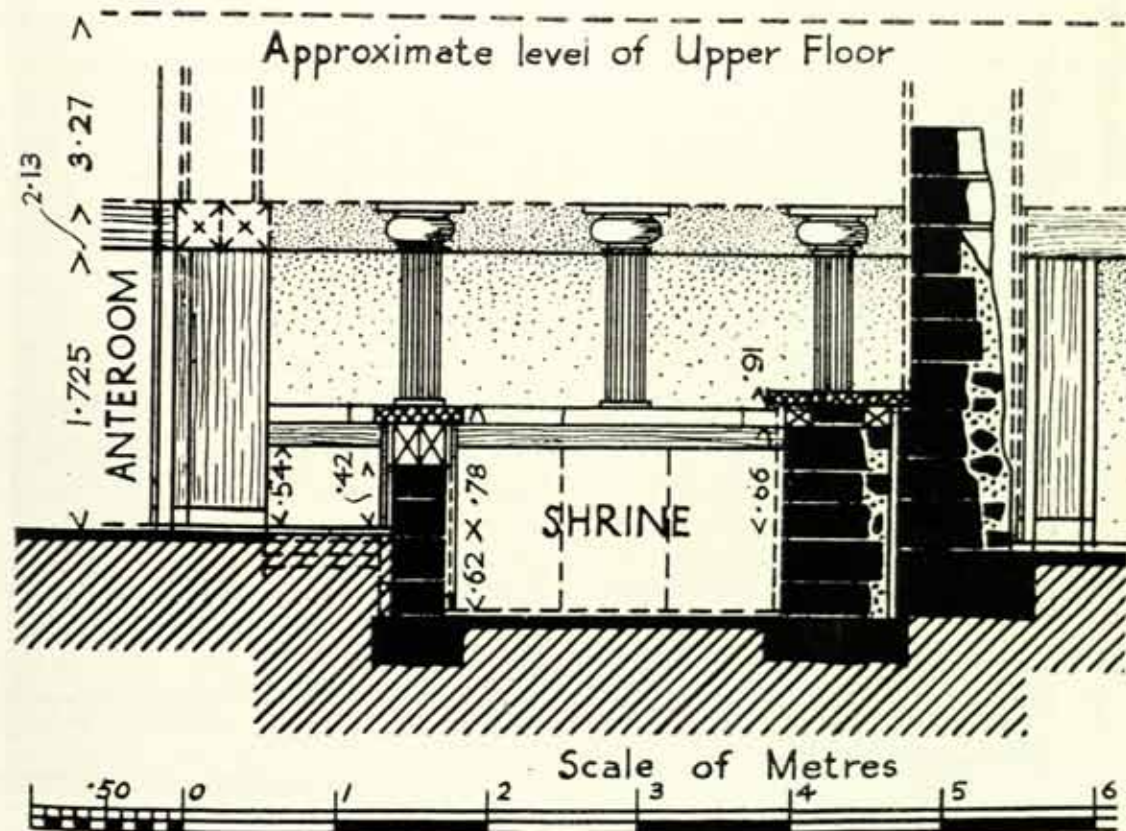
FIG. 322. SECTION SHOWING ELEVATION OF SUNKEN (LUSTRAL) AREA (LATER 'FETISH SHRINE'). BY CHRISTIAN C. T. DOLL.
