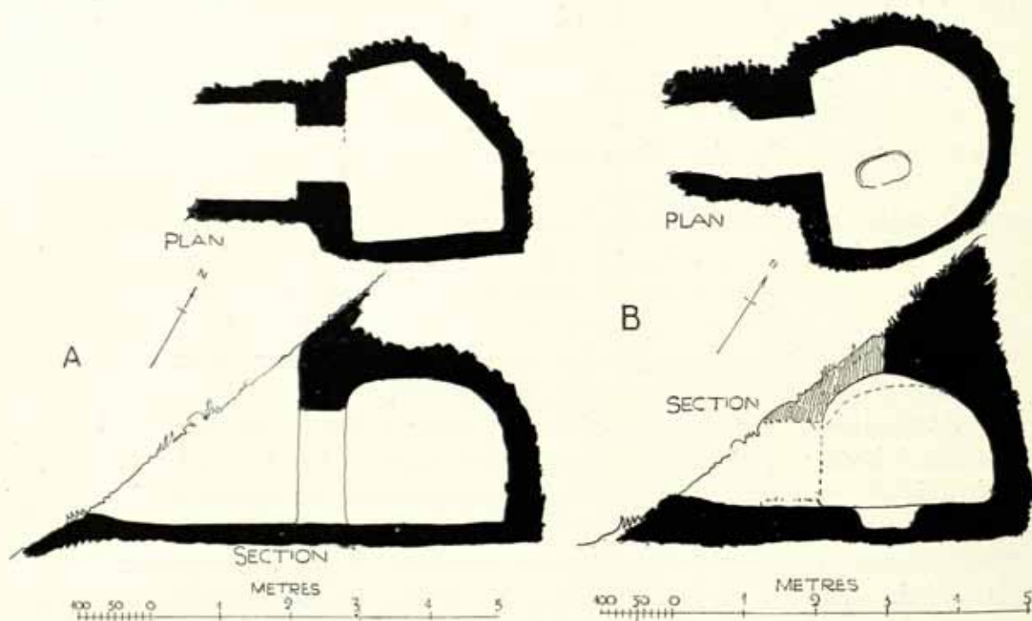
FIG. 351. PLAN AND SECTION OF CHAMBER TOMBS 1 (A) AND 3 (B); M. M. III a . MAVRO SPELIO, KNOSSOS.
