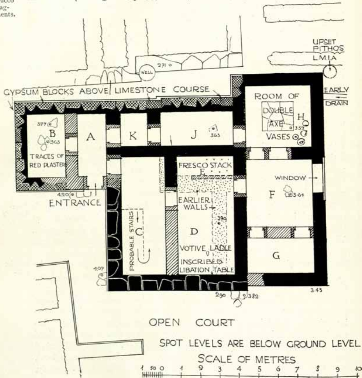
FIG. 251. PLAN OF 'HOUSE OF THE FRESCOES' (LOOKING EAST).
