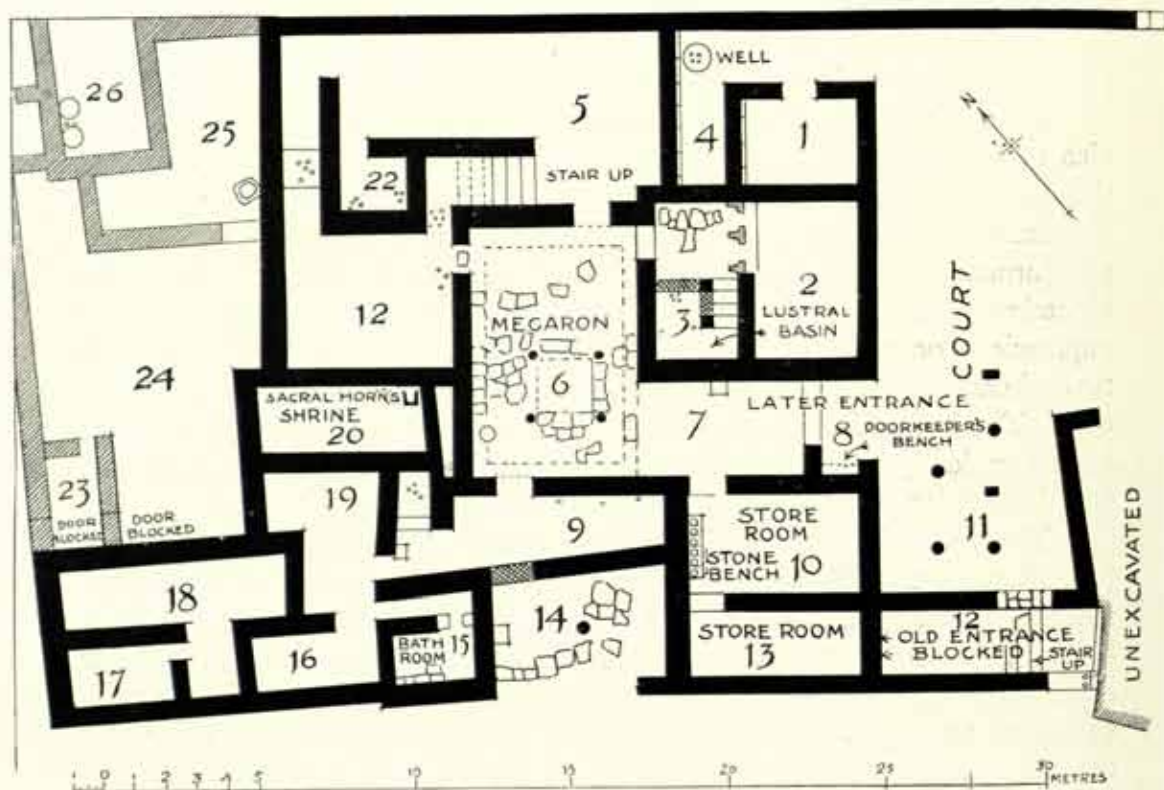
FIG. 354. PLAN OF 'HOUSE B' AT PALAIKASTRO.
