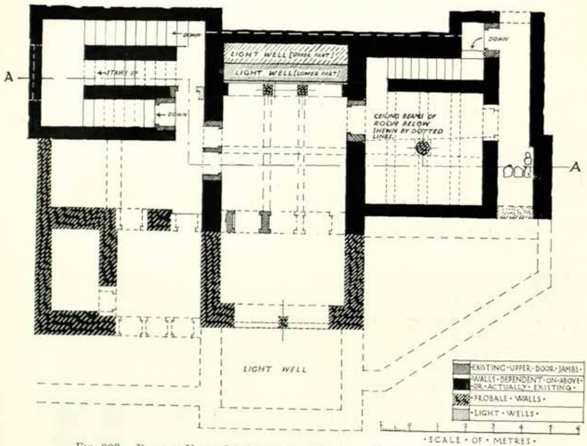
FIG. 228. PLAN OF UPPER STORY, 'ROYAL VILLA'; BY THEODORE FYFE, F.R.I.B.A.
