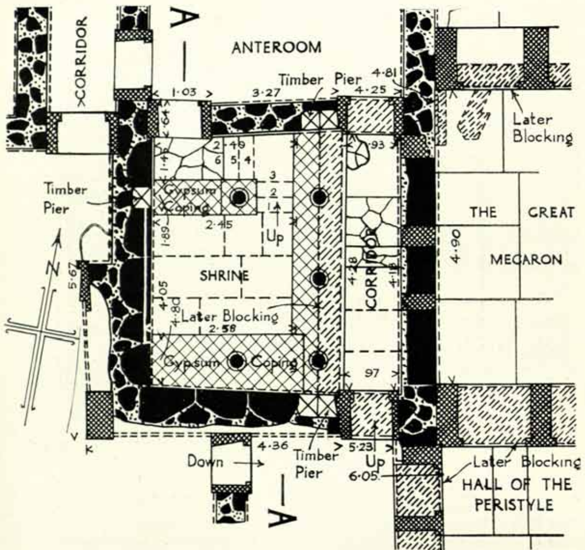
FIG. 321. PLAN OF LUSTRAL AREA OF 'LITTLE PALACE'. BY CHRISTIAN C. T. DOLL.
