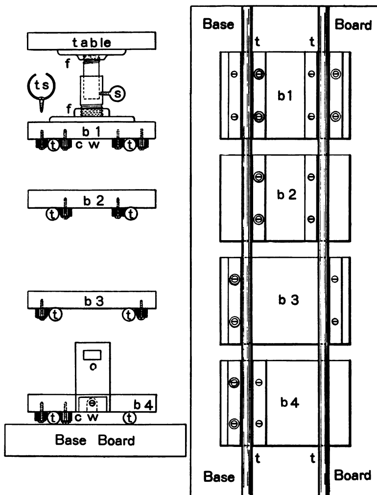
FIG. 159. HOME-MADE OPTICAL BENCH FOR ALL PURPOSES.
