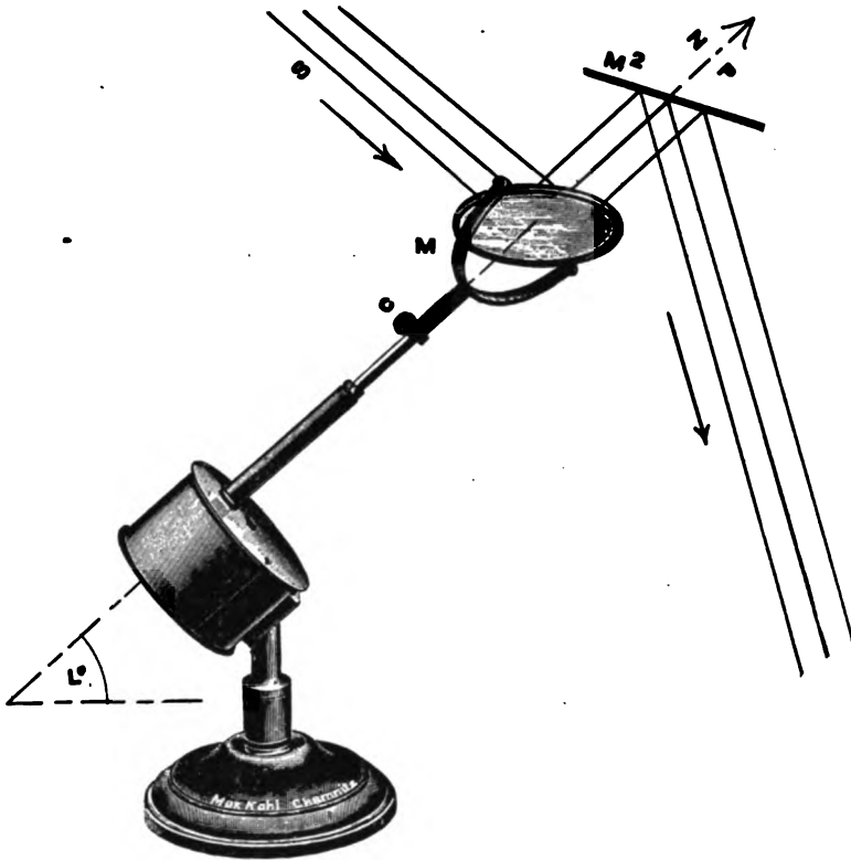
FIG. 81. TWO-MIRROR HELIOSTAT WITH THE MOVABLE MIRROR AT THE END OF THE CLOCK-SHAFT.
