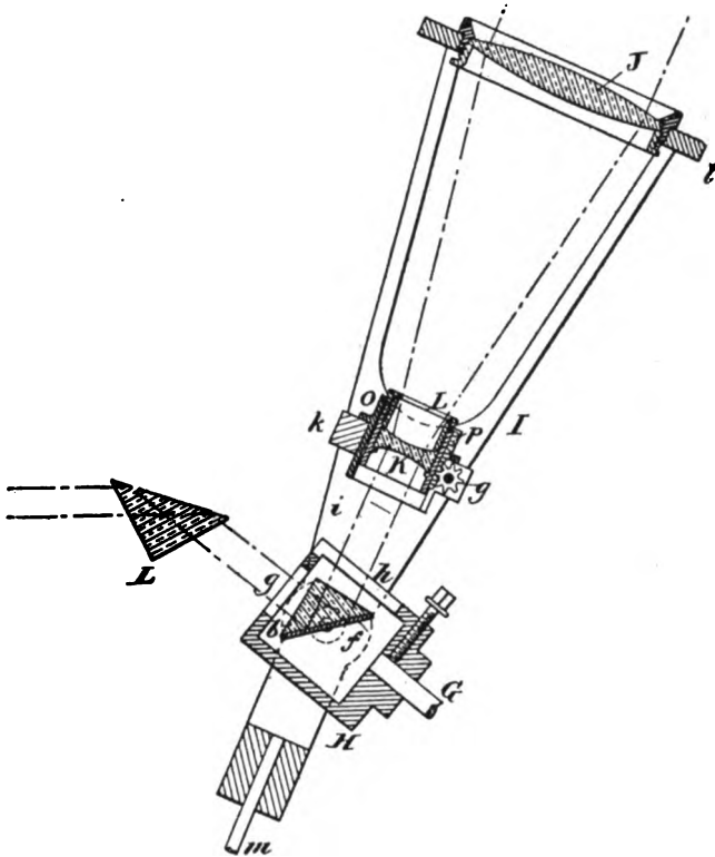
FIG. 83. LENS AND PRISM HELIOSTAT OF ALFRED M. MAYER. (From the American Journal of Science, Vol. 154, 1897).
