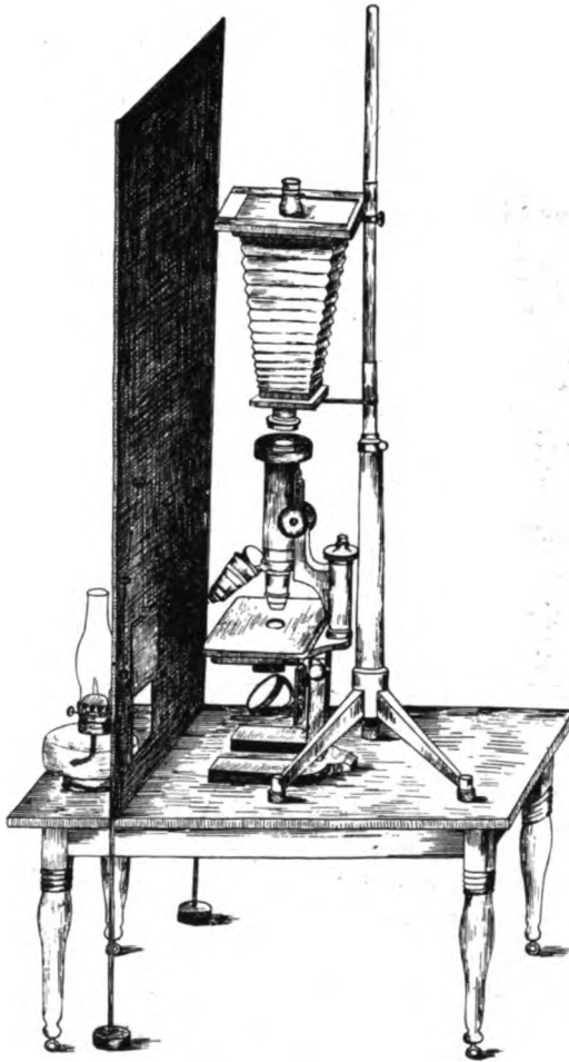
FIG. 217A. VERTICAL CAMERA WITH METAL SHIELD.
