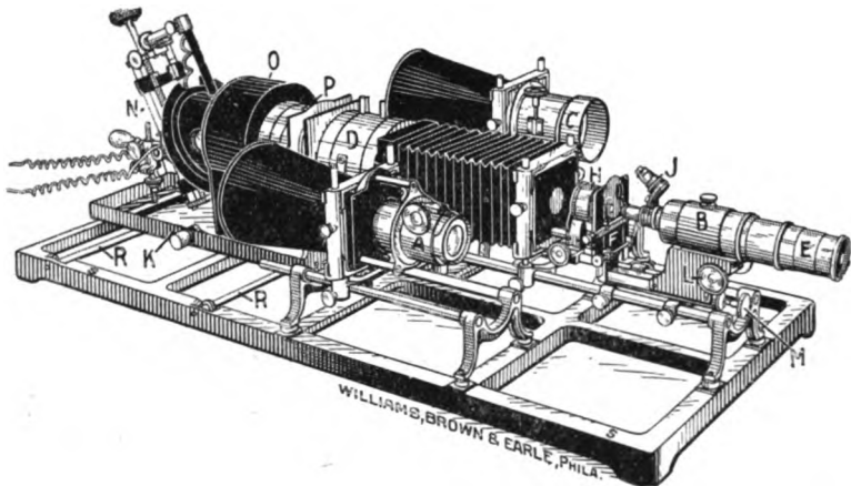
FIG. 164. PROJECTION MICROSCOPE, MAGIC LANTERN AND MEDIOSCOPE WITH SINGLE RADIANT.
