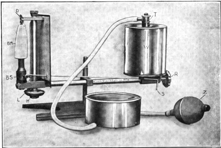
FIG. 73. ALCO-RADIANT, SHOWING THE PARTS. (Cut loaned by Williams, Brown & Earle).
