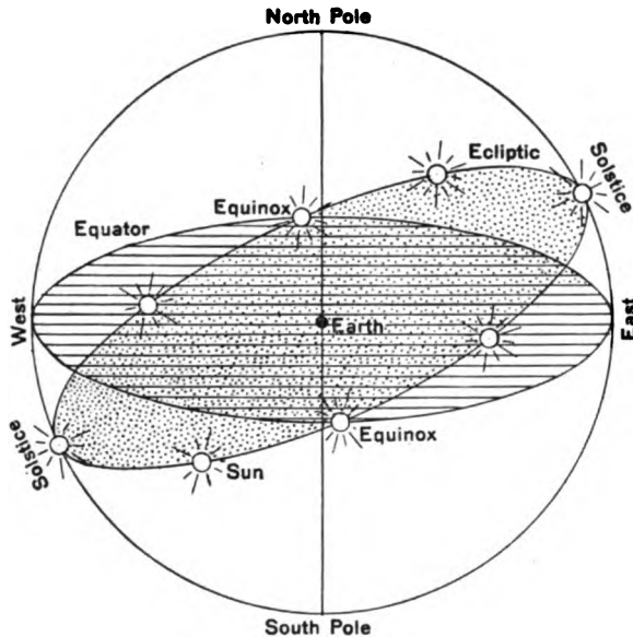
FIG. 86. DIAGRAM OF THE CELESTIAL SPHERE WITH THE PLANES OF THE CELESTIAL EQUATOR AND OF THE ECLIPTIC; AND WITH THE APPARENT POSITION OF THE SUN AT DIFFERENT SEASONS.
