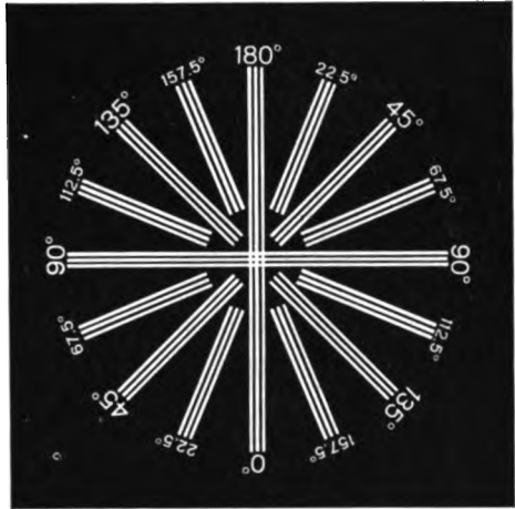
FIG. 391-392. RADIAL LINES IN BLACK AND WHITE FOR DETERMINING THE PRESENCE OF ASTIGMATISM.
