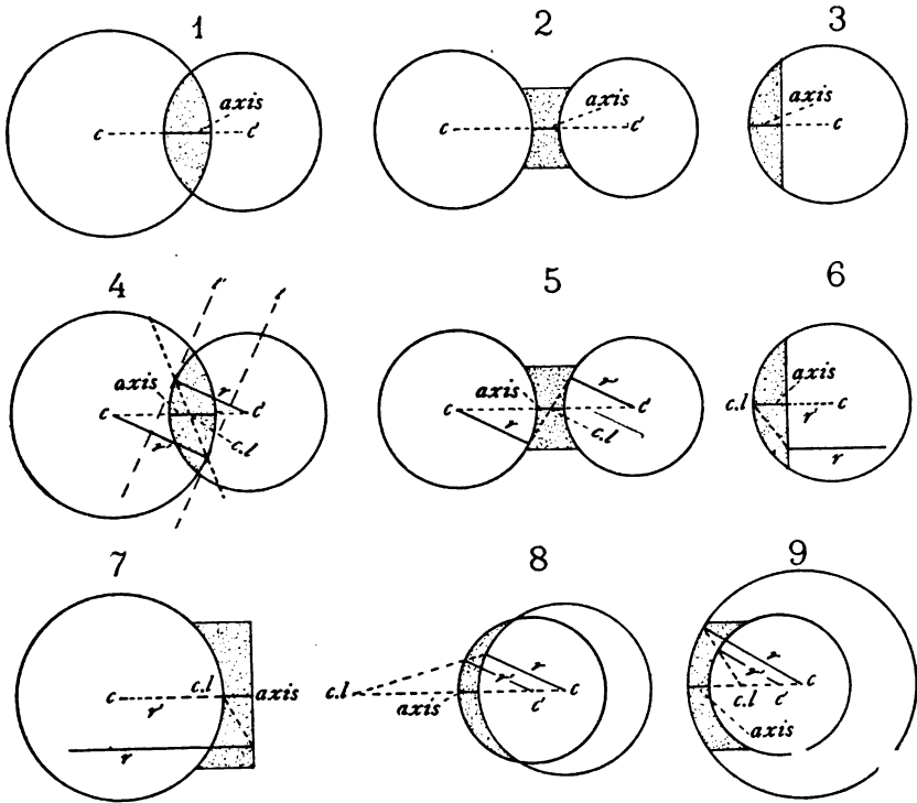
FIG. 314. THE OPTIC CENTER AND THE PRINCIPAL OPTIC AXIS OF VARIOUS FORMS OF LENSES.
