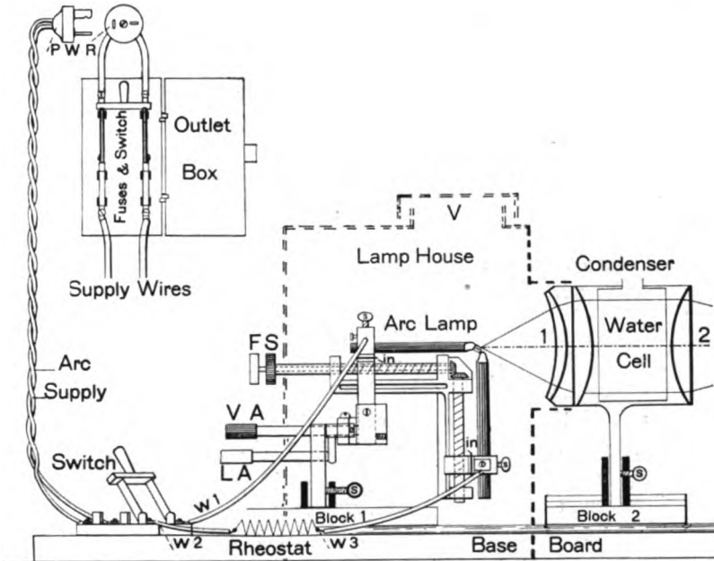
FIG. 270. WIRING OF THE ARC LAMP FOR PROJECTION. For full explanation, see fig. 3 and fig. 40.
