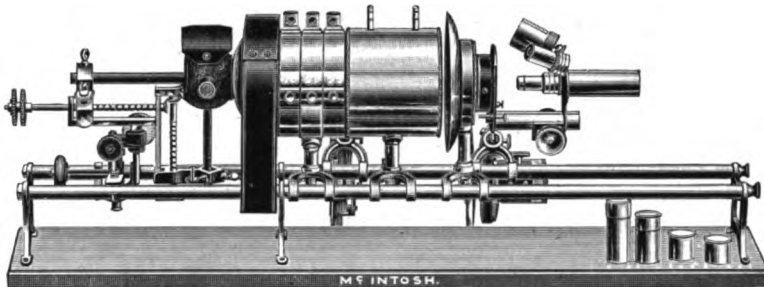
FIG. 166. IMPROVED, COLLEGE, BENCH LANTERN ARRANGED FOR MICRO-PROJECTION.
