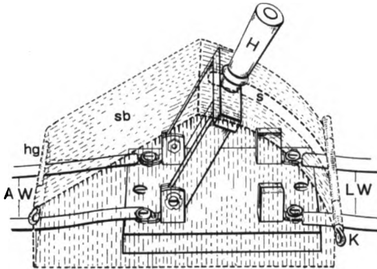
FIG. 278. ENCLOSED SWITCH IN A HORIZONTAL POSITION.
