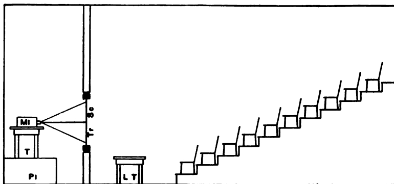
FIG. 245. SECTIONAL VIEW OF A LECTURE ROOM SHOWING THE POSITION OF THE PROJECTION APPARATUS WITH A TRANSLUCENT SCREEN.
