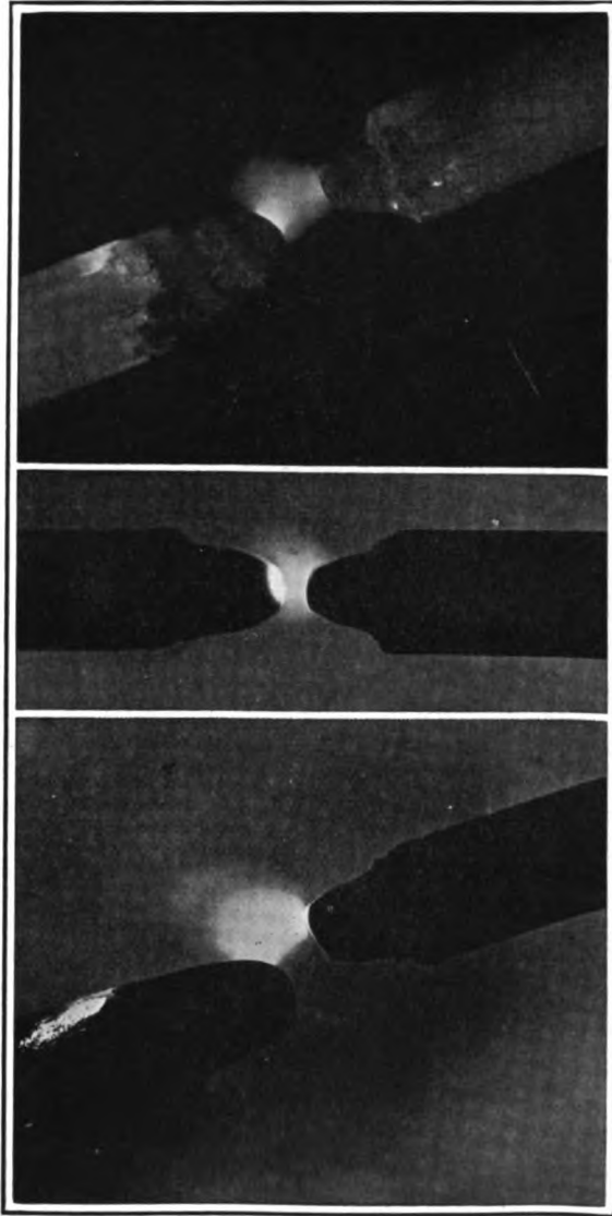
FIG. 298. FRONT AND SIDE VIEWS OF THE INCLINED CARBON ARC WITH 25 AMPERES OF ALTERNATING CURRENT.
