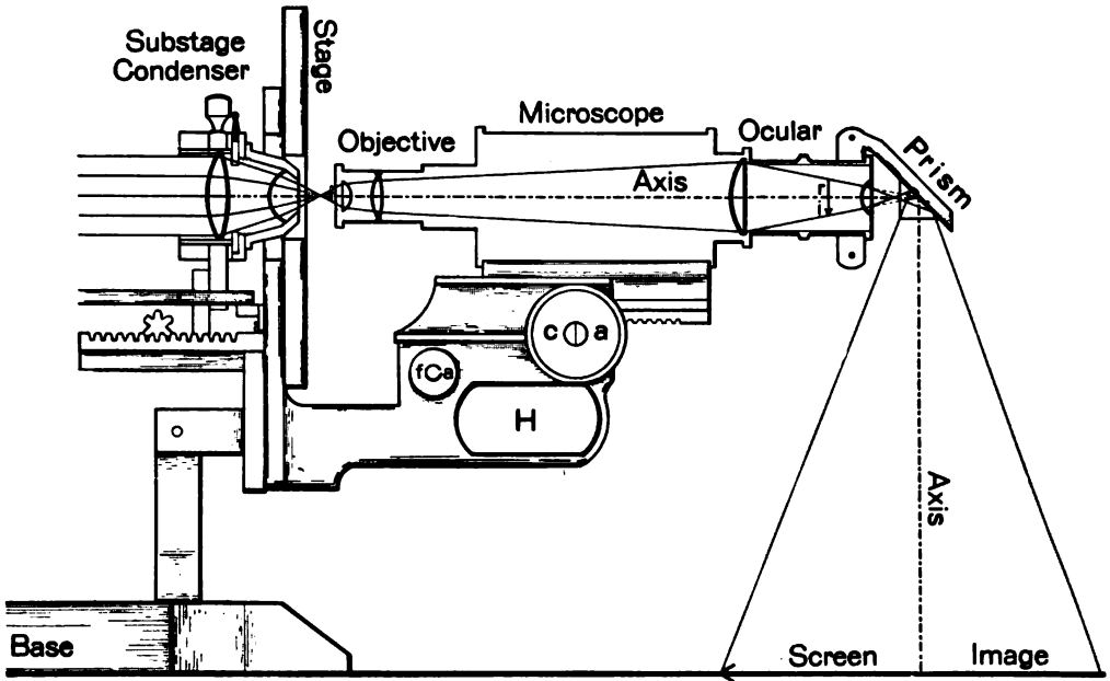
FIG. 192. DIAGRAM OF THE MICROSCOPE ARRANGED FOR DRAWING ON A HORIZONTAL SURFACE.
