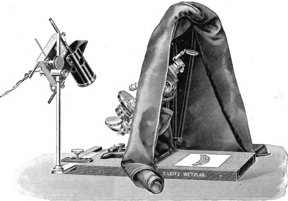
FIG. 204. EDINGER'S OUTFIT FOR DRAWING WITH AN ORDINARY MICROSCOPE AND SMALL ARC LAMP ON THE HOUSE LIGHTING SYSTEM.
