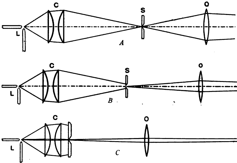
FIG. 364. ILLUMINATION OF THE SLIT FOR THE PROJECTION OF SPECTRA.
