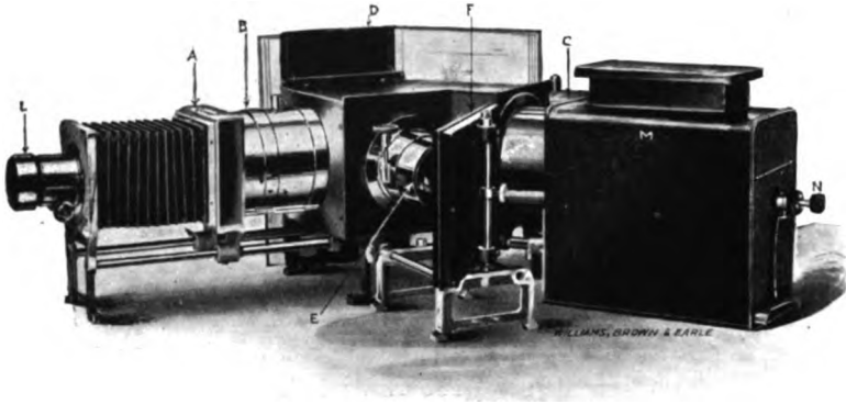
FIG. 98. THE NEW REFLECTING LANTERN OF WILLIAMS BROWN & EARLE (No. 3 BR 15).
