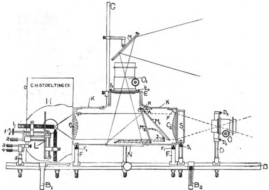
FIG. 167. UNIVERSAL PROJECTOSCOPE SHOWING THE ARRANGEMENT FOR HORIZONTAL TRANSPARENCIES AND FOR MICROSCOPIC PROJECTION.
