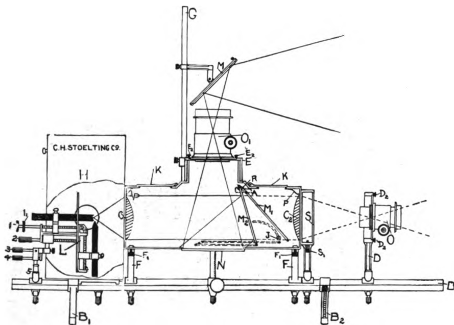
FIG. 103. DIAGRAM OF THE PARTS AND COURSE OF THE RAYS IN THE UNIVERSAL PROJECTOSCOPE FOR OPAQUE AND LANTERN-SLIDE PROJECTION.
