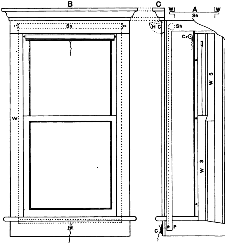
FIG. 238. FACE AND SECTIONAL VIEW OF WINDOW SHADES PLANNED FOR IN THE CONSTRUCTION OF THE BUILDING.
