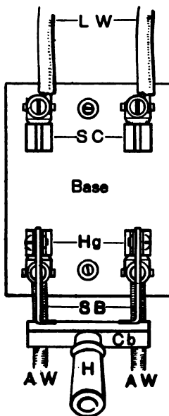
FIG. 277. OPEN KNIFE SWITCH IN A VERTICAL POSITION, WITH THE HANDLE BELOW SO THAT THERE IS NO DANGER OF THE SWITCH CLOSING BY GRAVITY.
