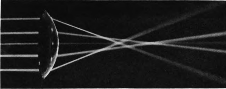
FIG. 320. CROSSING OF LIGHT RAYS WITH GREATEST ABERRATION, §809
