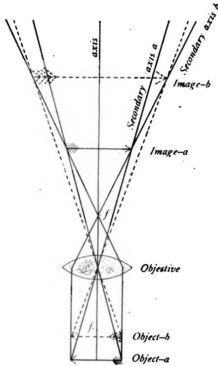
FIG. 210. DIAGRAM TO SHOW THAT THE SIZE OF THE IMAGE DEPENDS UPON THE DISTANCE OF THE OBJECT FROM THE CENTER OF THE LENS. (From The Microscope ).
