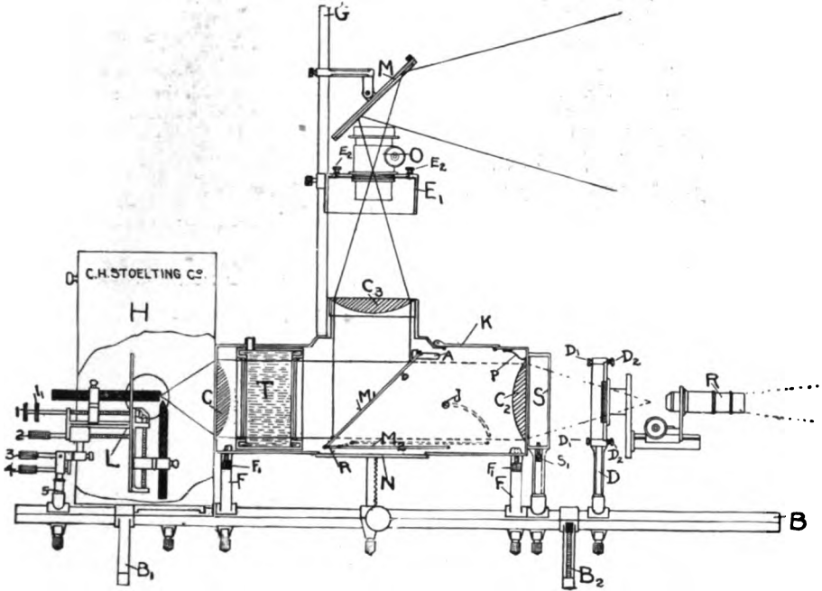
FIG. 16. ARRANGEMENT OF THE MAGIC LANTERN FOR HORIZONTAL OBJECTS.
