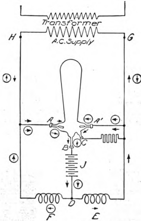
FIG. 261. MERCURY ARC RECTIFIER, DIAGRAM OF CONNECTIONS. (Cut loaned by the General Electric Co.).
