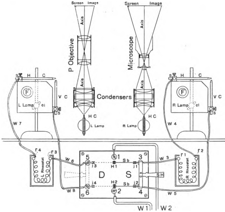
FIG. 162. COMBINED LANTERN-SLIDE AND MICRO-PROJECTION WITH TWO COMPLETE OUTFITS SIDE BY SIDE.
