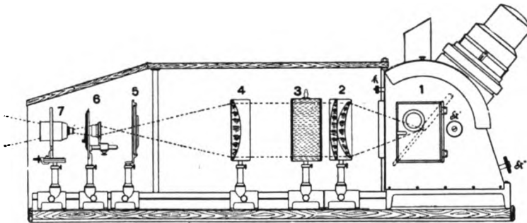
FIG. 156. PROJECTION MICROSCOPE OF ZEISS.
