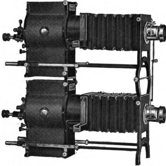
FIG. 17. MULTIPLE LANTERN FOR DISSOLVING VIEWS.
