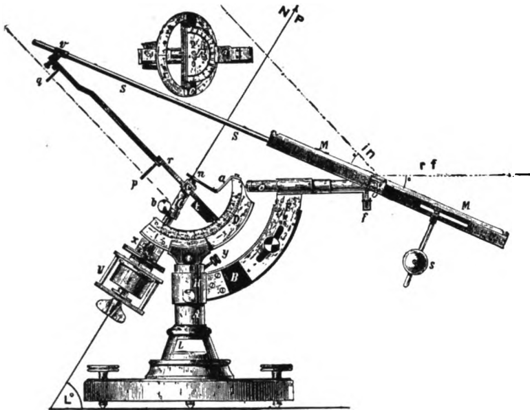
FIG. 79. UNIVERSAL, ONE-MIRROR HELIOSTAT.
