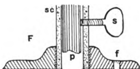
FIGURE 158F. SECTIONAL VIEW OF A RAILING FLANGE AND SOCKET.
