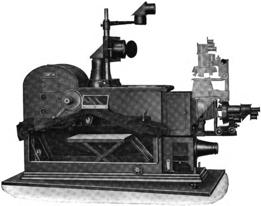
FIG. 176. MODEL 8 DELINEASCOPE SHOWING THE POSITION OF THE MICROSCOPIC ATTACHMENT FOR VERTICAL AND FOR HORIZONTAL OBJECTS.
