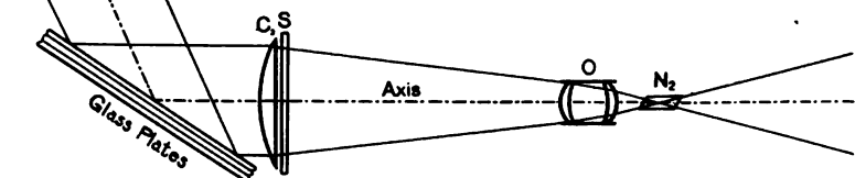
FIG. 351. LIGHT POLARIZED BY A PILE OF GLASS PLATES.
