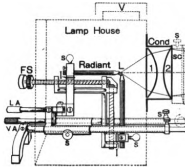
FIG. 331. TWO-LENS CONDENSER FOR PROJECTION.
