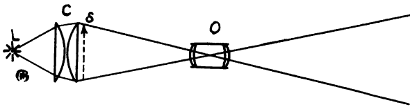
FIG. 325. LANTERN-SLIDE PROJECTION; NO SPHERICAL ABERRATION.
