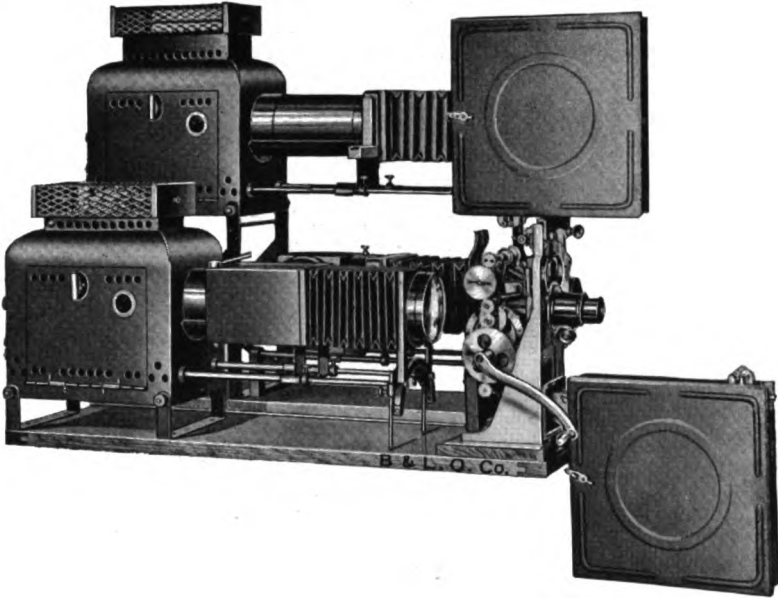
FIG. 224. DOUBLE DISSOLVING MODEL C BALOPTICON WITH EDISON MOVING PICTURE ATTACHMENT.
