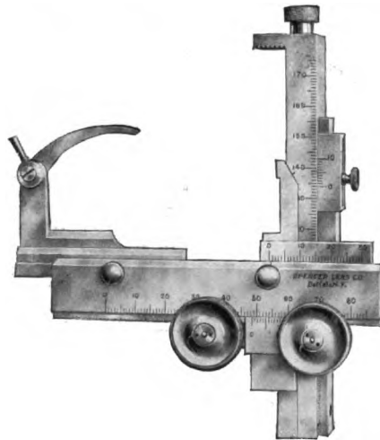
FIG. 135. MECHANICAL STAGE OF GREAT RANGE. (Cut loaned by the Spencer Lens Co.)
