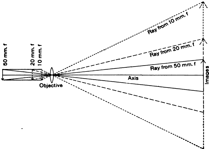
FIG. 144a. DIAGRAM TO SHOW THE POSITIONS OF THE SAME OBJECT AND THE SIZE OF THE SCREEN IMAGE FOR OBJECTIVES OF 50, 20 AND 10 MM. FOCUS.
