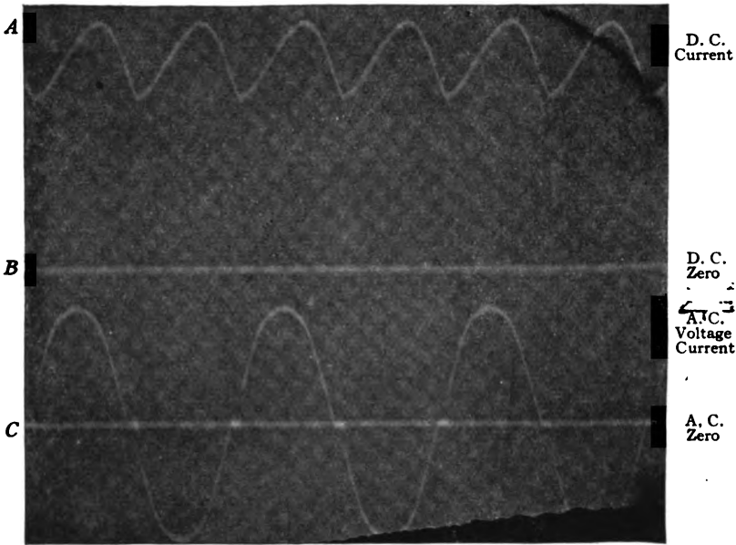
FIG. 262. OSCILLOGRAMS OF THE ALTERNATING CURRENT SUPPLY AND THE DIRECT CURRENT DELIVERED.
