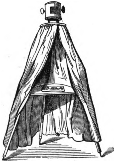
FIG. 88. CAMERA FOR DRAWING LANDSCAPES. (From the Catalogue of Queen & Co., 1880).
