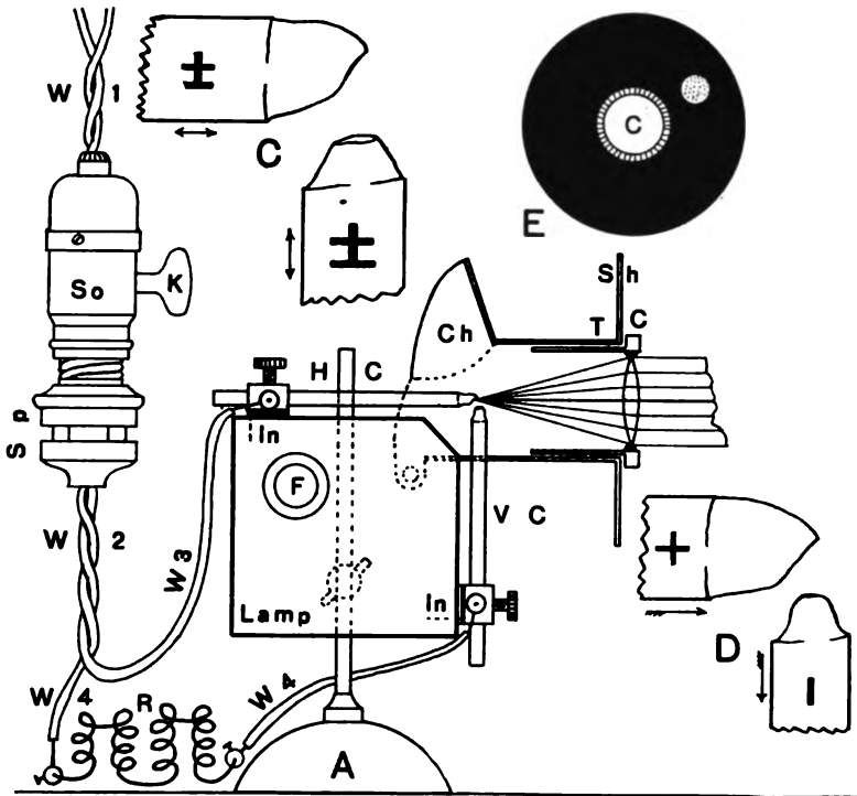
FIG. 189. SMALL ARC LAMP FOR DRAWING.
