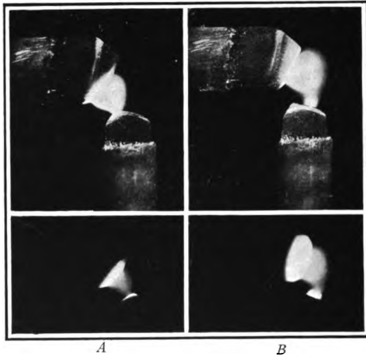
FIG. 293. SIDE VIEW OF THE RIGHT-ANGLE CARBON ARC WITH 10 and WITH 20 AMPERES OF DIRECT CURRENT
