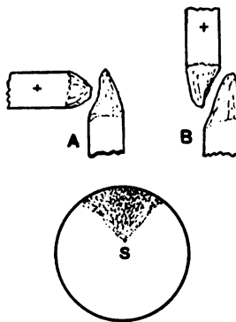
FIG. 25. CARBONS IN BAD RELATIVE POSITION, THE LOWER OR NEGATIVE CARBON EXTENDING UP IN FRONT OF THE POSITIVE CARBON.
