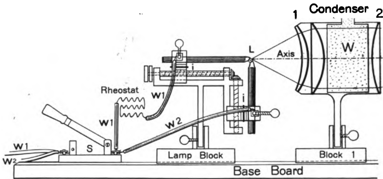
FIG. 332. THREE-LENS CONDENSER.
