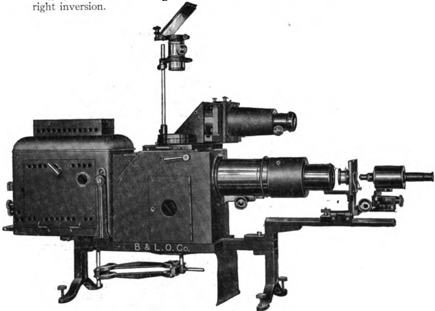
FIG. 172. UNIVERSAL BALOPTICON FOR OPAQUE OBJECTS, MICROSCOPIC OBJECTS AND FOR LANTERN SLIDES OR OTHER TRANSPARENT OBJECTS IN A VERTICAL OR A HORIZONTAL POSITION.
