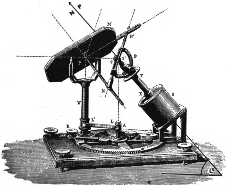
FIG. 78. ONE-MIRROR HELIOSTAT OF FOUCAULT. (From his Recueil des Travaux Scientifiques ).
