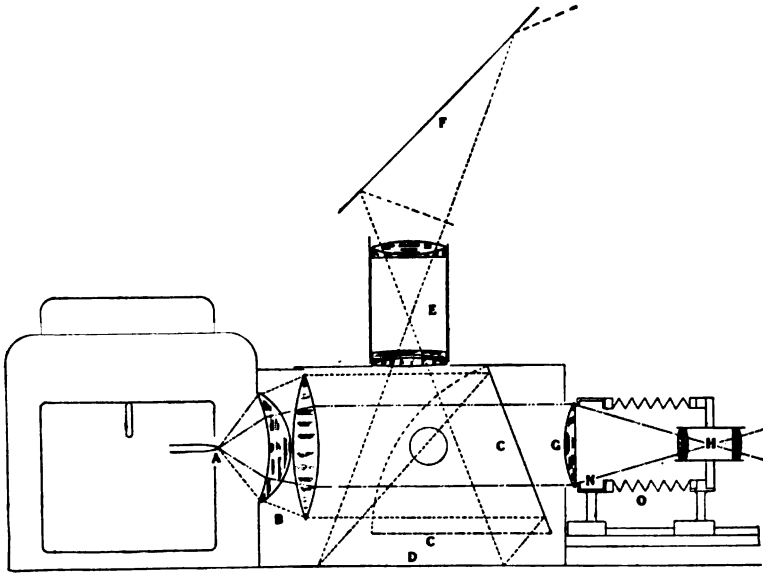
FIG. 105a. DIAGRAM SHOWING THE COURSE OF THE LIGHT RAYS FOR TRANSPARENCY AND OPAQUE PROJECTION WITH THE RADIANT HORIZONTAL. (Cut loaned by the Bausch & Lomb Optical Co.).
