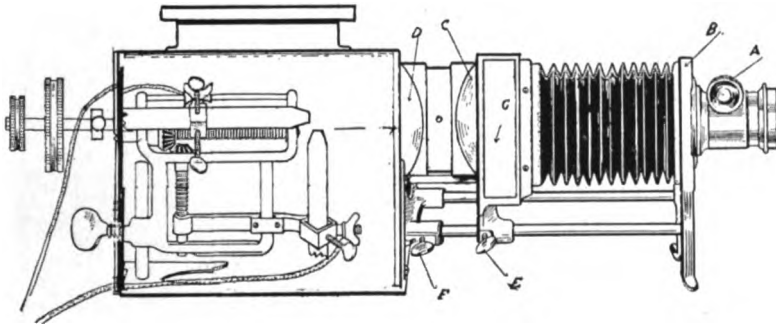
FIG. 32. MAGIC LANTERN IN OUTLINE TO SHOW THE PARTS. (Cut loaned by Williams, Brown & Earle).
