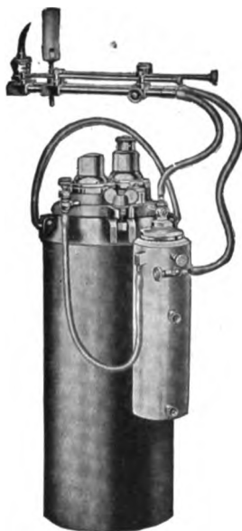
FIG. 63. PORTABLE OXYGEN GENERATOR AND ETHER SATURATOR.
