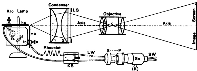
FIG. 185. SIMPLEST FORM OF MAGIC LANTERN WITH ARC LIGHT FOR USE IN DRAWING.
