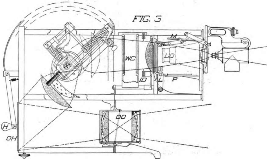
FIG. 199. MODEL 4-5 DELINEASCOPE WITH THE PROJECTION MICROSCOPE IN A HORIZONTAL POSITION.
