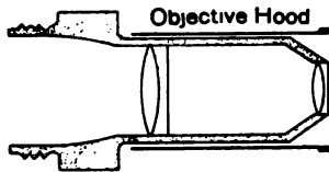
FIG. 139. PROJECTION OBJECTIVE WITH BLACK METAL HOOD.
