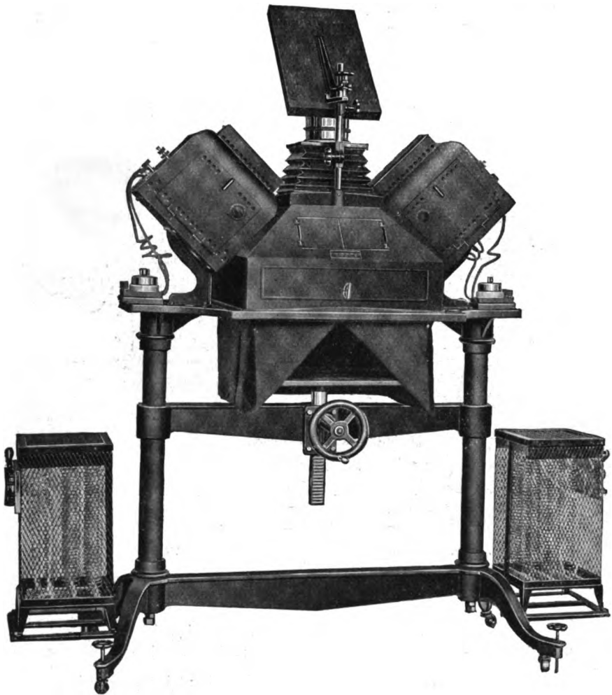
FIG. 107. BALOPTICON FOR THE PROJECTION OF LARGE OPAQUE OBJECTS. (Cut loaned by the Bausch & Lomb Optical Co.).
