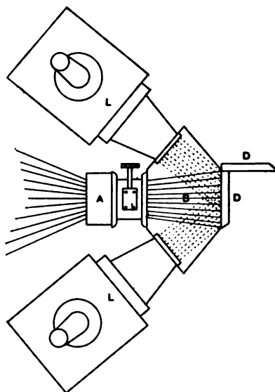
FIG. 93. CHADBURN'S OPAQUE LANTERN WITH TWO SOURCES OF LIGHT. (From Chadwick, Hepworth and Wright).
