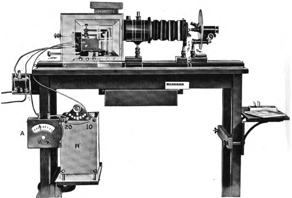
FIG. 133. PROJECTION MICROSCOPE WITH AMPLIFIER.
