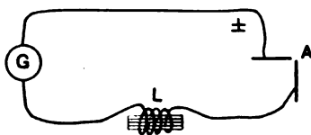
FIG. 289. INDUCTOR IN SERIES WITH AN ARC LAMP.
