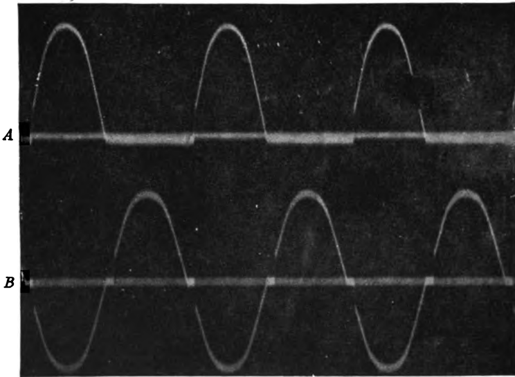
FIG. 263. OSCILLOGRAMS OF THE POTENTIAL DIFFERENCE BETWEEN THE ANODE AND CATHODE, IN RELATION TO THE IMPRESSED ELECTROMOTIVE FORCE.
