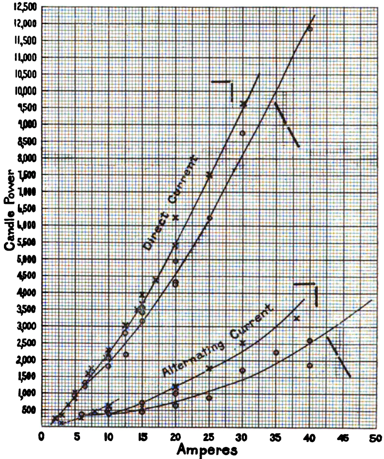
FIG. 302. VARIATION IN INTENSITY OF LIGHT FROM PROJECTION ARC LAMPS WITH DIRECT AND WITH ALTERNATING CURRENT.
