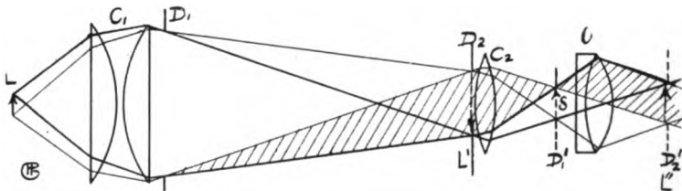
FIG. 349. KOEHLER'S METHOD OF ILLUMINATING MICROSCOPIC SPECIMENS.
