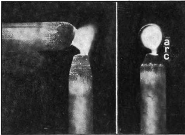
FIG. 295. LATERAL AND FACE VIEW OF THE RIGHT-ANGLE CARBON ARC WITH 20 AMPERES OF DIRECT CURRENT.
