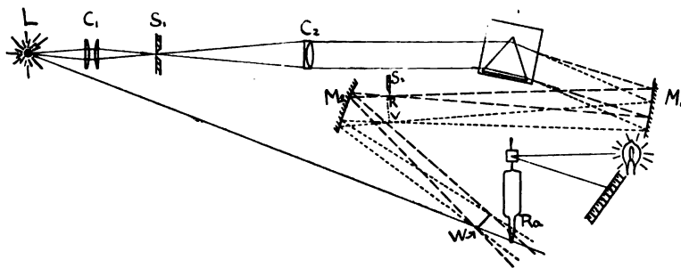
FIG. 308. ARRANGEMENT OF APPARATUS TO MEASURE L'/R .
