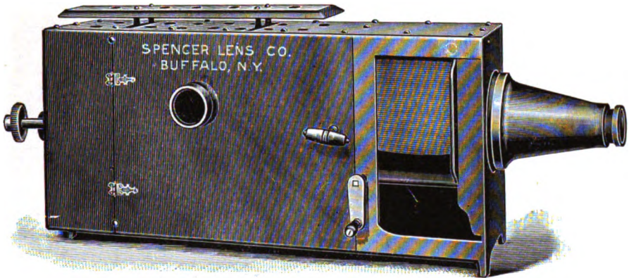
FIG. 38 A. SIMPLE MAGIC LANTERN WITH TWO-LENS CONDENSER AND A HAND-FEED ARC LAMP WITH RIGHT-ANGLED CARBONS AND WATER-CELL.
