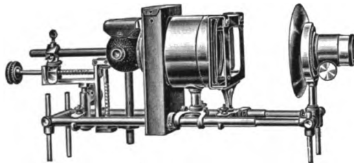
FIG. 37. MAGIC LANTERN WITH TWO-LENS CONDENSER, AND HAND-FEED ARC LAMP.
