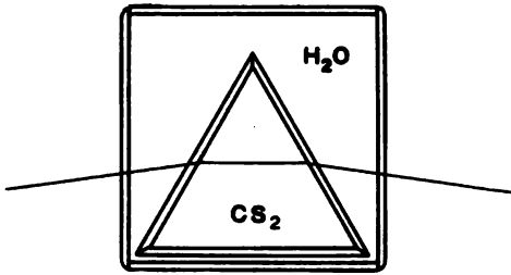
FIG. 358. LIQUID PRISM OF GOOD DISPERSION BUT SMALL DEVIATION.
