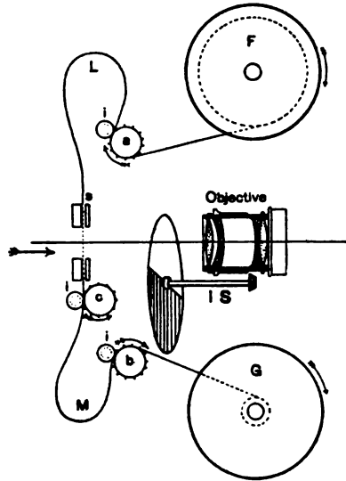
FIG. 225. MOVING PICTURE MECHANISM WITH INSIDE SHUTTER, I S. For full explanation see Fig. 231.
