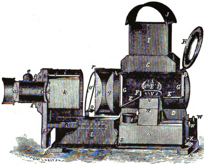
FIG. 65. MARCY'S MAGIC LANTERN OR "SCIOPTICON" WITH A MULTIPLE-WICK, PETROLEUM LAMP.
