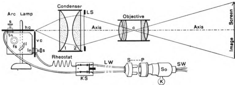
FIG. 46. THE MAGIC LANTERN FOR USE ON THE HOUSE LIGHTING SYSTEM.
