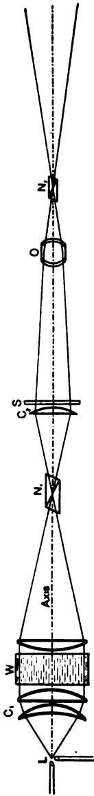
FIG. 350. PROJECTION WITH POLARIZED LIGHT, USING SMALL NICOL PRISMS.
