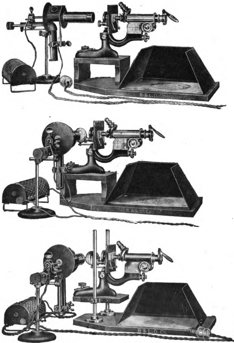
FIG. 201, A, B, C. SIMPLE DRAWING OUTFIT FOR THE MICROSCOPE. (Cuts loaned by the Bausch & Lomb Optical Co.).
