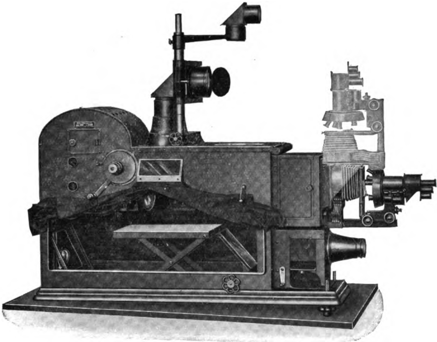
FIG. 110. MODEL 8 DELINEASCOPE FOR ALL KINDS OF PROJECTION. (Cut loaned by the Spencer Lens Co.).
