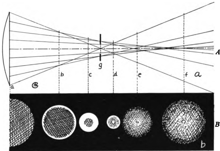
FIG. 326A. THE PATH OF THE LIGHT RAYS FROM THE DIFFERENT ZONES OF THE CONDENSER.
