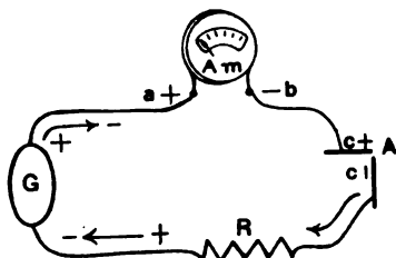
FIG. 273. AMMETER FOR TESTING POLARITY.
