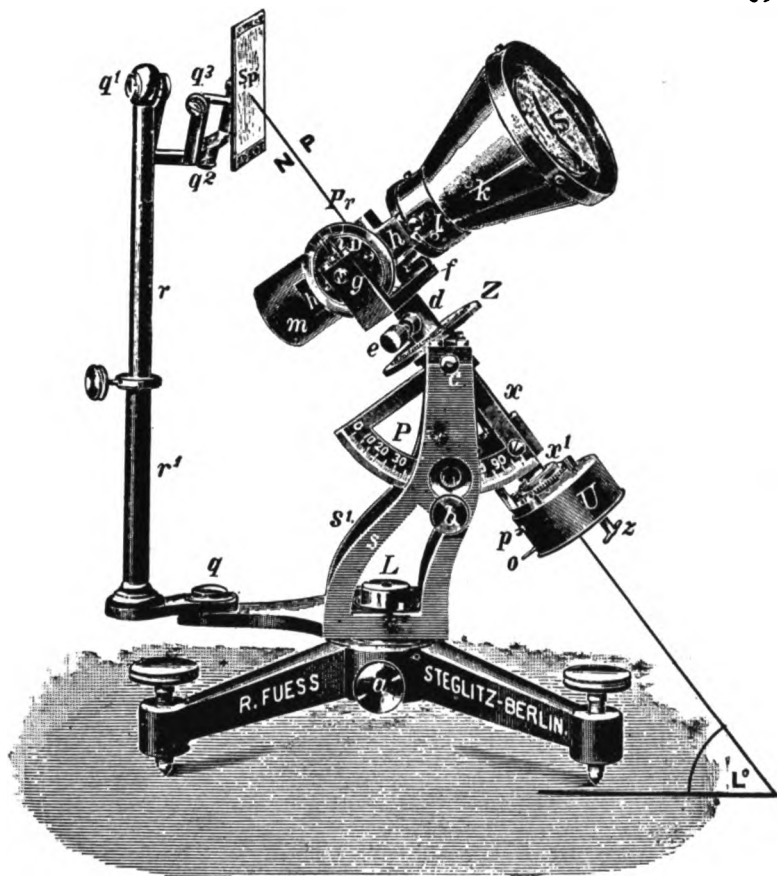
FIG. 84. LENS AND PRISM HELIOSTAT OF ALFRED M. MAYER. (From the Catalogue of Optical Instruments by R. Fuess).
