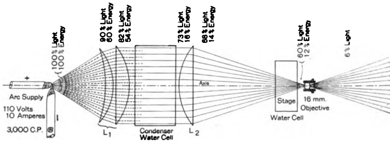
FIG. 342. ILLUSTRATION OF THE LIGHT AND ENERGY LOSSES IN THE PROJECTION MICROSCOPE.
