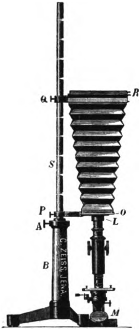
FIG. 217. VERTICAL PHOTO-MICROGRAPHIC CAMERA. (From Zeiss' Photo-micro-graphic Catalogue).
