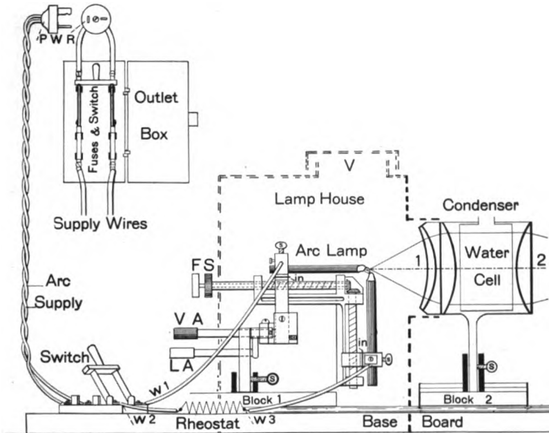
FIG. 3. ARC LAMP FOR PROJECTION, WITH WIRING, SWITCHES AND FUSES
