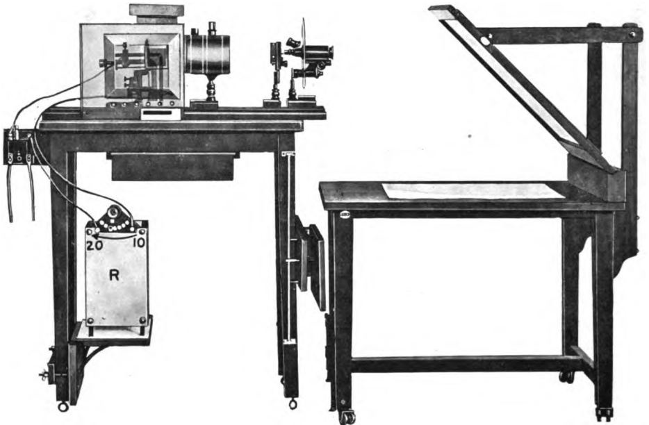
FIG. 182. DRAWING WITH PROJECTION APPARATUS AND A MOVABLE TABLE WITH 45° MIRROR.
