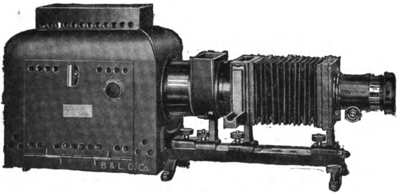
FIG. 34. MAGIC LANTERN OF THE LATHE-BED TYPE WITH A THREE-LENS CONDENSER AND WATER-CELL. ( Model D, Balopticon; Cut loaned by the Bausch & Lomb Optical Co. )
