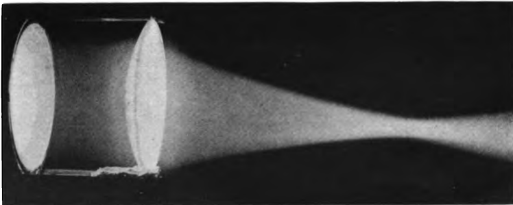
FIG. 323A. LIGHT CONE WITH THE RADIANT ABOVE THE OPTIC AXIS, §57
