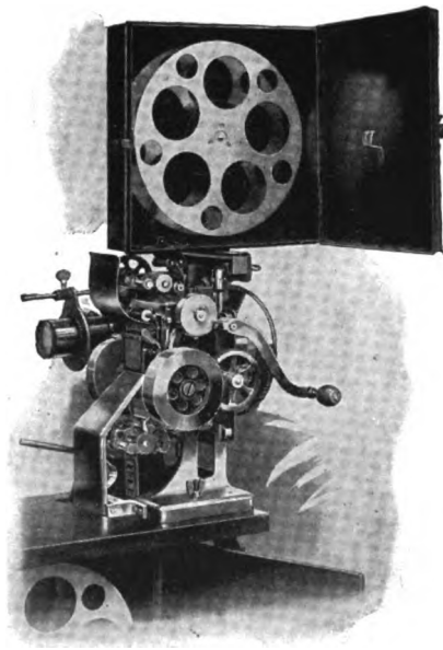
FIG. 233. EDISON KINETOSCOPE MECHANISM.
