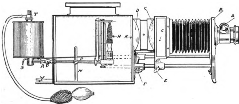
FIG. 72. MAGIC LANTERN WITH THE ALCO-RADIANT. (Cut loaned by Williams, Brown & Earle). For the details see fig. 32 and 73.
