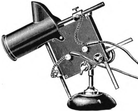
FIG. 41. THE LILIPUT ARC LAMP OF LEITZ.
