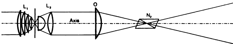
FIG. 352. CONVERGING POLARIZED LIGHT TO SHOW RINGS AND BRUSHES.
