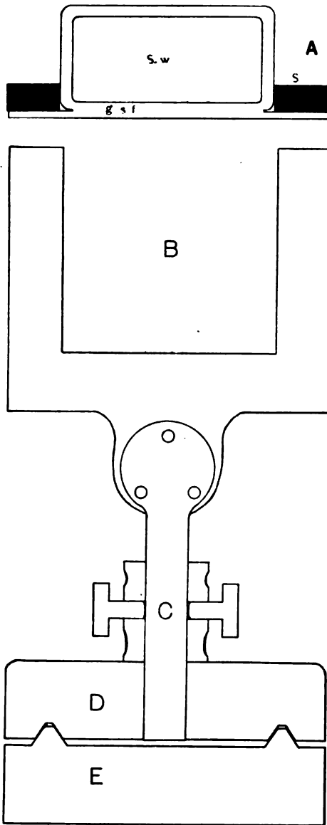
FIG. 134. FACE VIEW OF THE STAGE OF THE PROJECTION MICROSCOPE AND SECTIONAL VIEW OF THE STAGE WATER-CELL.
