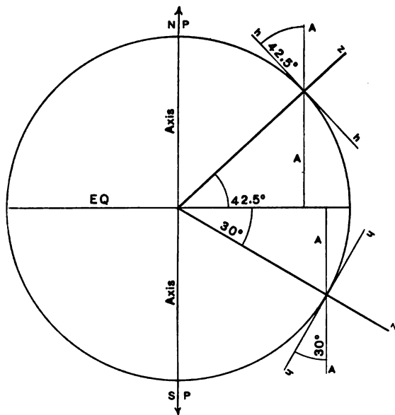
FIG. 85. DIAGRAM SHOWING THAT THE ELEVATION OF THE CLOCK-SHAFT AT AN ANGLE EQUAL TO THE LATITUDE OF A PLACE WILL MAKE THE CLOCK-SHAFT PARALLEL WITH THE EARTH'S AXIS.
