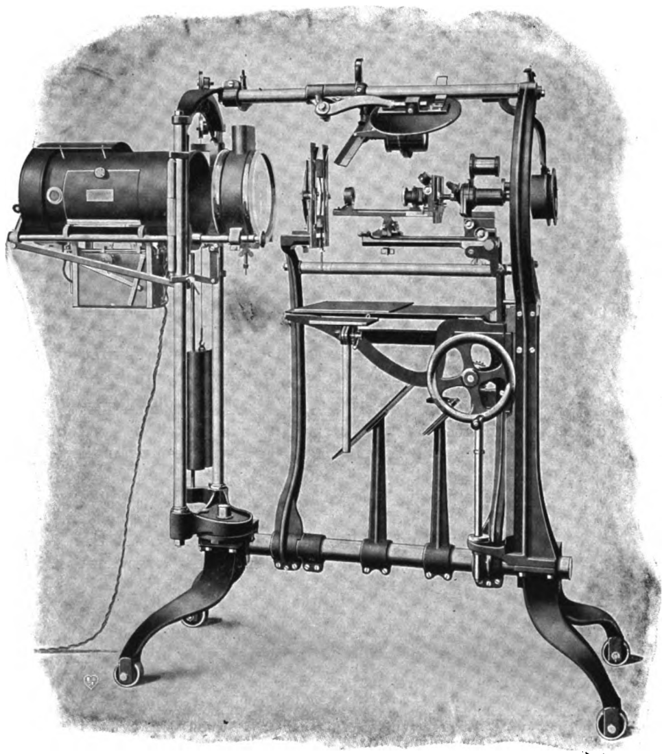
FIG. 96. UNIVERSAL PROJECTION APPARATUS WITH THE PROJECTION MICROSCOPE IN POSITION. (Cut loaned by E. Leitz).
