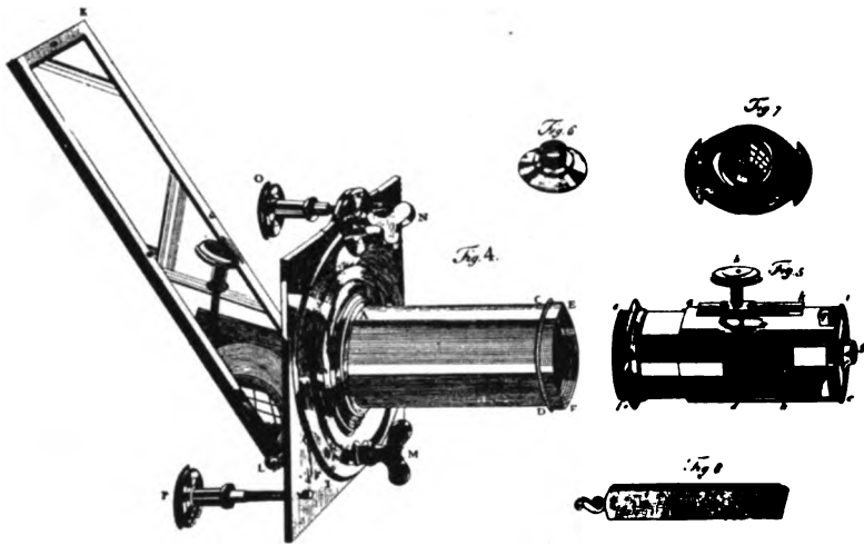
FIG. 75a. SOLAR, PROJECTION MICROSCOPE OF ADAMS, WITH PORTE-LUMIÈRE.
