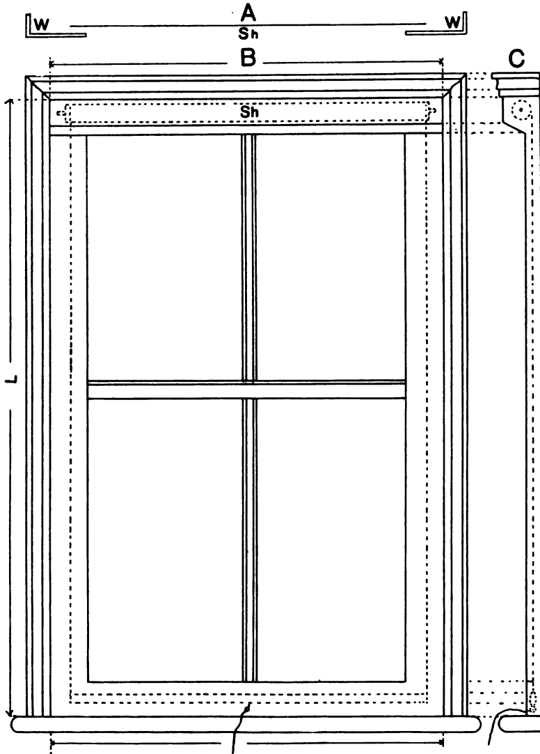
FIG. 239. FACE AND SECTIONAL VIEW OF A WINDOW SHOWING HOW THE LIGHT-EXCLUDING SHADE CAN BE INSTALLED AFTER THE BUILDING IS CONSTRUCTED.
