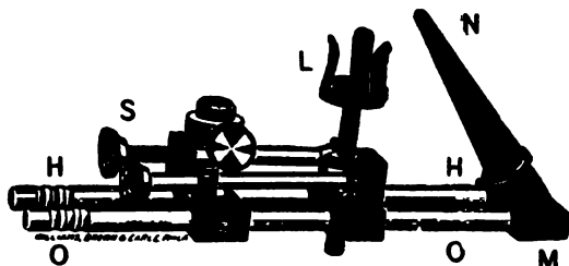
FIG. 59. MIXED BURNER OR JET FOR THE LIME LIGHT.
