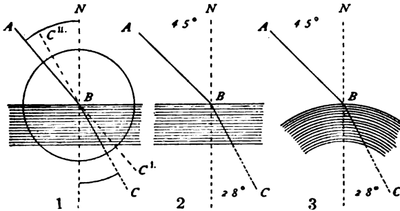
FIG. 312. REFRACTION AT PLANE AND AT CURVED SURFACES.
