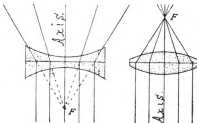
FIG. 319. THE PRINCIPAL FOCUS OF A CONVEX AND OF A CONCAVE LENS. (From The Microscope )
