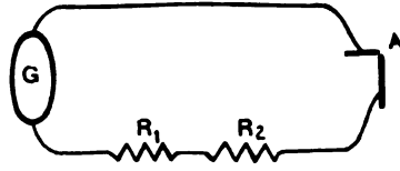
FIG. 287. RHEOSTATS IN SERIES.
