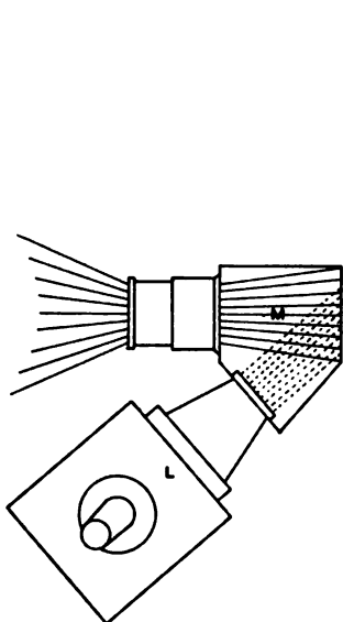
FIG. 92. CHADBURN'S OPAQUE LANTERN WITH ONE SOURCE OF LIGHT. (From Chadwick, Hepworth and Wright).
