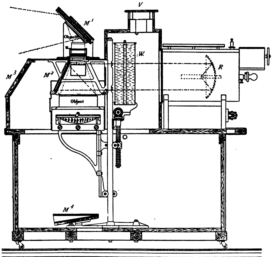
FIG. 95. ZEISS EPIDIASCOPE FOR OPAQUE AND FOR TRANSPARENT OBJECTS IN A HORIZONTAL POSITION. ( Zeiss' Special Catalogue ).
