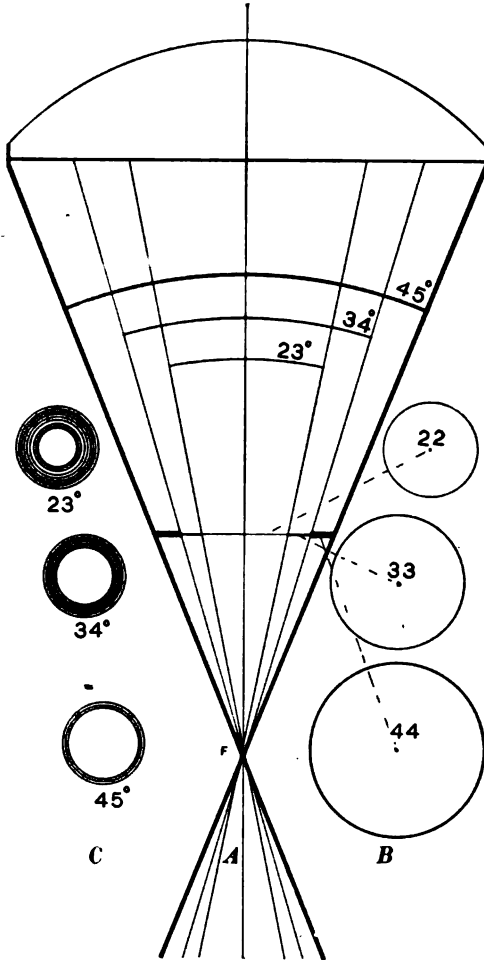
FIG. 155. THE EFFECT OF USING AN IRIS DIAPHRAGM IN THE CONE OF LIGHT FROM THE MAIN CONDENSER.
