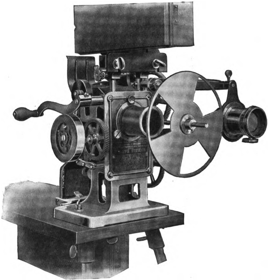
FIG. 227. MECHANISM OF POWER'S NO. 6 CAMERAGRAPH, SHOWING THE THREE-WING, OUTSIDE SHUTTER. (Cut loaned by the Nicholas Power Company).
