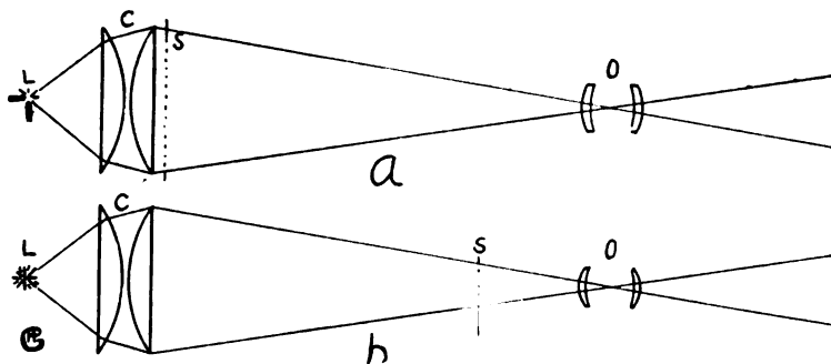
FIG. 328. INTERCHANGEABLE MAGIC LANTERN AND MOVING PICTURE PROJECTION WITH POINT SOURCE AND CONDENSER FREE FROM SPHERICAL ABERRATION.
