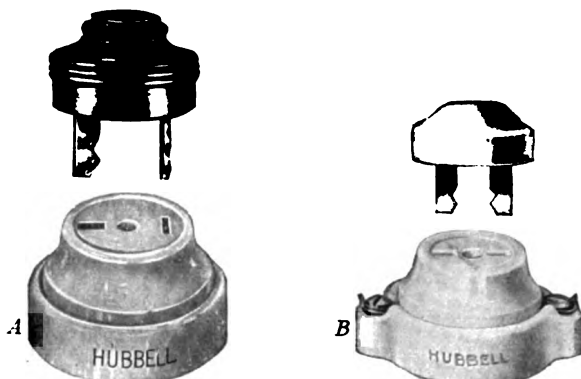
FIG. 268. SEPARABLE WALL RECEPTACLES, POLARIZED (A) AND NON-POLARIZED (B).
