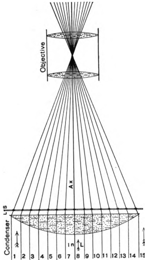
FIG. 91. TRANSPARENCY PROJECTION.
