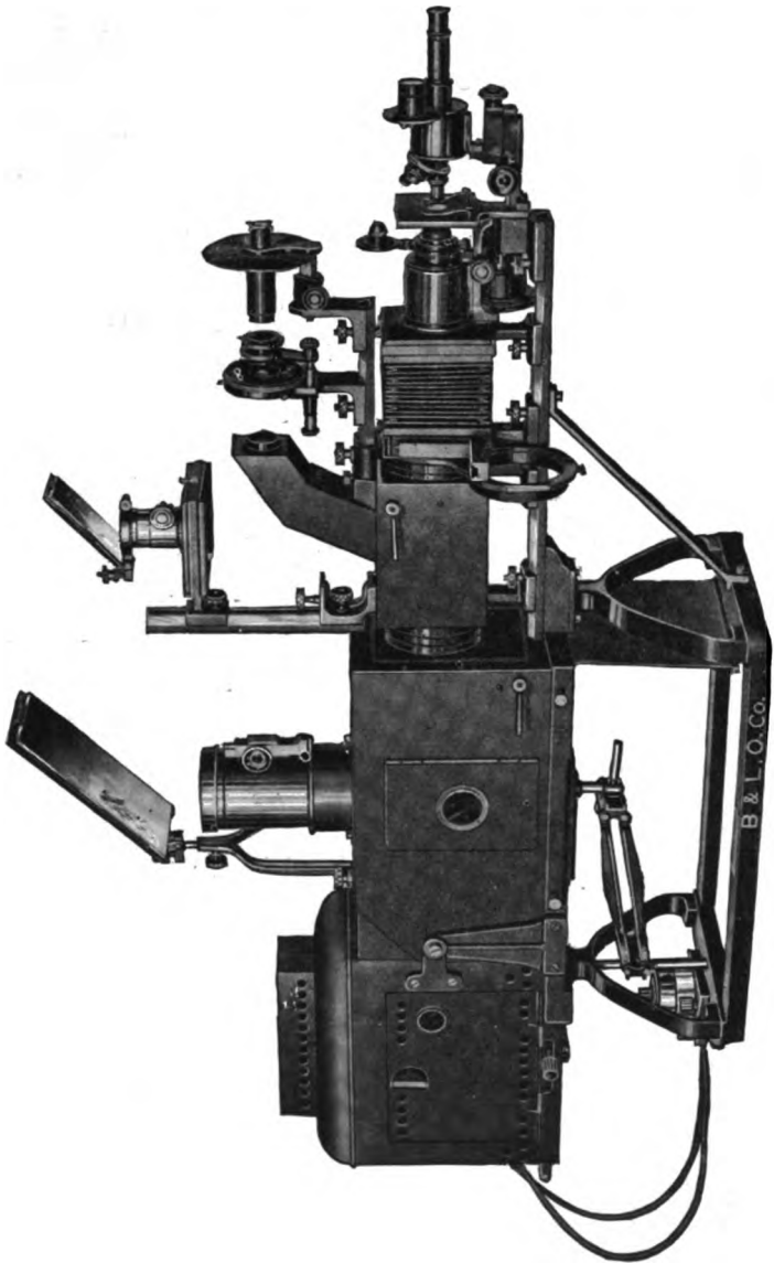
FIG. 169. NEW MODEL (1913) CONVERTIBLE BALOPTICON FOR ALL FORMS OF PROJECTION. (Cut loaned by the Bausch & Lomb Optical Co.).
