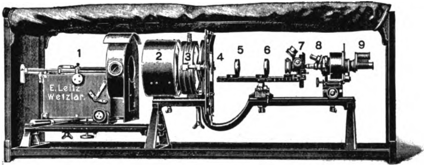
FIG. 163. LEITZ PROJECTION MICROSCOPE. (From Leitz Catalogue ).
