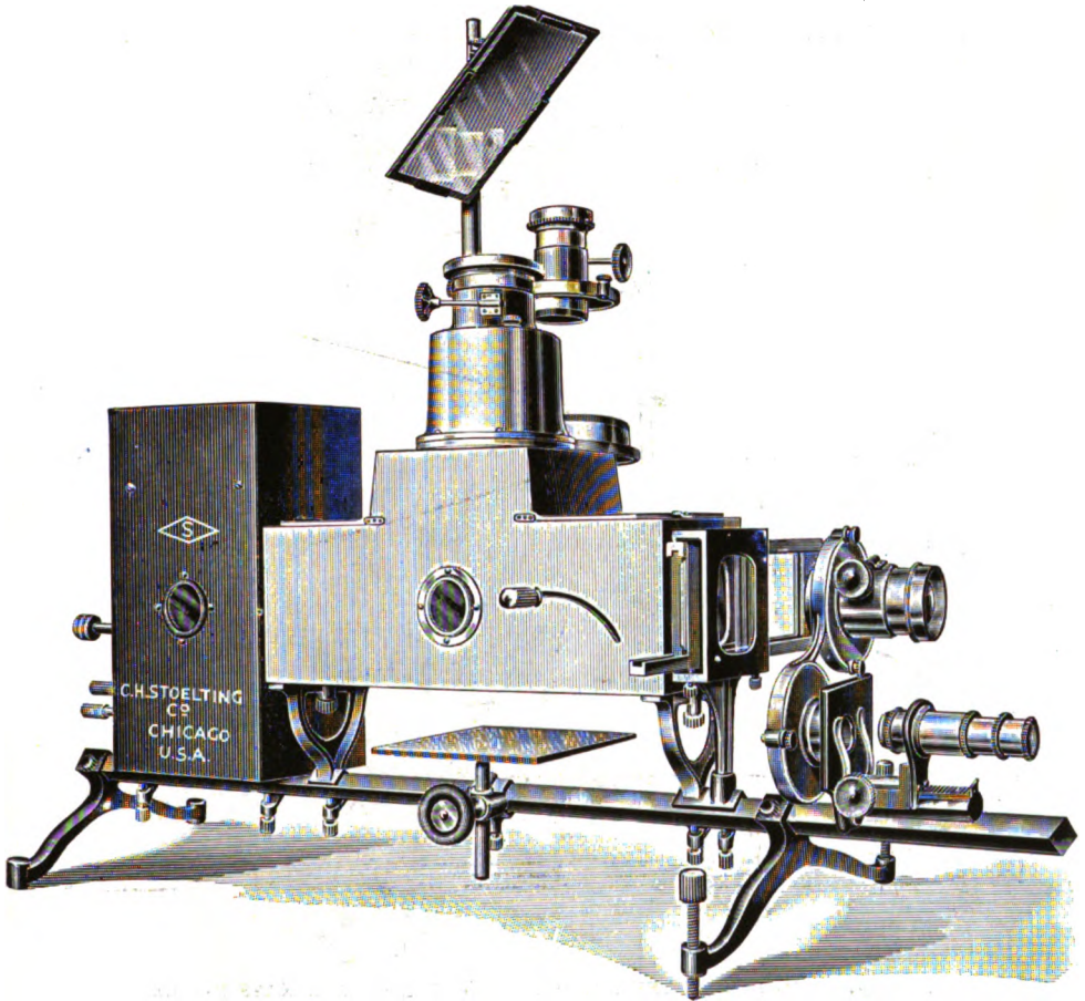
FIG. 102. UNIVERSAL PROJECTOSCOPE. (Cut loaned by C. H. Stoebling Company).
