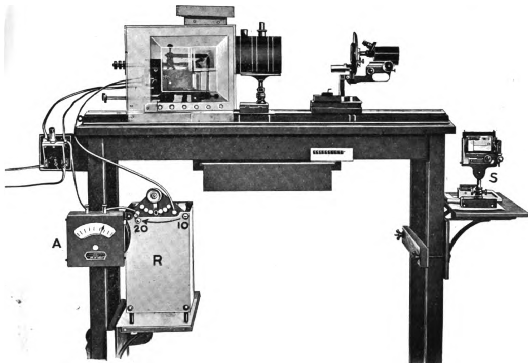
FIG. 145. ORDINARY MICROSCOPE FOR PROJECTION.
