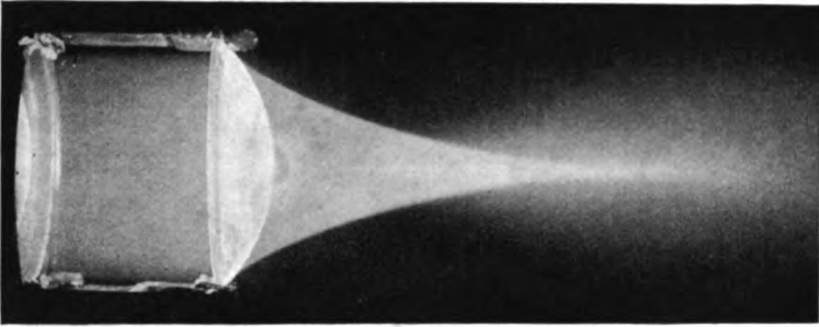
FIG. 322. PLANO-CONVEX LENS WITH GREATEST ABERRATION, §809
