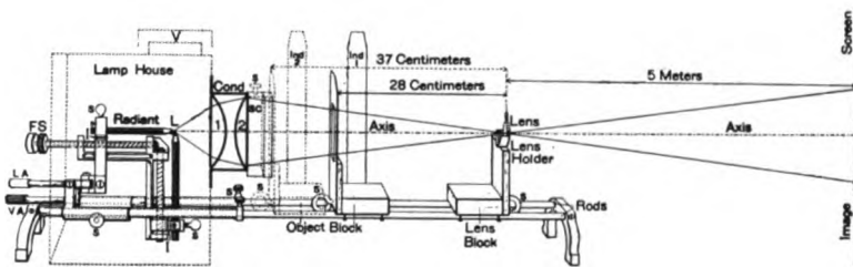
FIG. 379. PROJECTION APPARATUS WITH TWO-LENS CONDENSER FOR DEMONSTRATIONS REPRESENTING VISION.
