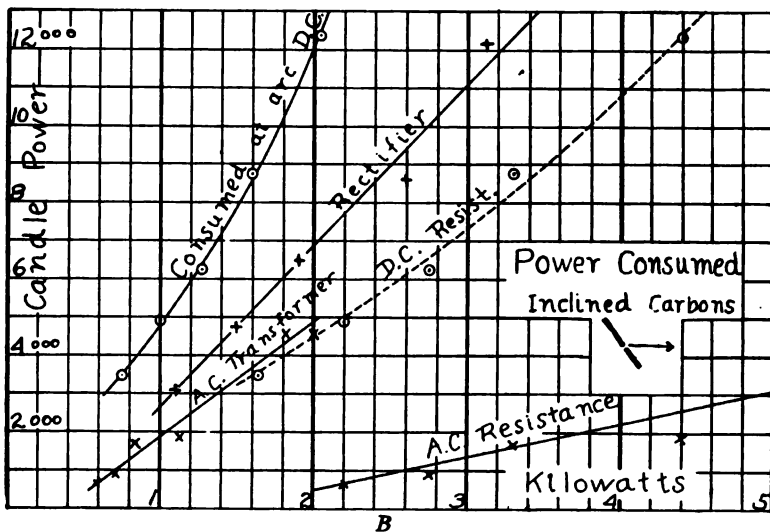
FIG. 304. RELATION BETWEEN POWER CONSUMPTION AND CANDLE-POWER.
