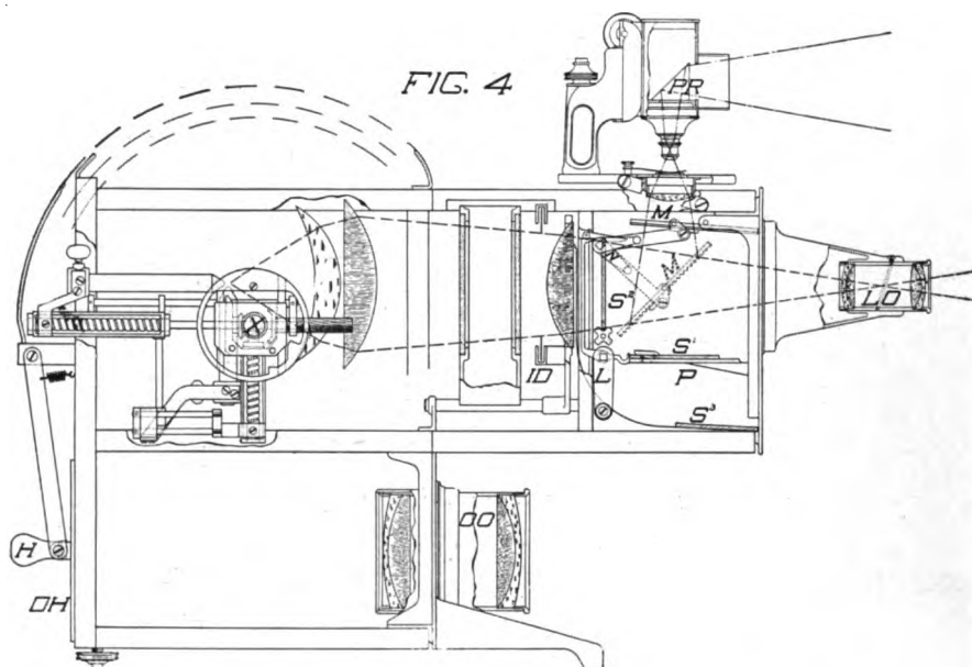
FIG. 175. MODEL 4-5 DELINEASCOPE WITH THE MICROSCOPE IN A VERTICAL POSITION FOR HORIZONTAL OBJECTS. (Cut loaned by the Spencer Lens Co.).
