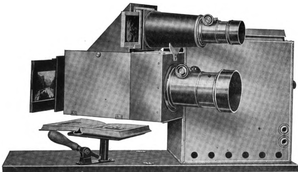
FIG. 97. THOMPSON'S REFLECTOSCOPE, MODEL G-2, 1913. (Cut loaned by A. T. Thompson & Co.).
