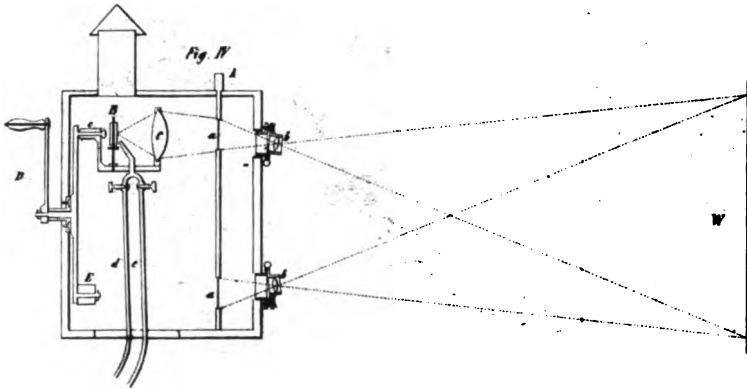
FIG. 410. THE MOVING PICTURE PROJECTOR OF UCHATIUS.
