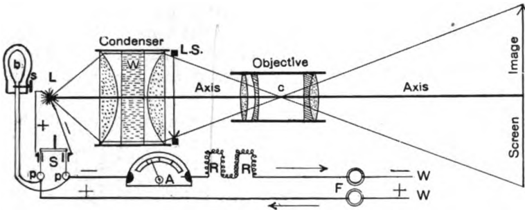
FIG. 4. MAGIC LANTERN WITH INCANDESCENT LAMP IN THE CIRCUIT AFTER THE RHEOSTAT (Compare fig. 2).
