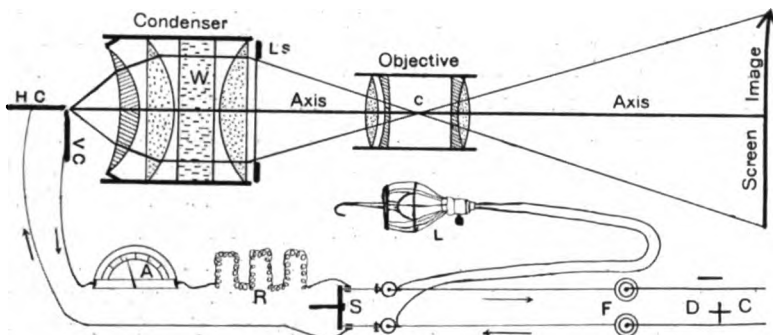
FIG. 2. MAGIC LANTERN WITH TRIPLE CONDENSER AND WATER-CELL.
