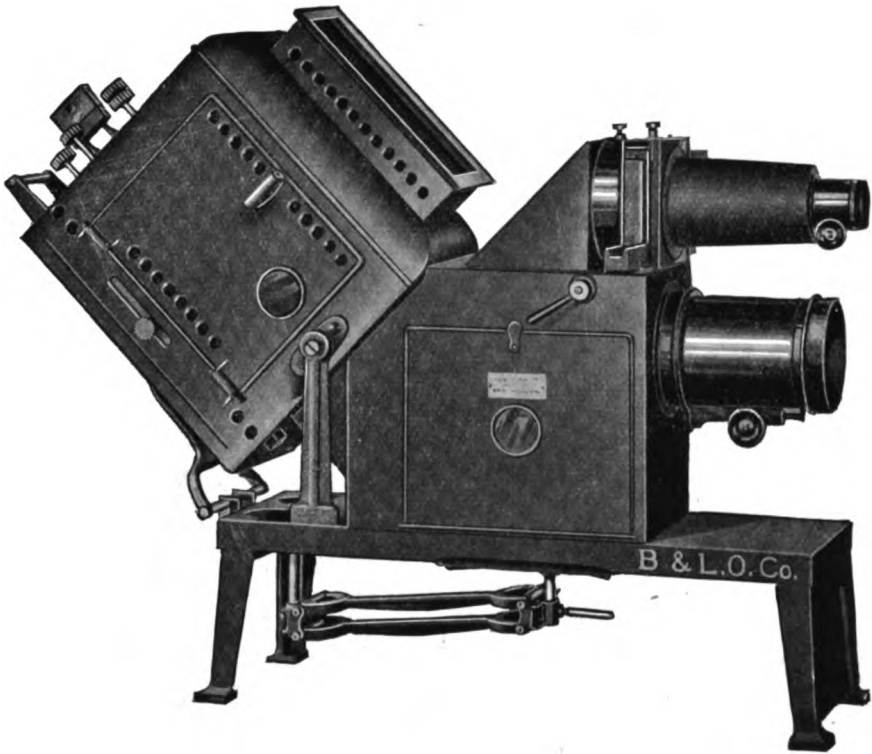
FIG. 106. NEW MODEL UNIVERSAL BALOPTICON IN POSITION FOR OPAQUE PROJECTION. (Cut loaned by the Bausch & Lomb Optical Co.).
