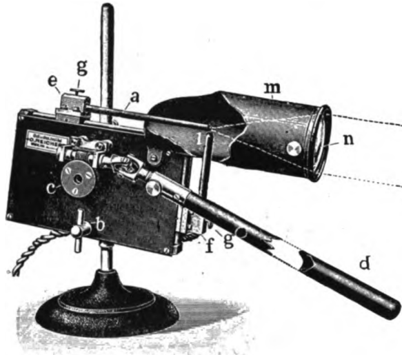
FIG. 43. THE SMALL ARC LAMP OF REICHERT.
