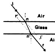
FIG. 313. REFRACTION BY GLASS WITH PARALLEL FACES.
