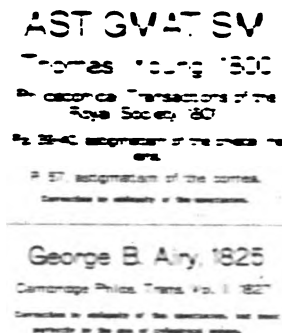
FIG. 394, 395. FIGURES SHOWING THE APPEARANCE OF THE RADIAL LINES AND OF PRINTED MATTER WHEN AN ASTIGMATIC LENS IS IN FOCUS FOR HORIZONTAL LINES.
