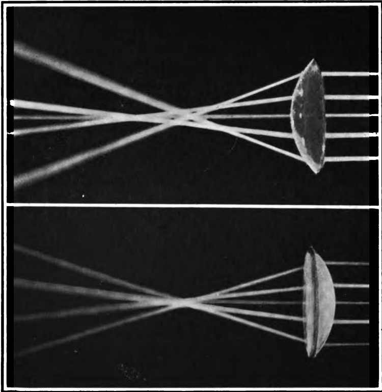
FIGS. 320-321. BEAMS OF PARALLEL LIGHT TRAVERSING PLANO-CONVEX LENSES TO SHOW MAXIMUM AND MINIMUM SPHERICAL ABERRATION.
