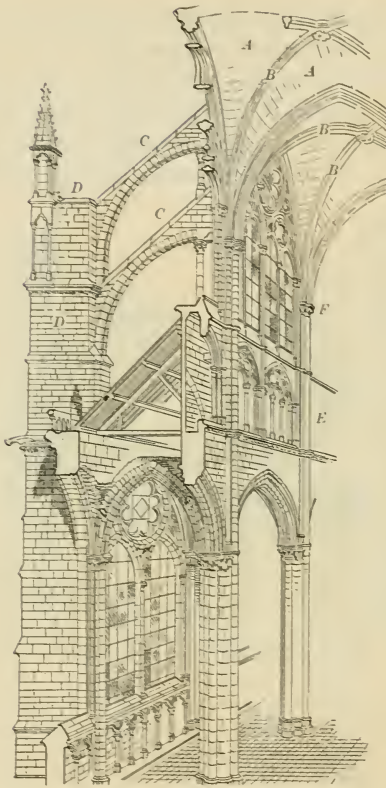
FIG. 183. CROSS SECTION OF AMIENS CATHEDRAL
