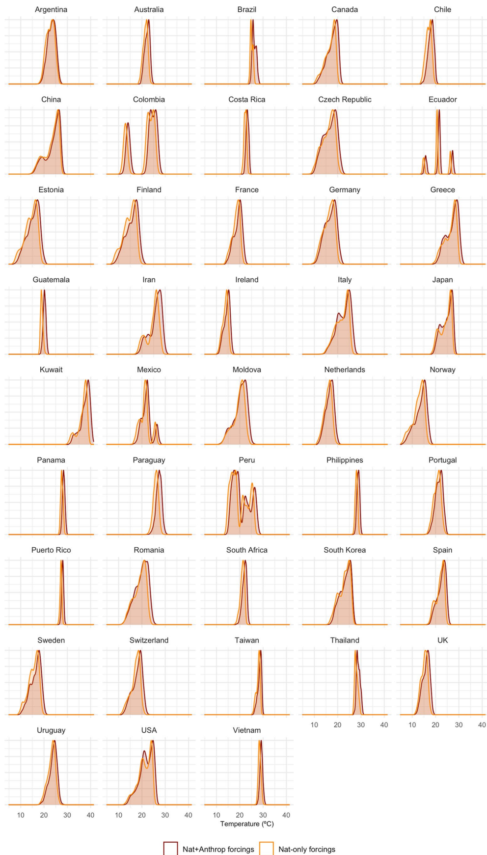
Extended Data Fig. 3 | Country-averaged warm-season temperature distributions modeled in each scenario. As Fig.1, factual scenario (with natural and anthropogenic forcings) is depicted in brown, while counterfactual scenario (with natural forcings only) in orange.
